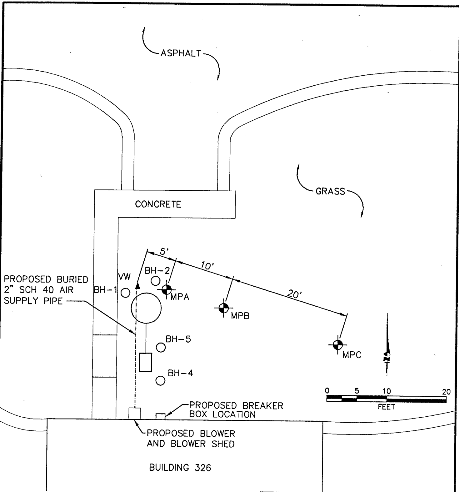
FIGURE 3.2 PROPOSED VENT WELL, MONITORING POINT, AND BLOWER LOCATIONS SWMU #70
