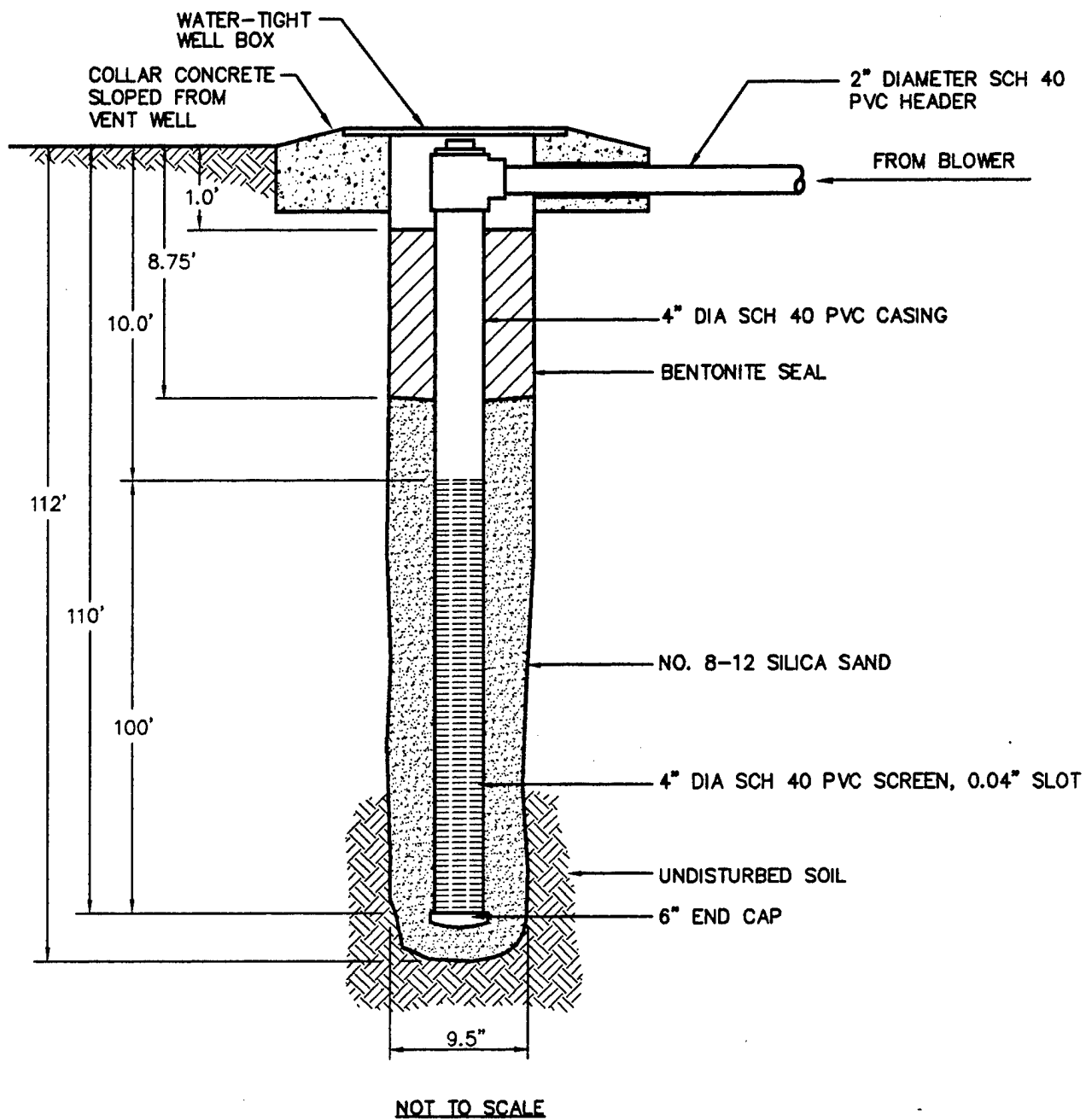
FIGURE 1.2 AS-BUILT INJECTION VENT WELL CONSTRUCTION DETAIL SWMU #70 CANNON AFB, NEW MEXICO ENGINEERING-SCIENCE, INC. Denver, Colorado
