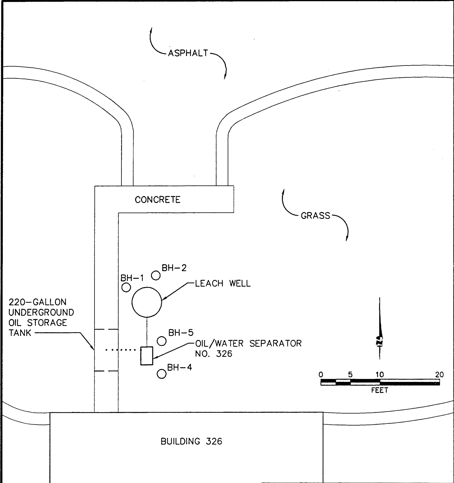
FIGURE 3.1 SITE LAYOUT SWMU #70 CANNON AFB, NEW MEXICO ENGINEERING-SCIENCE, INC. Denver, Colorado
