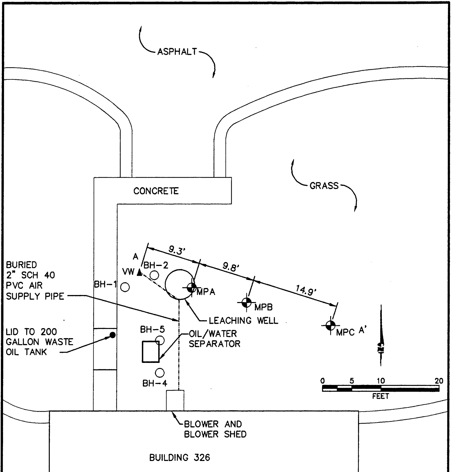
FIGURE 1.1 AS-BUILT VENT WELL, MONITORING POINT, AND BLOWER LOCATIONS SWMU #70 CANNON AFB, NEW MEXICO ENGINEERING-SCIENCE, INC. Denver, Colorado
