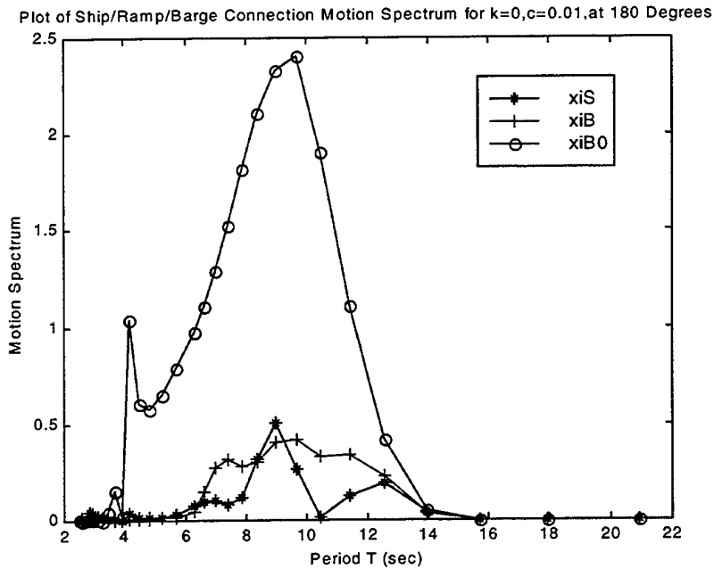
Figure 141. Plot of Vertical Motion Spectrum at the Ship/Ramp/Barge Connections, for k=0 and c=0.01 , at a Wave Angle of 180 Degrees.
