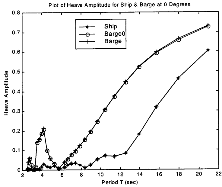
Figure 1. Plot of Heave Amplitude for the Ship, Barge without Ship/Ramp Influence and Barge without Ramp Influence at 0 Degrees Wave Angle.
