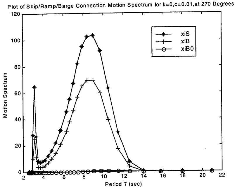
Figure 149. Plot of Vertical Motion Spectrum at the Ship/Ramp/Barge Connections, for k=0 and c=0.01 , at a Wave Angle of 270 Degrees.
