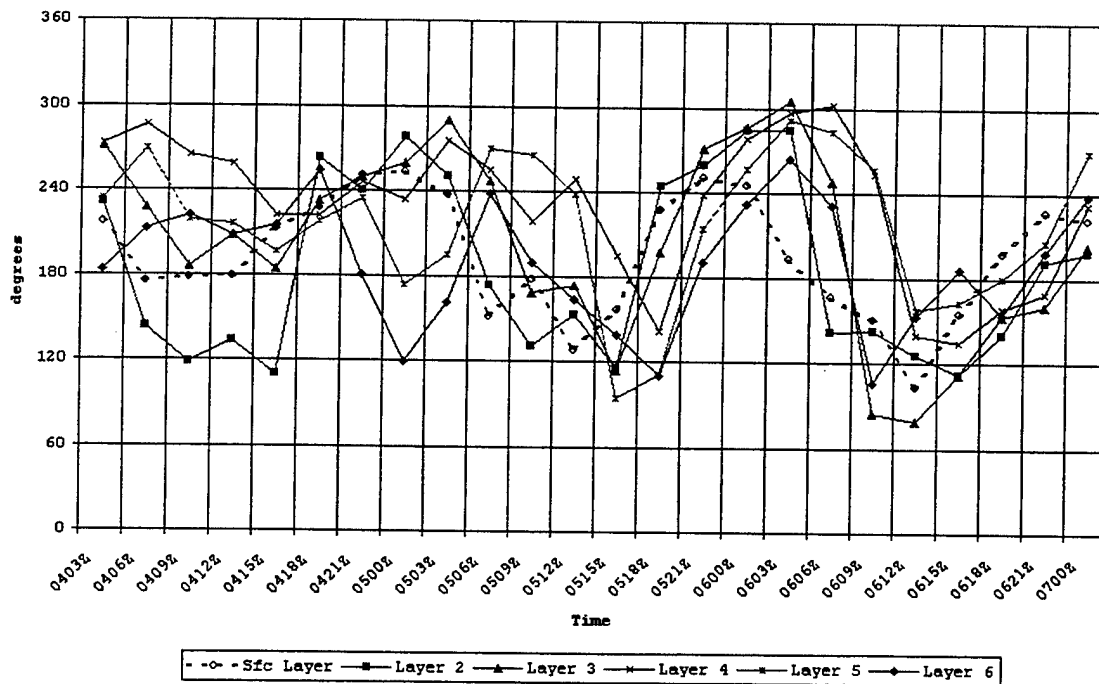
Figure 5-31. Mean wind direction, observations.
