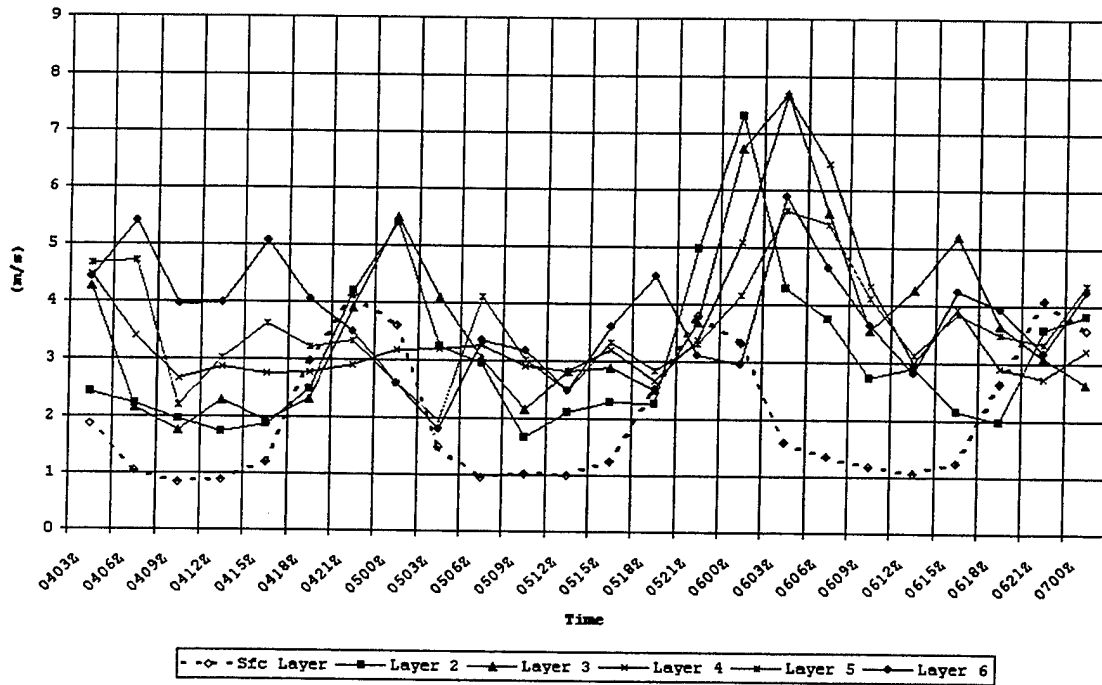
Figure 5-30. Mean wind speed, observations.
