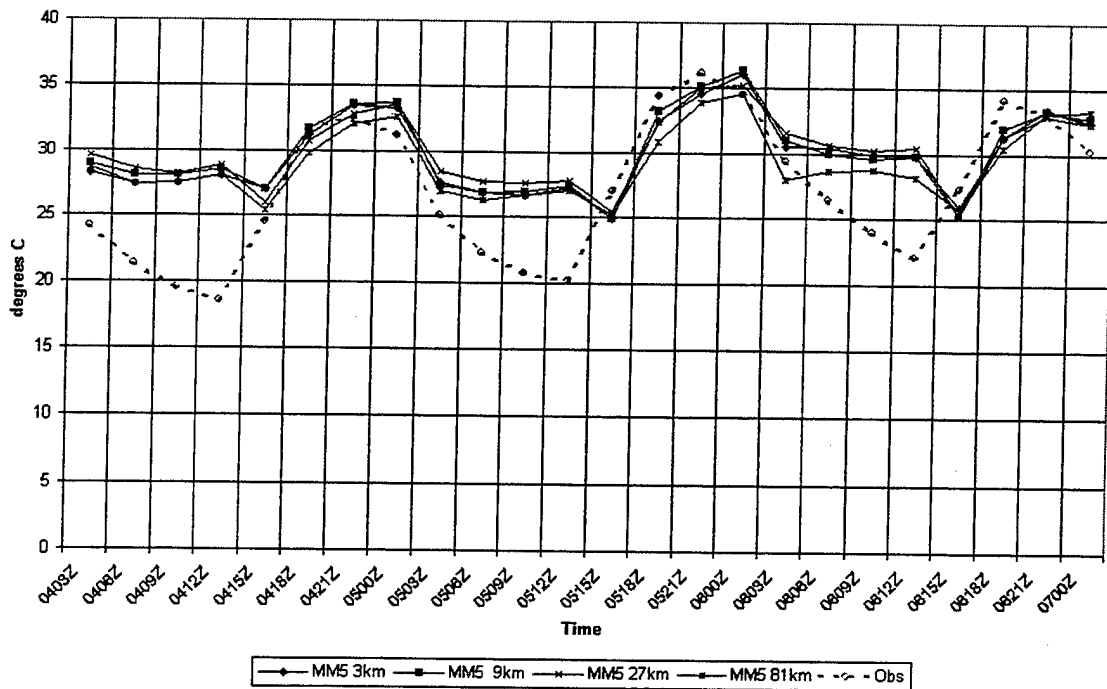
Figure 6-9. TEST1 mean temperature.
