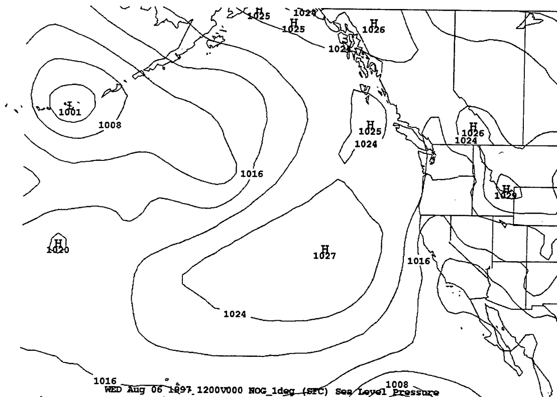
WED Aug 06 1997 0000V000 NOG_1deg (SFC) Sea Level Pressure Figure 5-24. 06/00Z NOGAPS surface mean sea level pressure.
