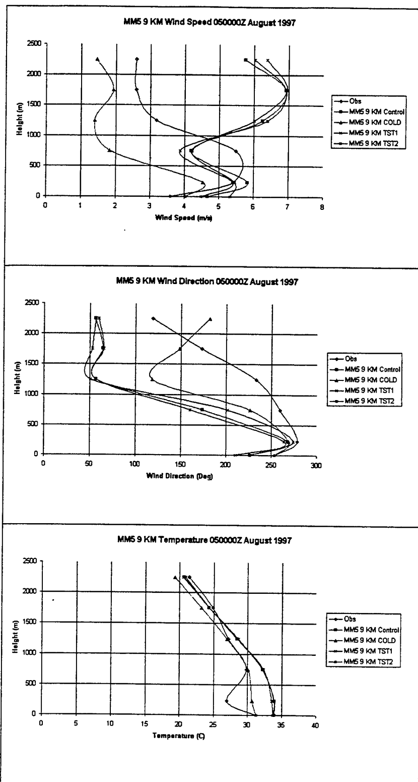
Figure 6-14. 05/00Z 9km mean vertical profiles.
