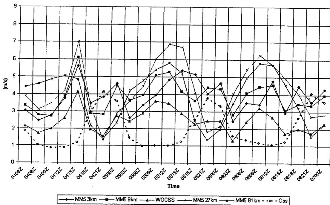
Figure 6-10. TEST2 mean wind speed.
