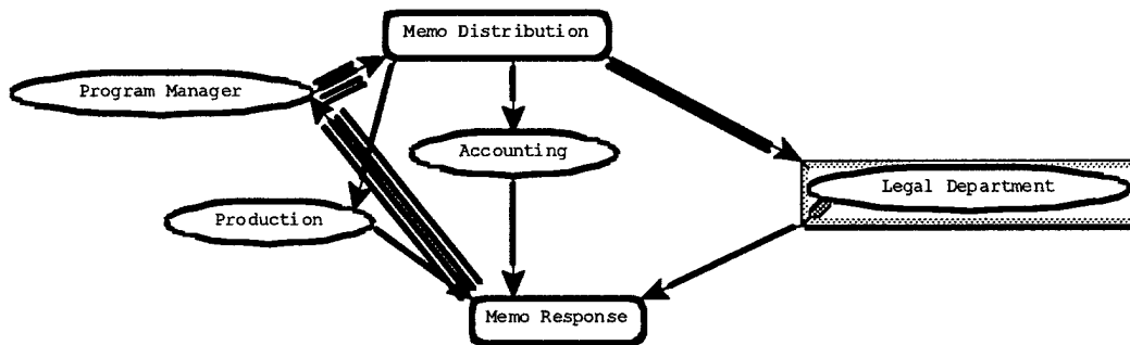
Figure: 3 Contracted Version of the Function of Figure 2. The Place "Legal Department" has been contracted; however, one arc is drawn from the place to the Transition "Memo Response" and it is colored orange. In the expanded version of this Function, two arcs are drawn to this transition.
