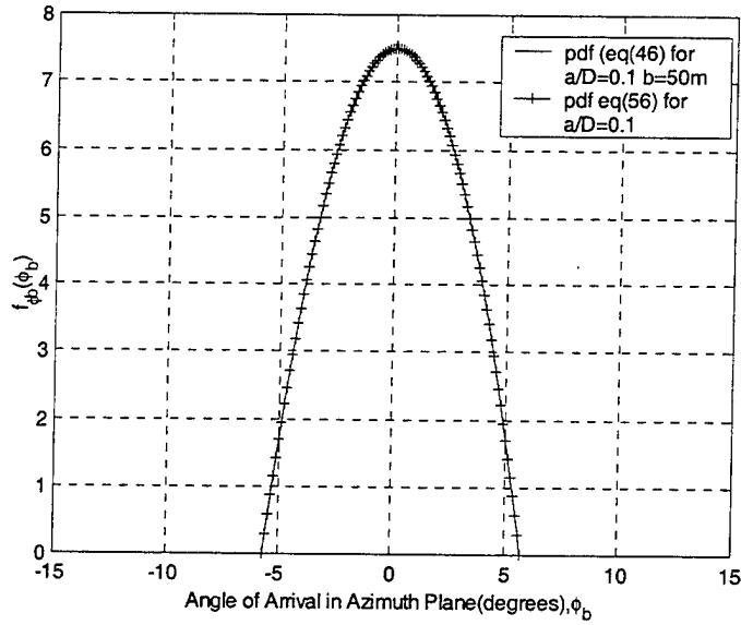
Figure 11. Plot of f_{\phi_b}(\phi_b) versus \phi_b for D=1000\text{m} , a=100\text{m} and b=50\text{m} (using the two different formulas).
