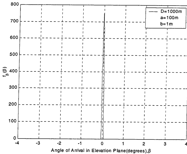
Figure 14. Plot of f_{\beta}(\beta) versus \beta for D=1000\text{m} , a=100\text{m} and b=1\text{m} .
