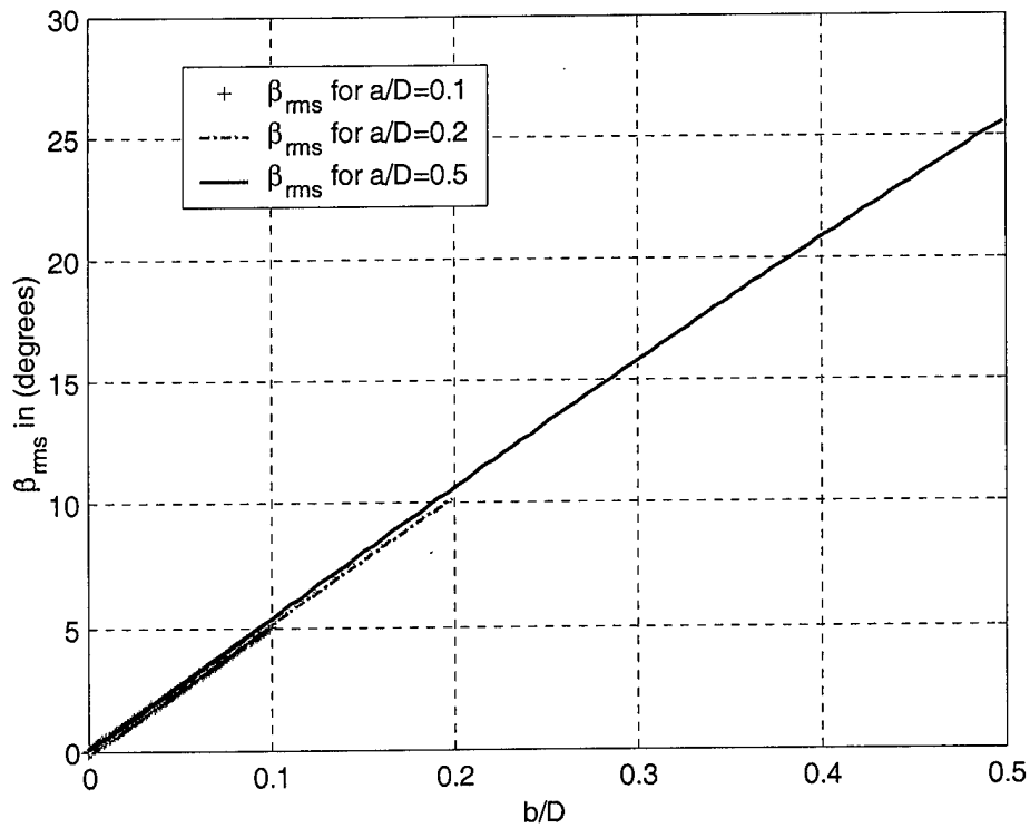
Figure 19. Plot of the r.m.s angular \beta_{rms} spread versus b/D for various ratios a/D , for the spheroid scattering model.
