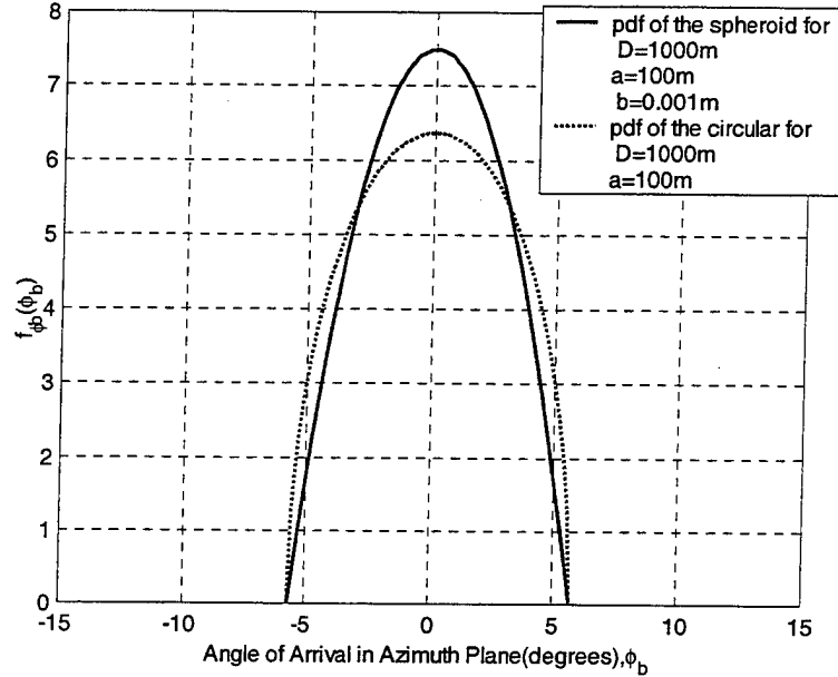
Figure 10. Plot of f_{\phi_b}(\phi_b) versus \phi_b for D=1000\text{m} , a=100\text{m} and b=0.001\text{m} . Also shows the AOA p.d.f. for a circular spatial model for D=1000\text{m} and a=100\text{m} .
