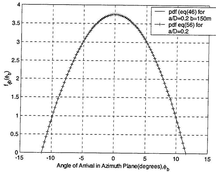
Figure 12. Plot of f_{\phi_b}(\phi_b) versus \phi_b for D=1000\text{m} , a=200\text{m} and b=150\text{m} (using the two different formulas).
