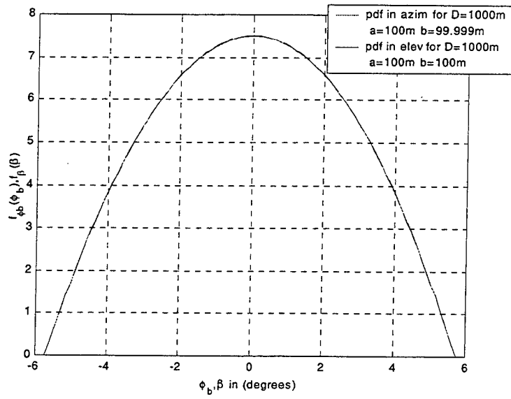
Figure 20. Plot of f_{\phi_b}(\phi_b) versus \phi_b and f_{\beta}(\beta) versus \beta for D=1000\text{m} , a=100\text{m} and b=99.999\text{m} and for D=1000\text{m} , a=100\text{m} and b=100\text{m} respectively.
