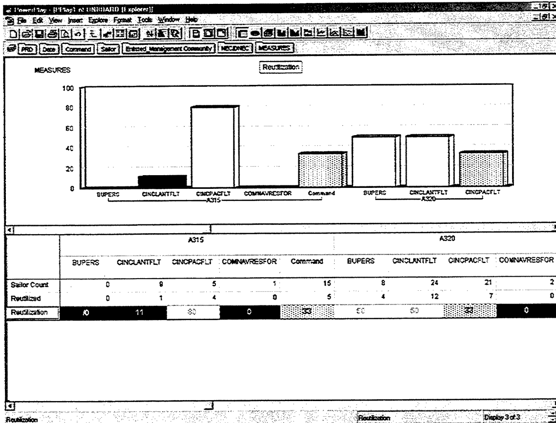
Figure 31. ECM/MCA View of %NECReutilizationOnboard Performance Metric
