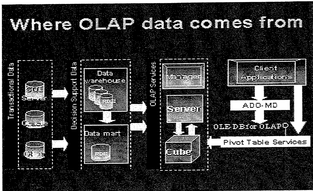
Figure 2. Microsoft HOLAP Architecture (Microsoft Corp.)
