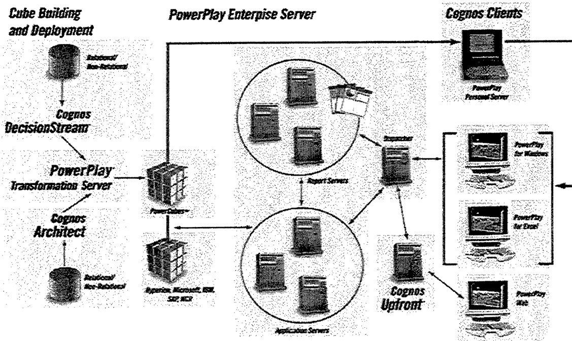
Figure 16. PowerPlay™ Enterprise Server Architecture (Cognos Corp.)
