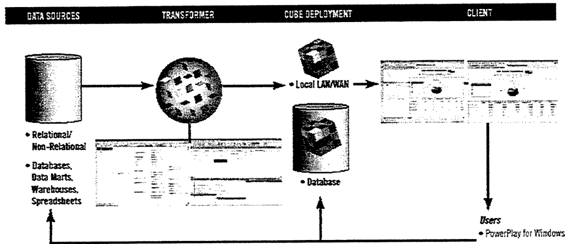
Figure 19. Cognos PowerPlay™ Architecture (Cognos Corp.)
