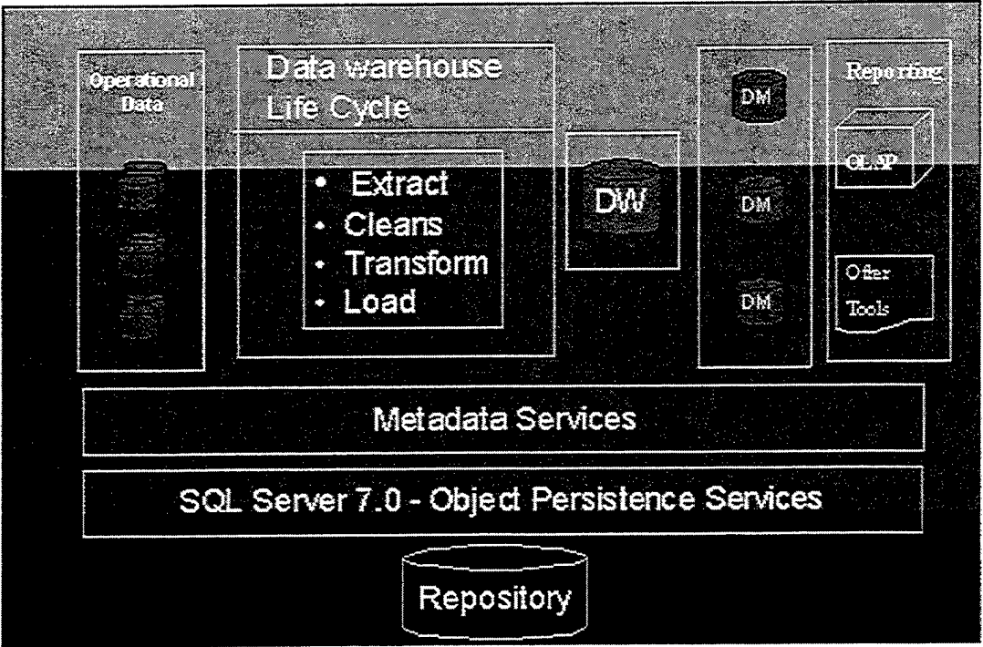
Figure 33. Data Warehouse Architecture & Repository (Cross, Rahimi, 1999)
