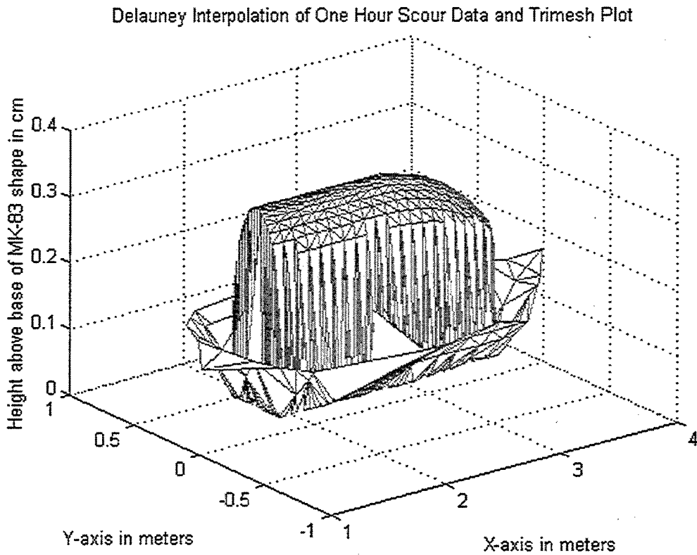
Figure 13 Trimesh Plot of Interpolated Data for Scour after One Hour
