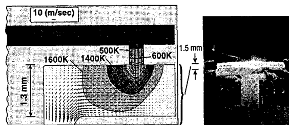
Figure 14: 200 watt microcombustor.
