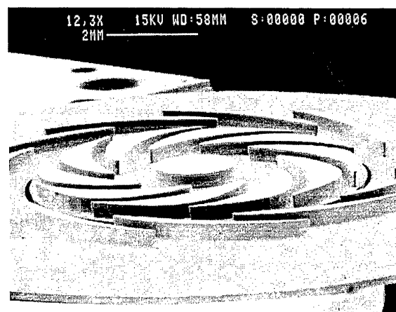
Figure 11: Microcompressor with 8 mm dia rotor.
