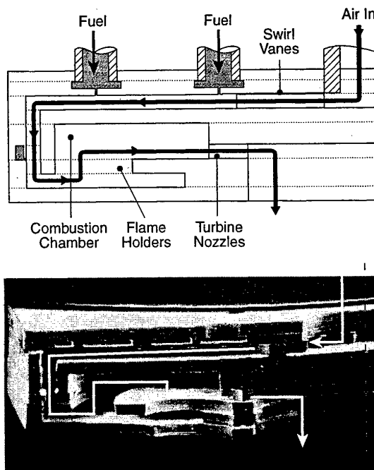
Figure 13: Microcombustor which comprises the static structure of the demo engine of Figure 5.
