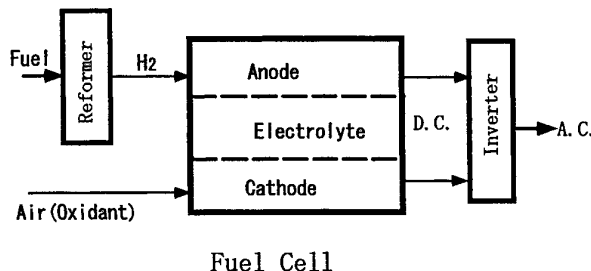
Fig.2 Fuel Cell System
