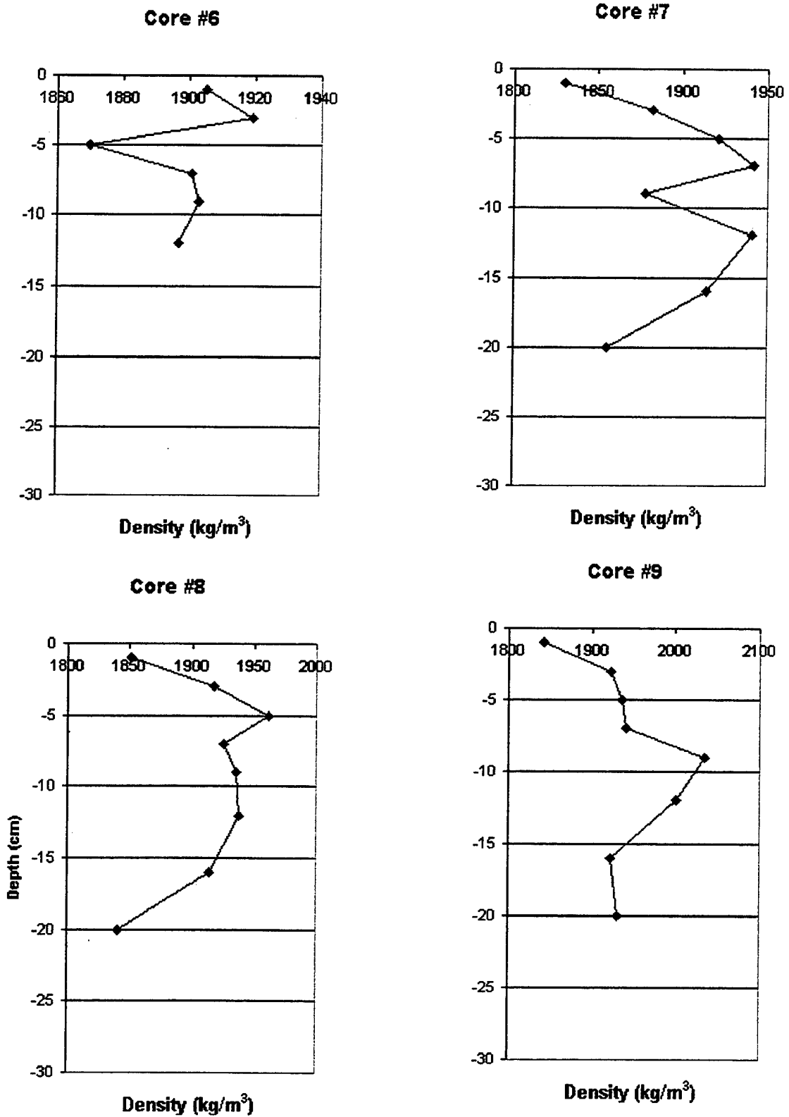
Figure 12. Density Vs. Depth for Cores 6-9.
