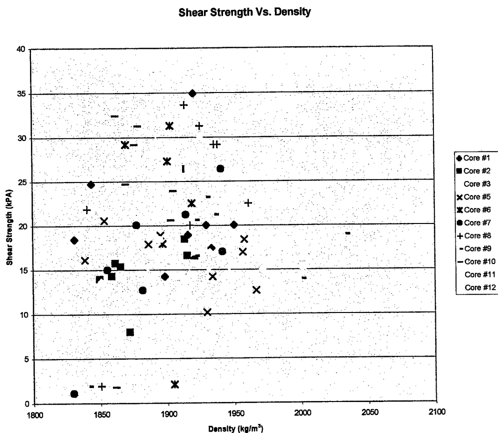
Figure 17. Shear Strength Vs. Density analyzed on June 1, 2000.
