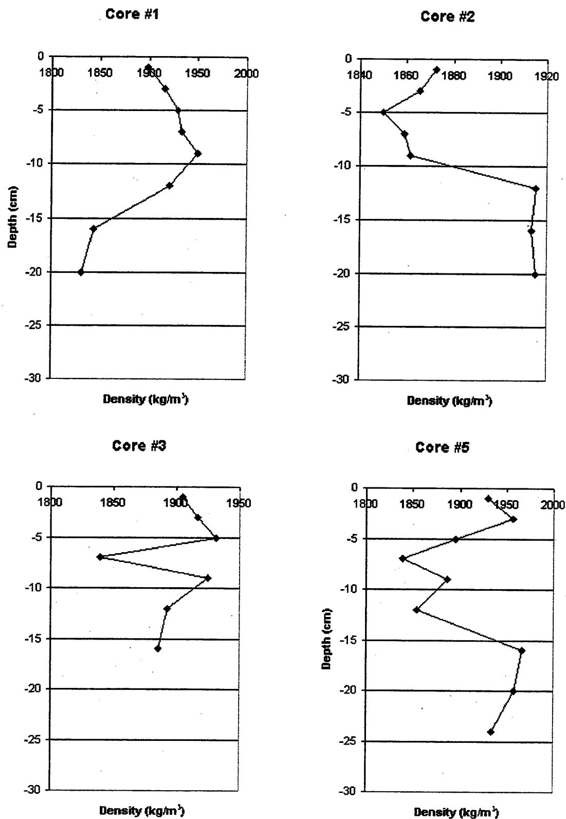
Figure 11. Density Vs. Depth For Cores 1-3, 5.
