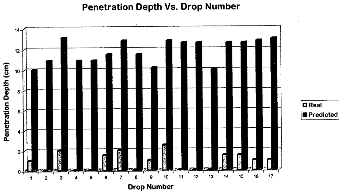
Figure 20. Measured versus Impact Burial Model output for May 23, 2000.
