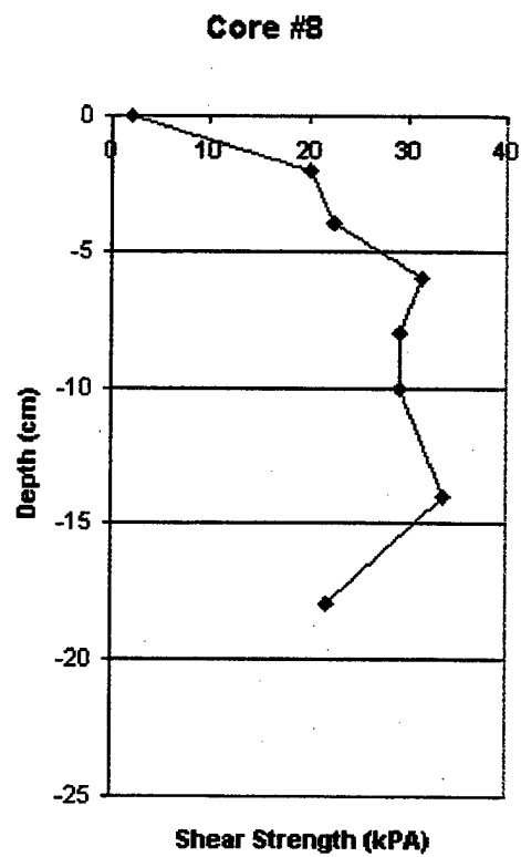
Figure 15. Shear Strength Vs. Depth for Cores 6-9.
