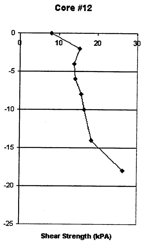
Figure 16. Shear Strength Vs. Depth for Cores 10 – 12.
