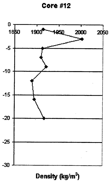
Figure 13. Density Vs. Depth for Cores 10-12.
