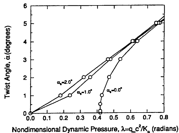
Figure 3.3 Divergence and Post-Divergence of an Airfoil Including Transonic Nonlinear Inviscid Aerodynamics: NACA 64A010A Airfoil Section, M = 0.80 , Elastic Axis Location, a = c/b = 0.0
