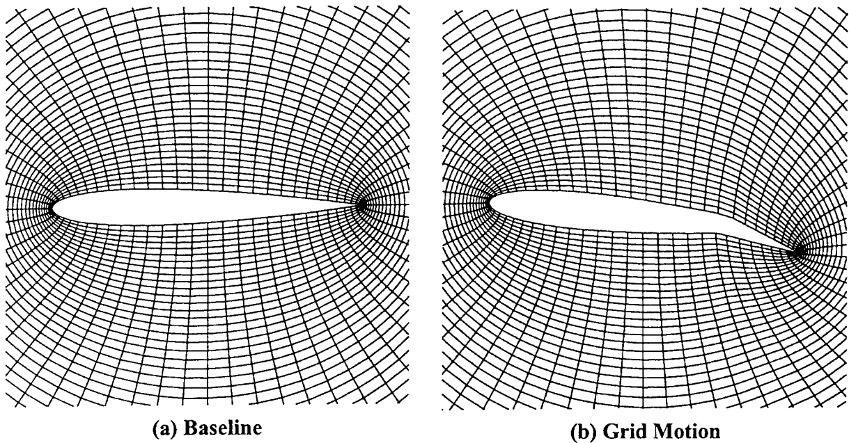
Figure 2.4 NACA 0012 Grid: 65 x 97 Computational Nodes, Outer Boundary Radius=15c
