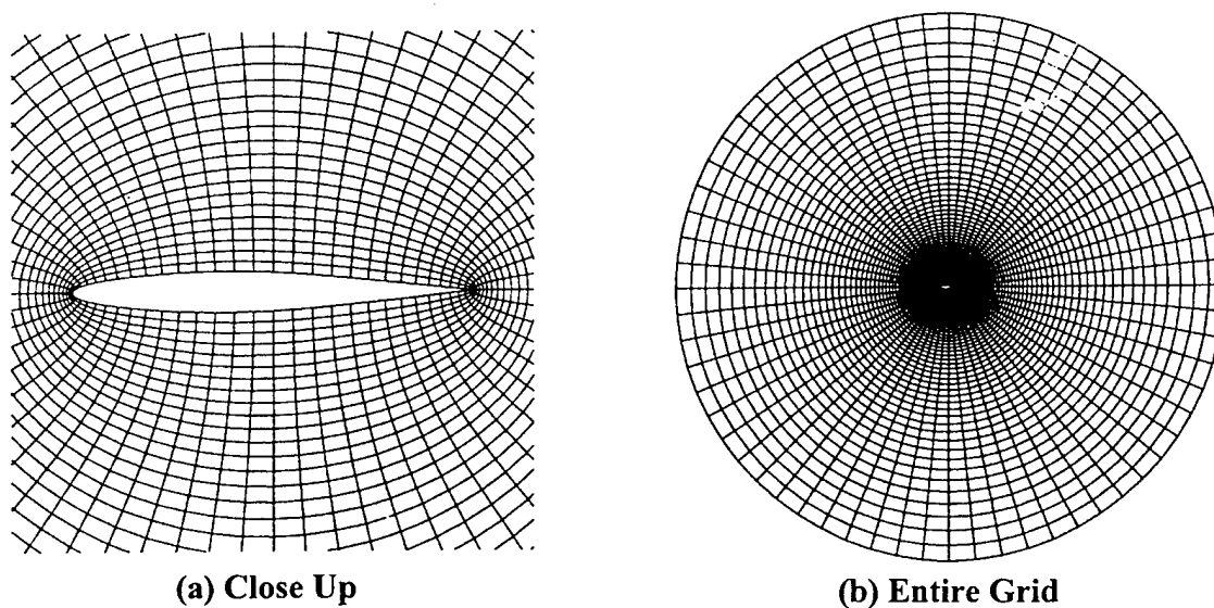
Figure 3.1 NACA 64A010A Computational Grid
