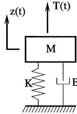
Figure 6-1: An SDOF spring-mass-dashpot system.
