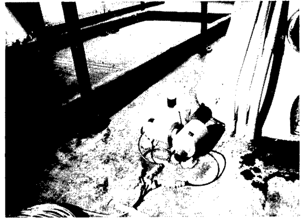
Fig. 22. Triaxial geophone array at WES station 2.
