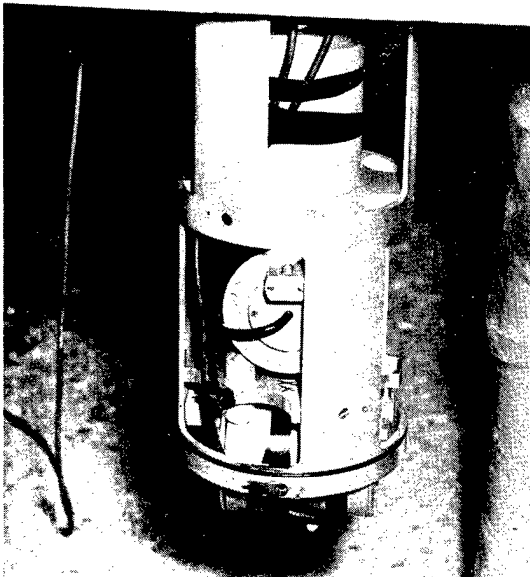
Fig. 17. LRL triaxial mounting frame for velocity detectors.
