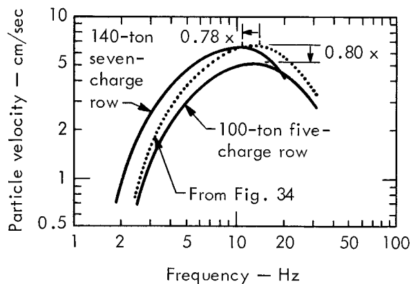
Fig. 36. Shift of amplitude-frequency curve for 100-ton and 140-ton row charges (Ref. 7).
