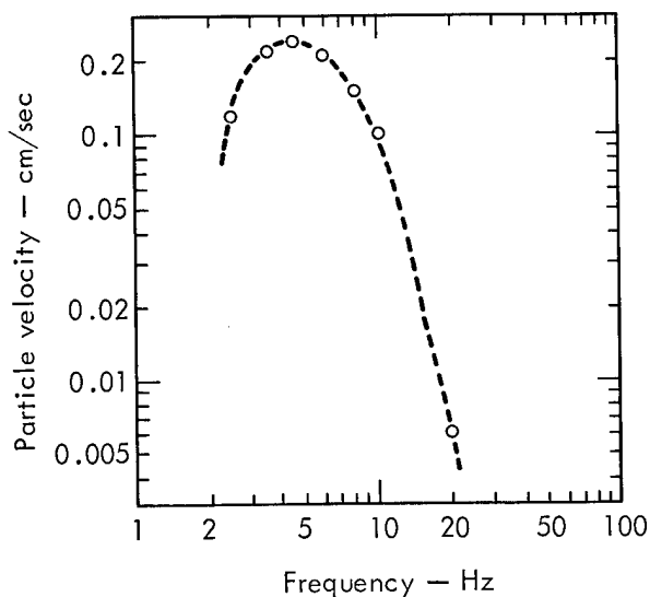
Fig. 35. Spectrum of peak ground motion at Fort Peck Dam ( R = 18.5 km), derived from Fig. 34 (Ref. 7).
