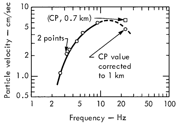
Fig. 34. Derived values of V_0 for R_0 = 1 km (Ref. 7).
