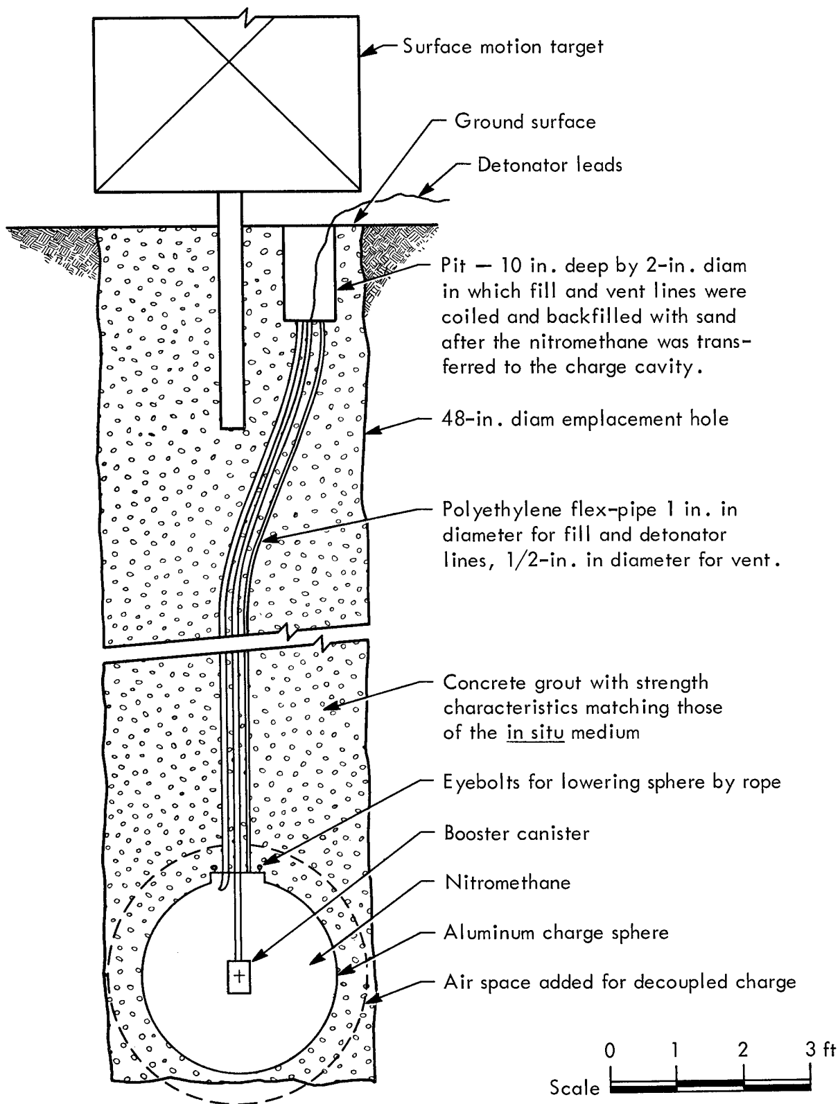
Fig. 11. Emplacement of 1000-lb nitromethane charge sphere for seismic decoupling series.
