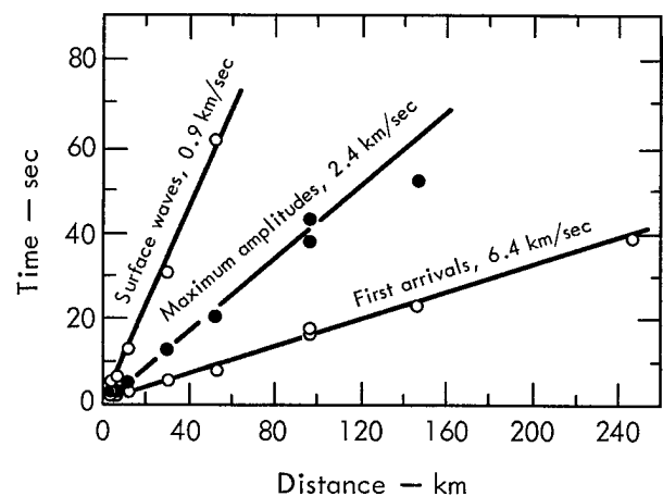
Fig. 31. Travel times for Pre-Gondola II.
