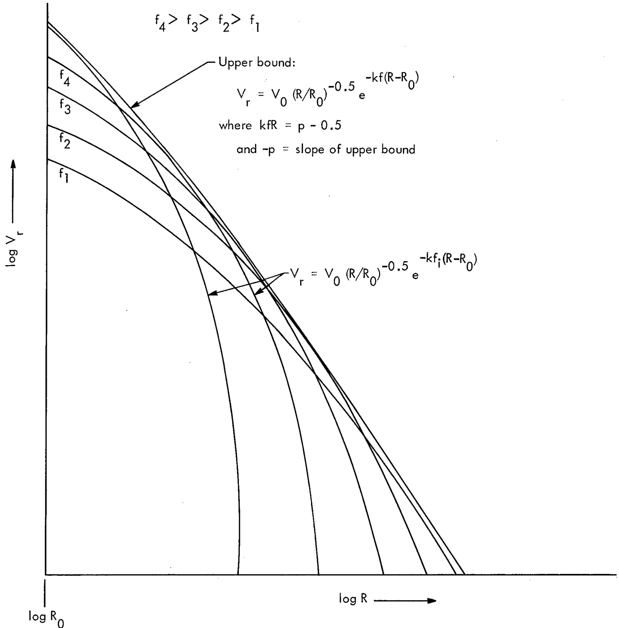
Fig. 32. Idealized representation of attenuation curves and their upper bound (Ref. 7).
