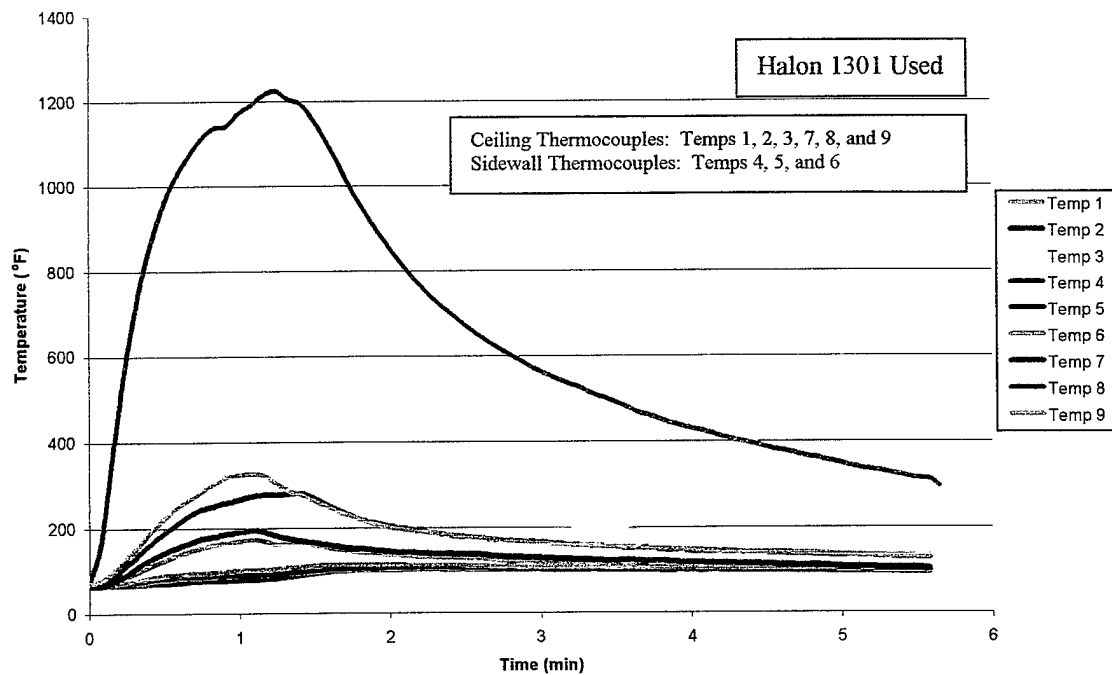
FIGURE 48. SURFACE BURN TEST 15 (111899T4) TEMPERATURE PLOT
