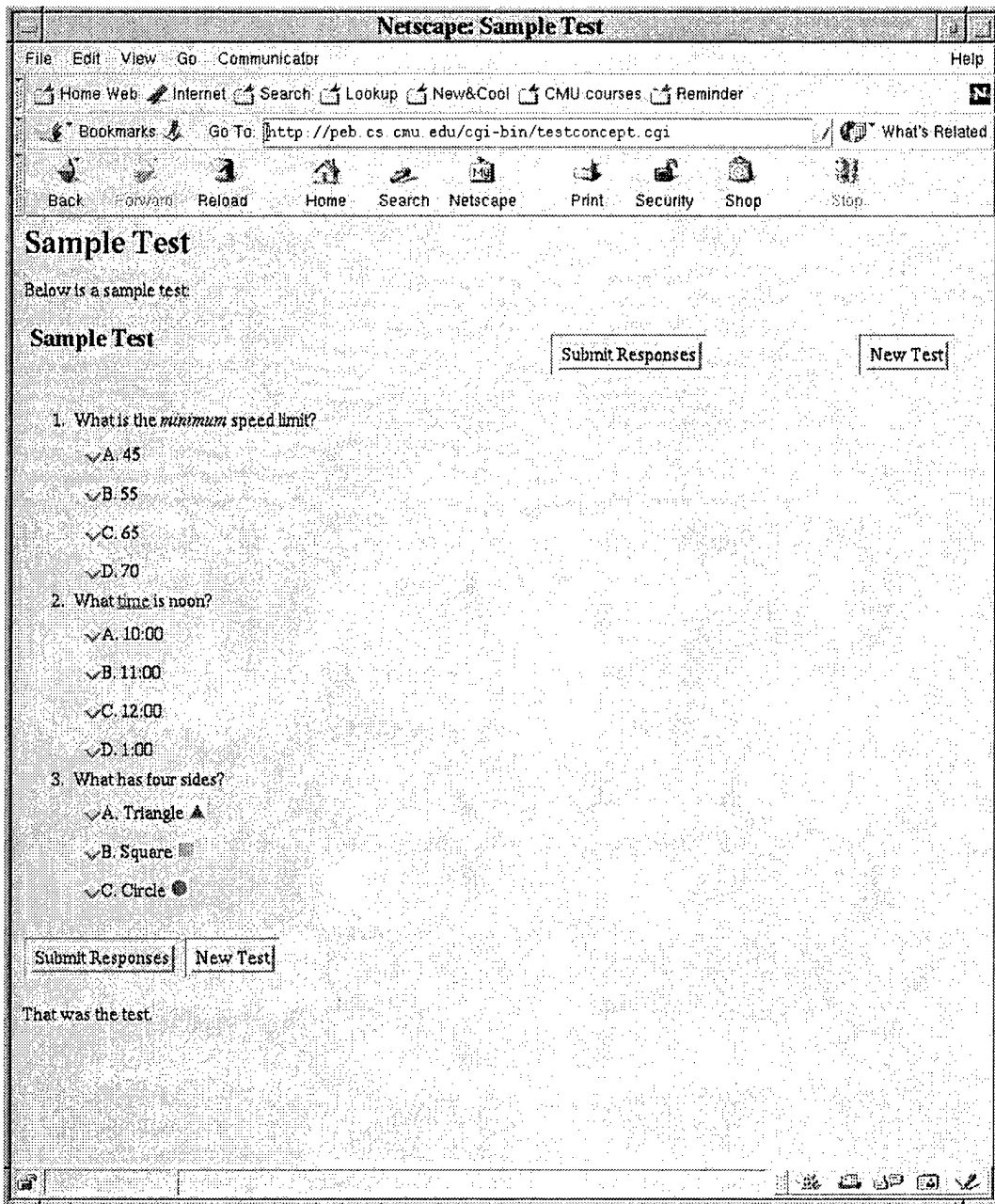
Figure 7: Initial page for a sample concept test
