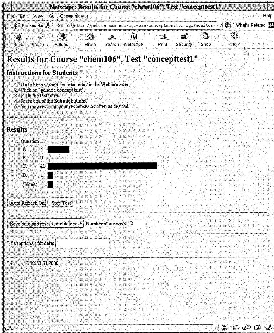
Figure 14: Page monitoring generic concept test
