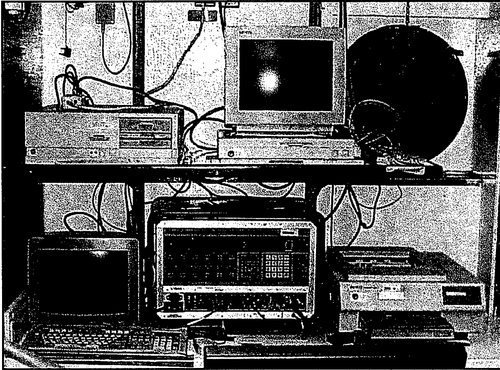
Figure 4-4 A/N UMQ-12 Mini-rawinsonde system.
