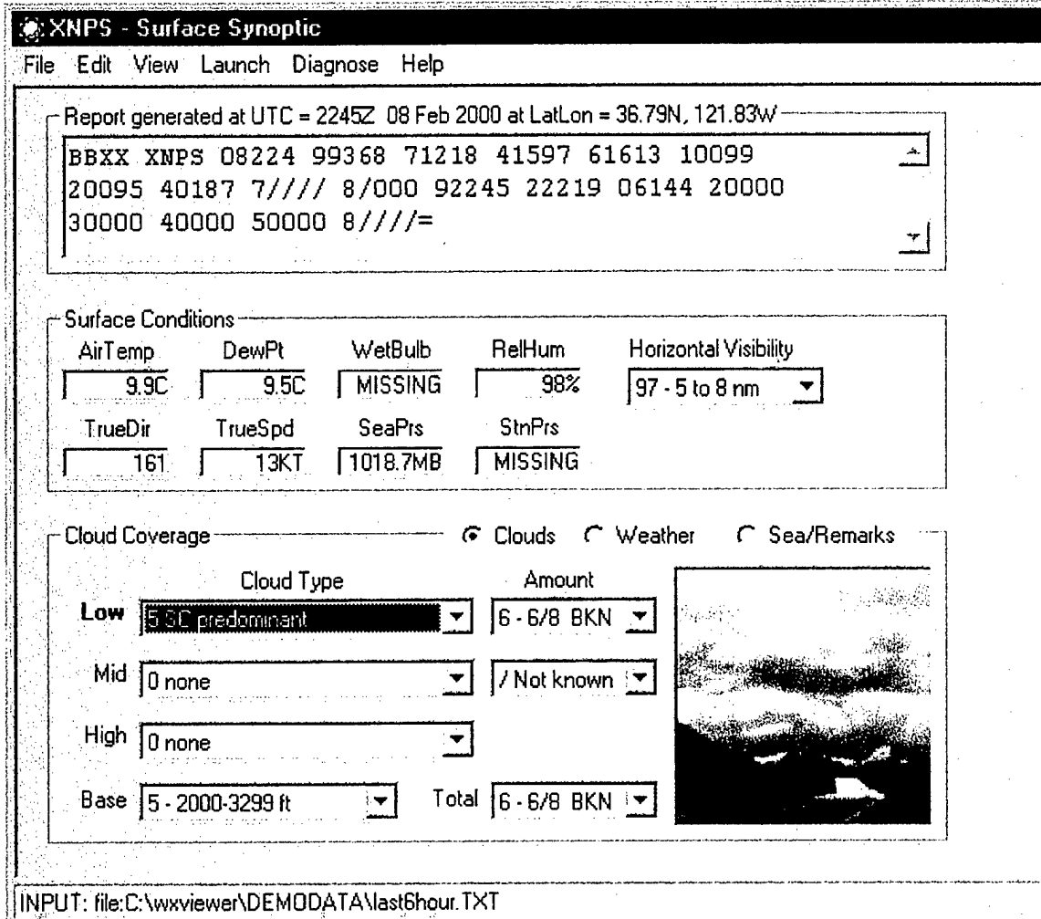
Figure 7-1 WxViewer Client Surface Synoptic Observation input screen.
