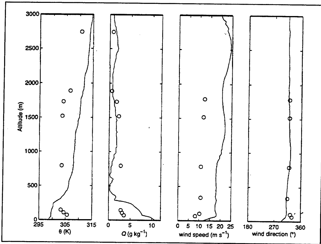
Figure 3-1 Profiles of potential temperature ( \theta ), total water mixing ratio ( Q ), wind speed, and wind direction taken at Kuwait International Airport at 1200 UTC (○) and from a rawinsonde observation taken on board USS Caron at 26°09'N 053°06'E at 1330 UT (—) on 28 APR 1996 (from Brooks, 1998).
