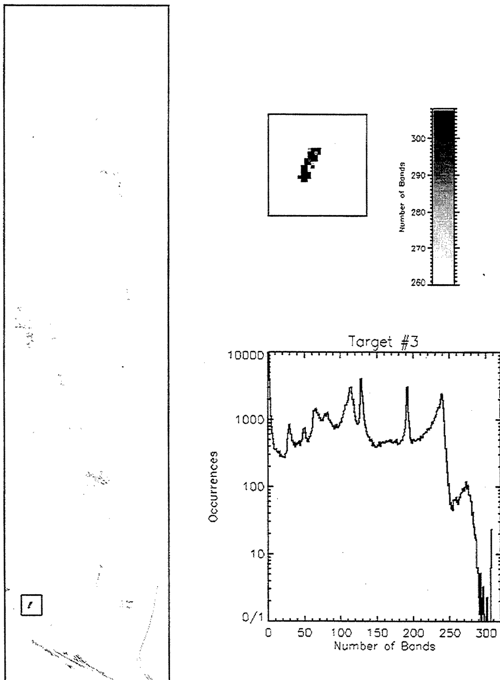
Fig. B.19 Parallelepiped Rule Image for Target #3
