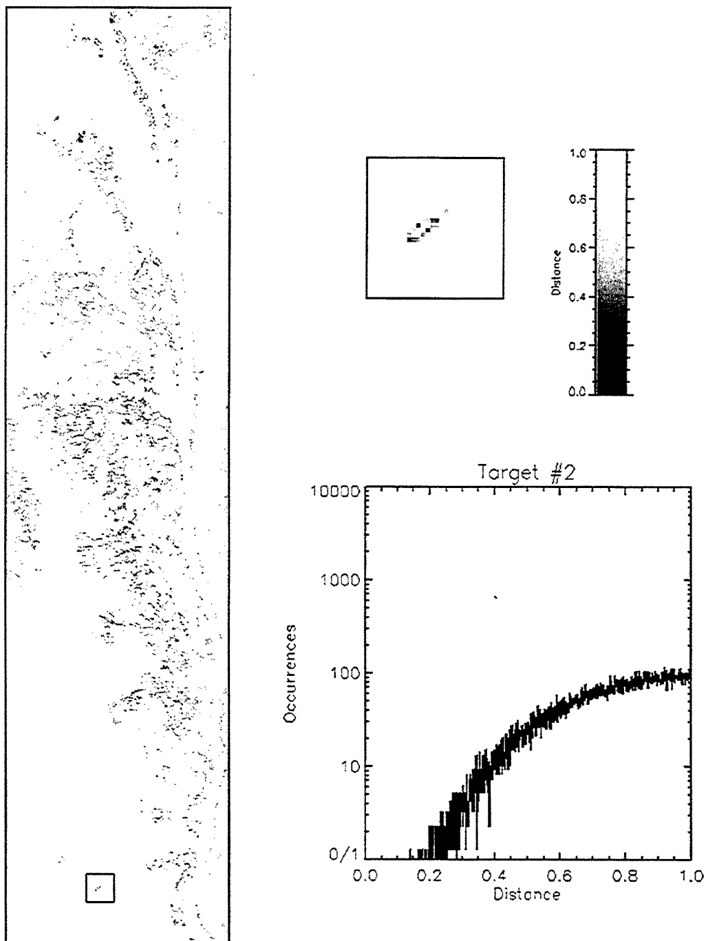
Fig. B.30 Minimum Distance Rule Image for Target #2
