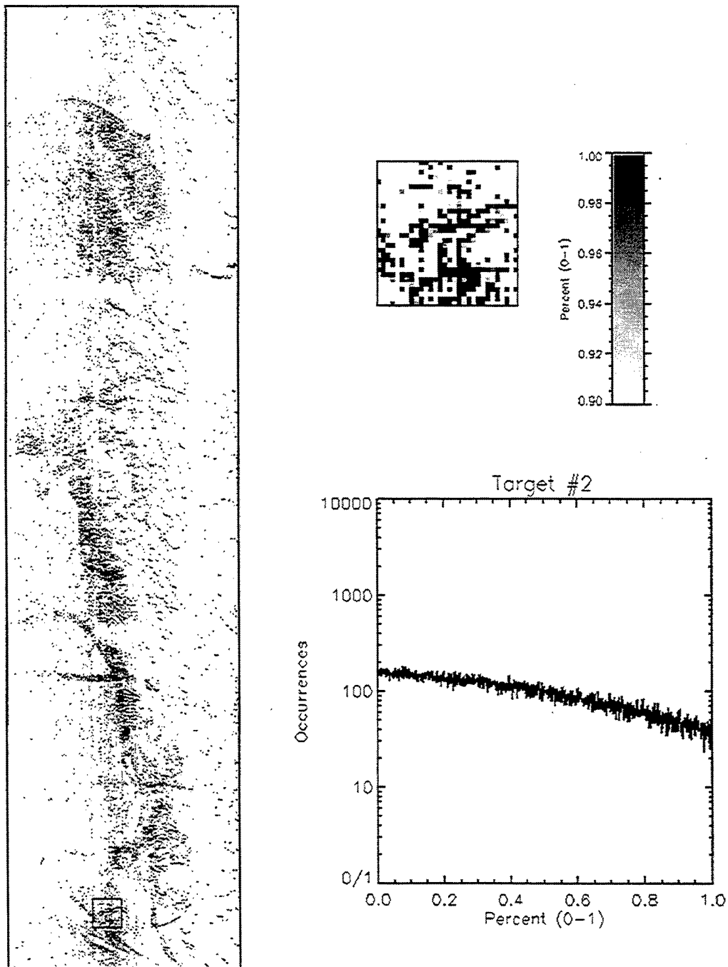
Fig. B.47 Linear Spectral Unmixing Rule Image for Target #2
