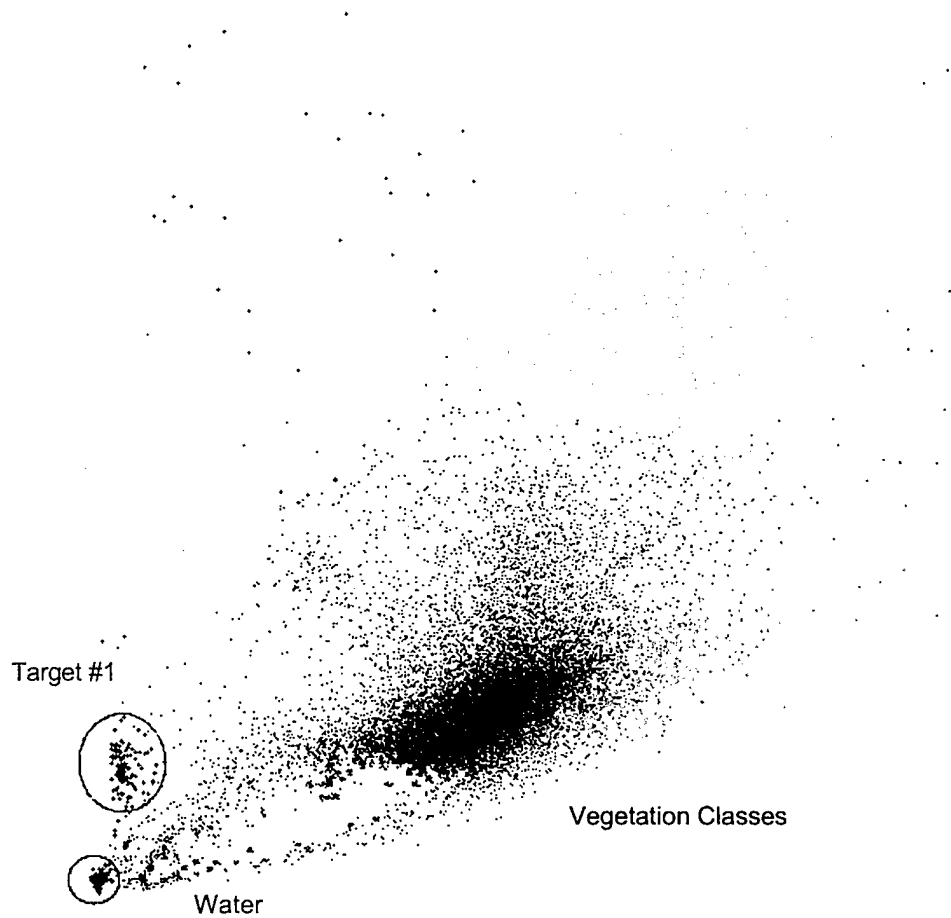
Fig. 5.5 Illustration of Using N-Dimensional Visualizer to Separate Spectral Classes
