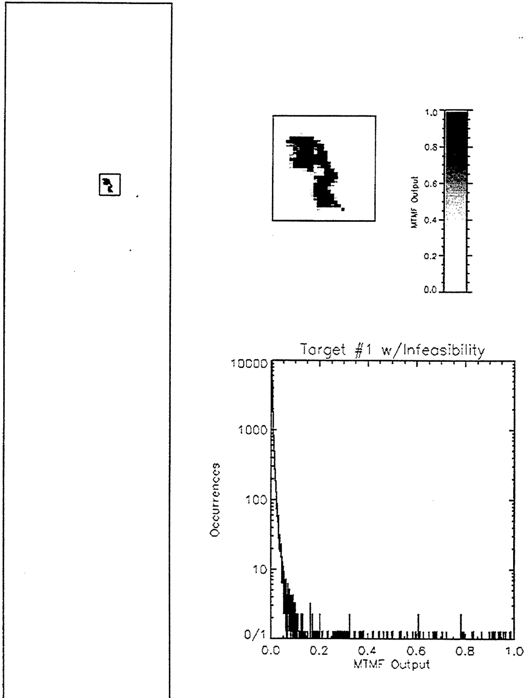
Fig. B.54 MTMF TM Rule Image for Target #1
