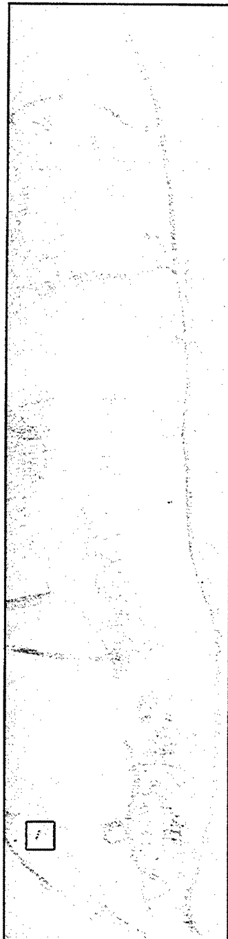
Fig. B.60 Spectral Feature Fitting Rule Image for Target #3
