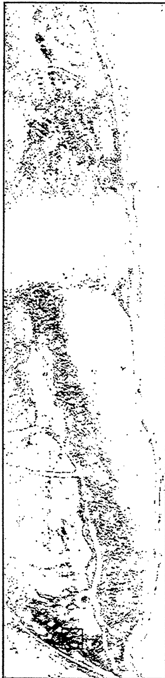
Fig. B.42 Maximum Likelihood Rule Image for Target #2
