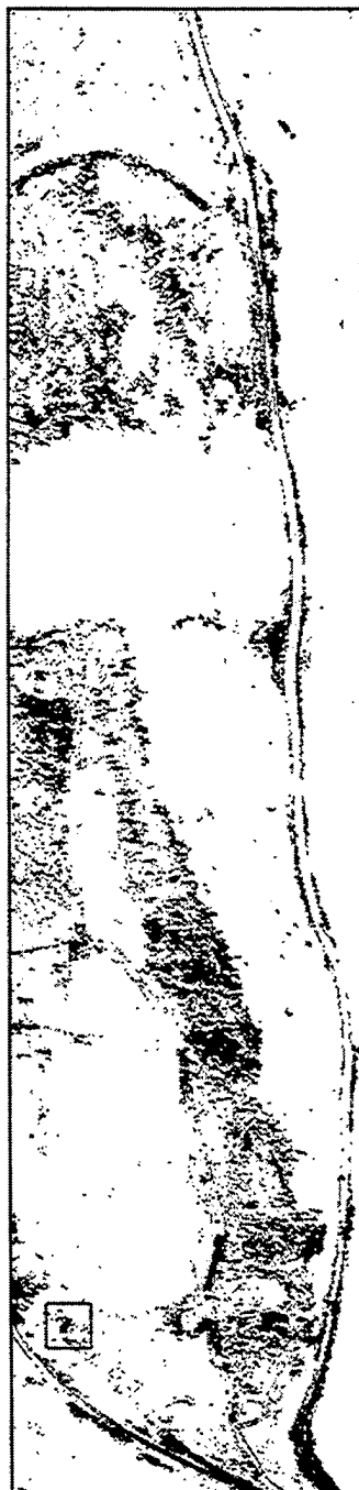
Fig. B.43 Maximum Likelihood Rule Image for Target #3
