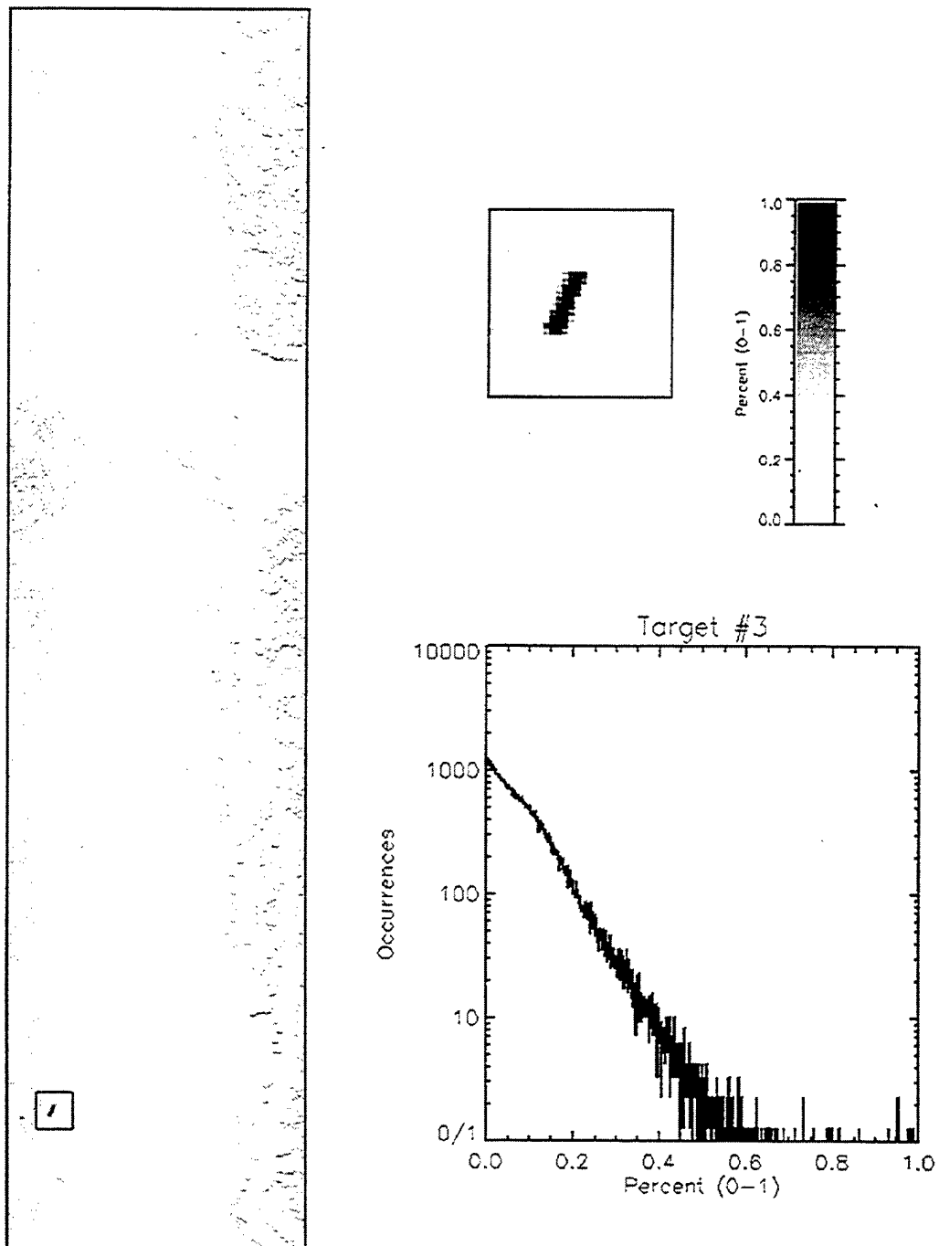
Fig. B.48 Linear Spectral Unmixing Rule Image for Target #3
