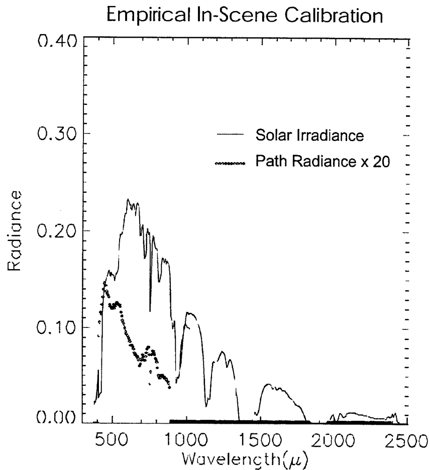
Fig. 5.4 Empirical In-Scene Calibration Coefficients
