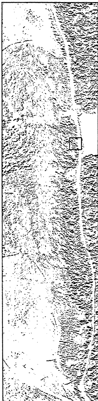
Fig. B.49 Linear Spectral Unmixing Rule Image for Target #4
