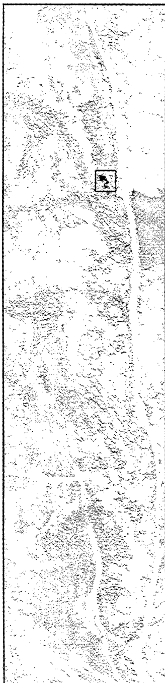
Fig. B.35 Mahalanobis Distance Rule Image for Target #1
