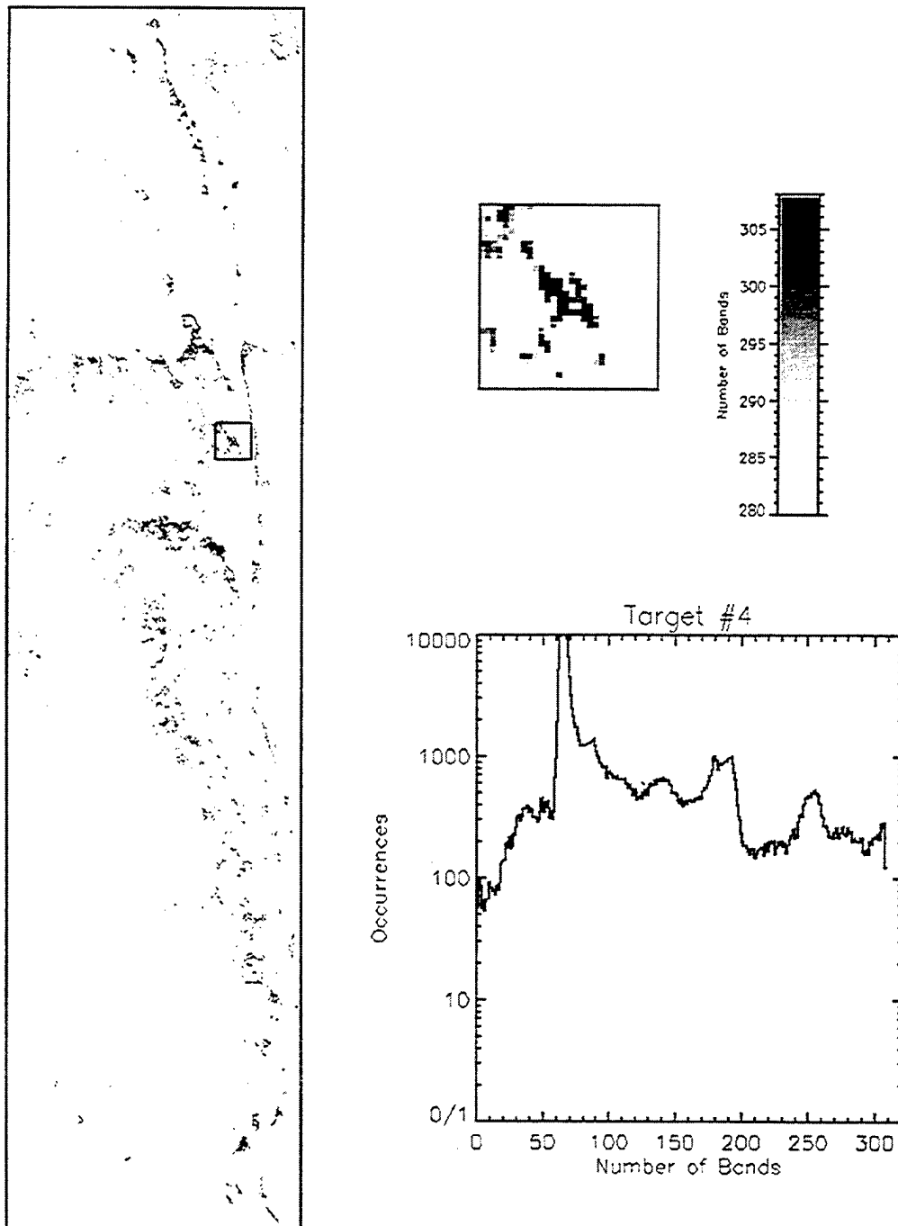
Fig. B.20 Parallelepiped Rule Image for Target #4
