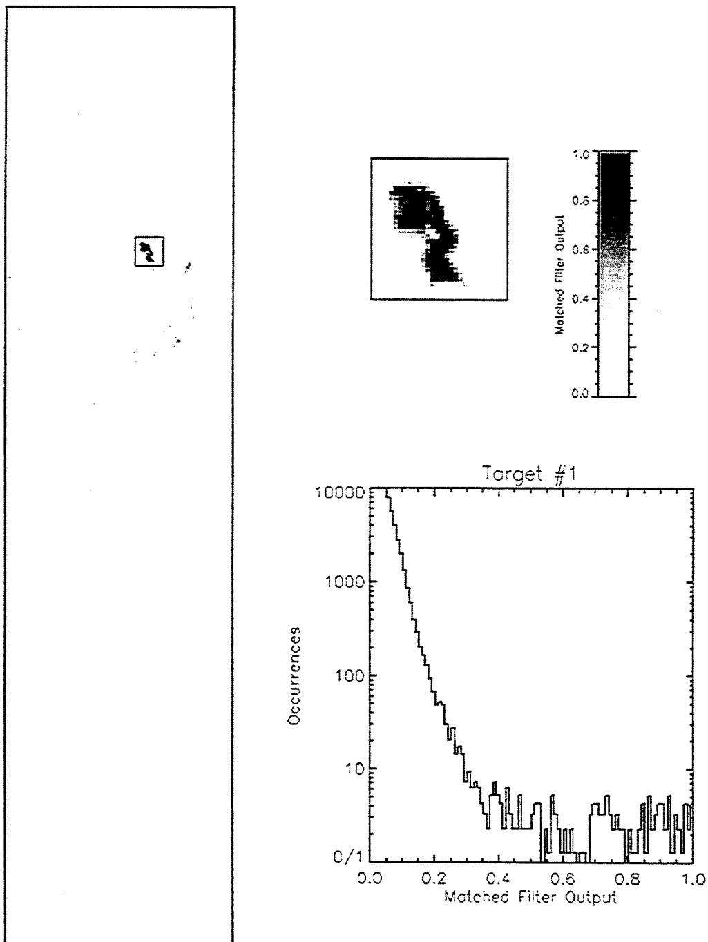
Fig. B.50 Matched Filter Rule Image for Target #1
