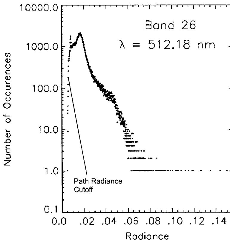
Fig. 4.1 Histogram Illustrating EISC Method
