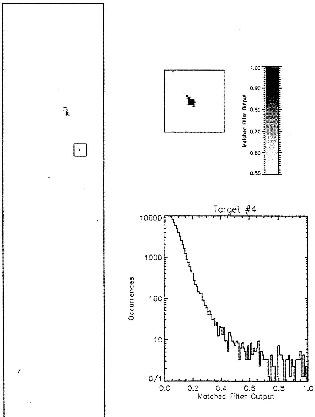
Fig. B.53 Matched Filter Rule Image for Target #4
