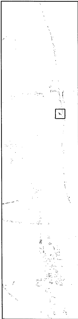
Fig. B.61 Spectral Feature Fitting Rule Image for Target #4
