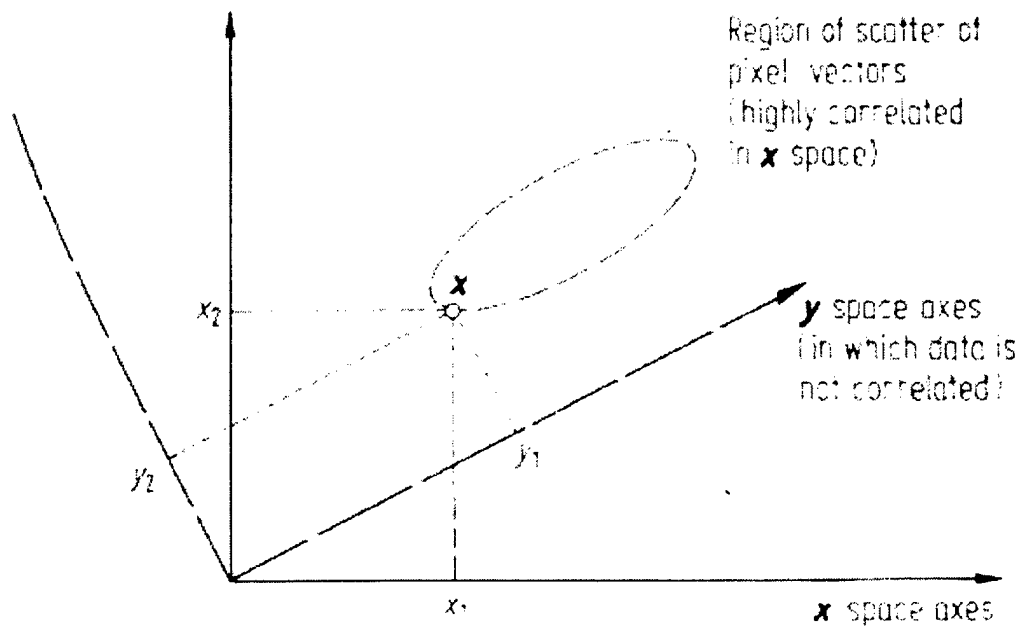
Fig. 4.3 Illustration of a modified co-ordinate system in which the pixel vectors have uncorrelated components (From Richards, 1999)
