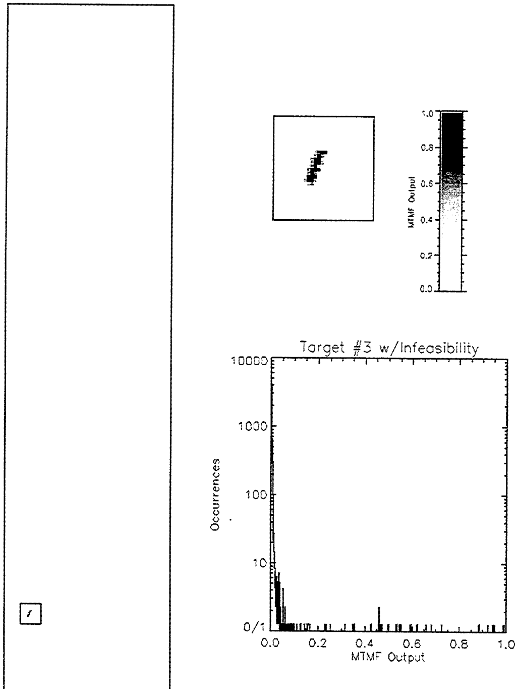
Fig. B.56 MTMF TM Rule Image for Target #3
