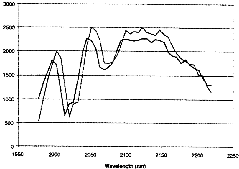
Fig. 3.4 Spectral Shift Due to Smile on SWIR FPA (From Simi, 2000)
