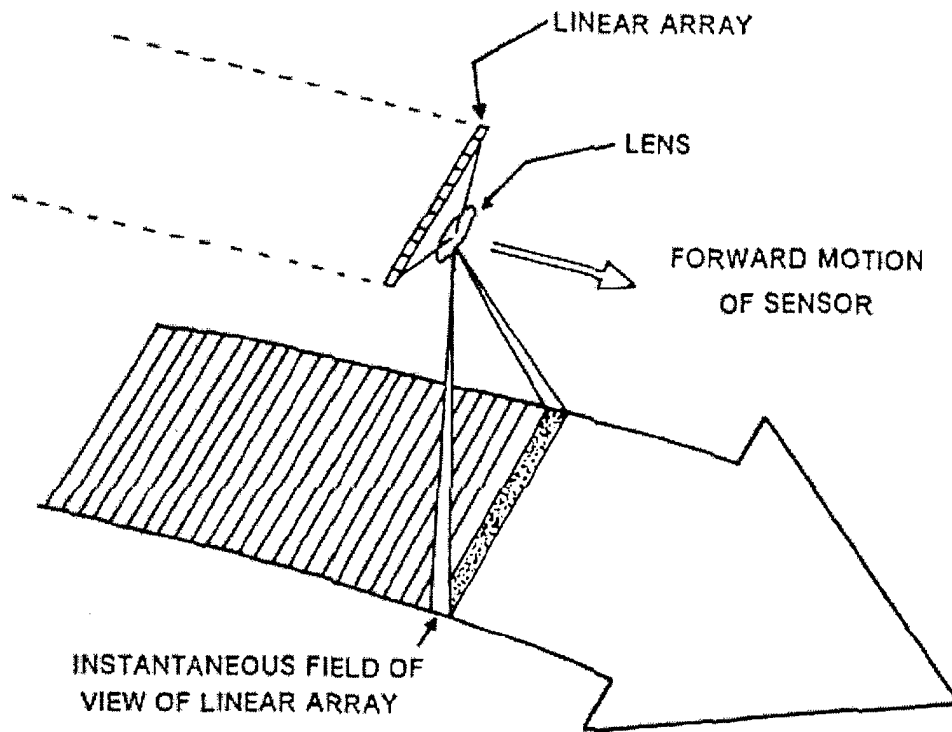
Fig. 2.10 A Pushbroom Scanner (From Campbell, 1996)
