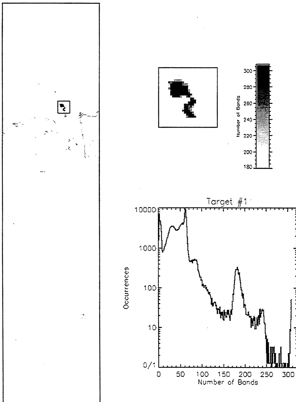
Fig. B.17 Parallelepiped Rule Image for Target #1
