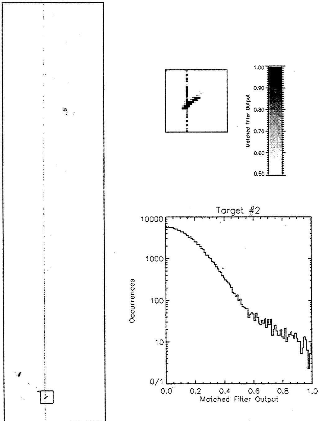
Fig. B.51 Matched Filter Rule Image for Target #2
