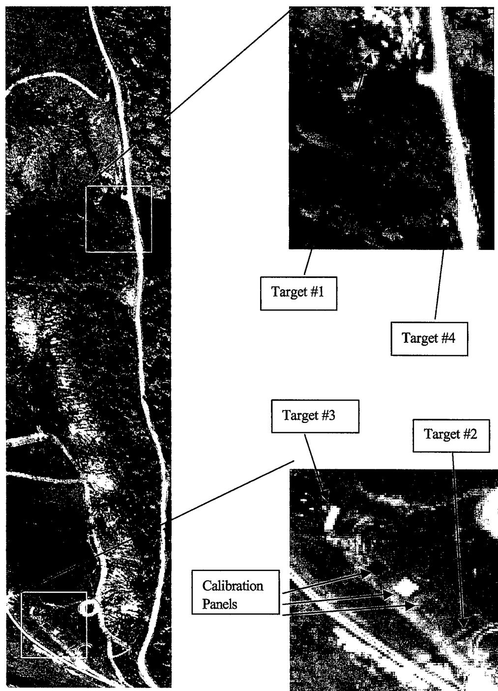
Fig. B.1 False Color Image of the Scene, Illustrating Targets of Interest
