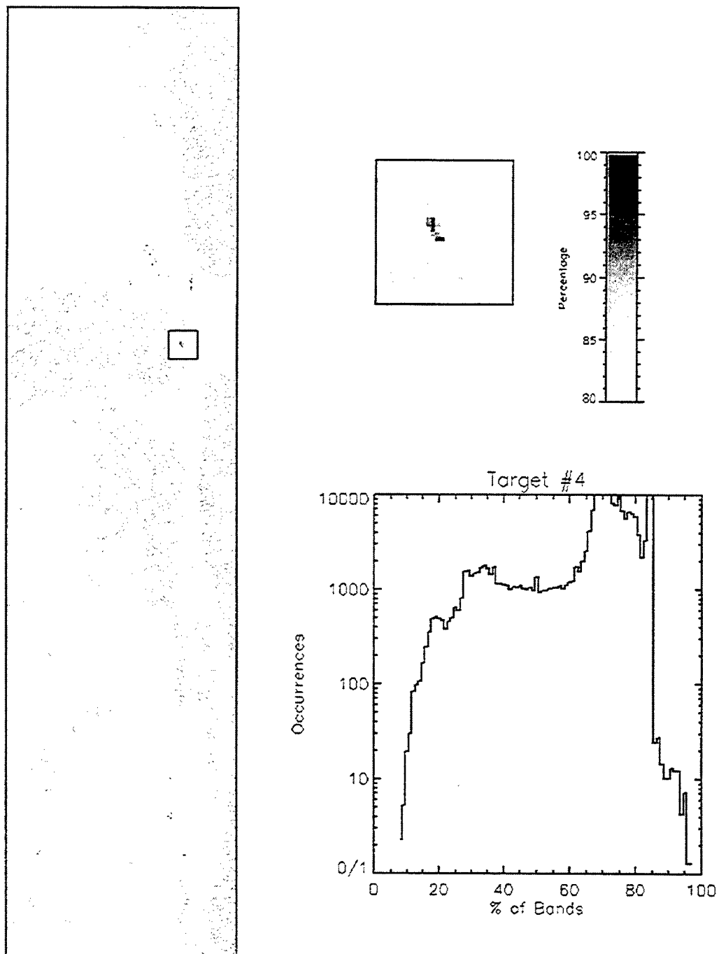
Fig. B.26 Binary Encoding Rule Image for Target #4
