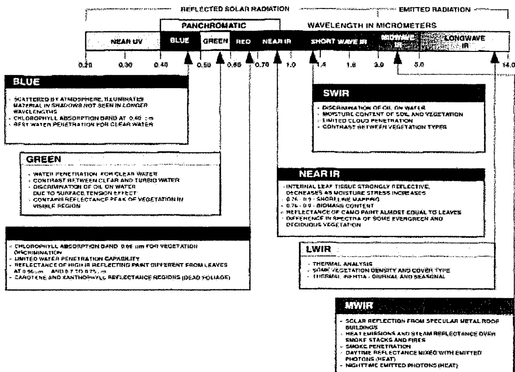
Fig. 2.2 Characteristics of Spectral Regions. (From Multispectral Users Guide, 1995)
