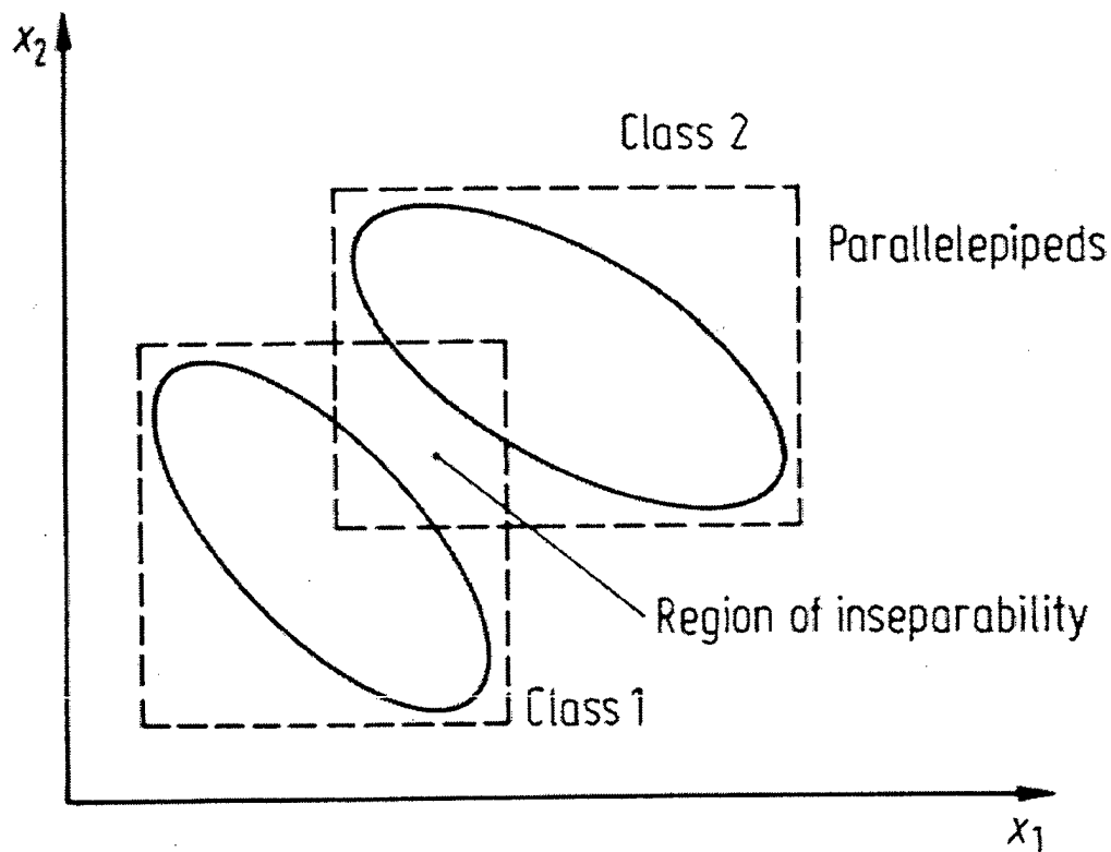
Fig. 4.6 Parallelepiped Classification of Correlated Data Showing Regions of Inseparability (From Richards, 1999)
