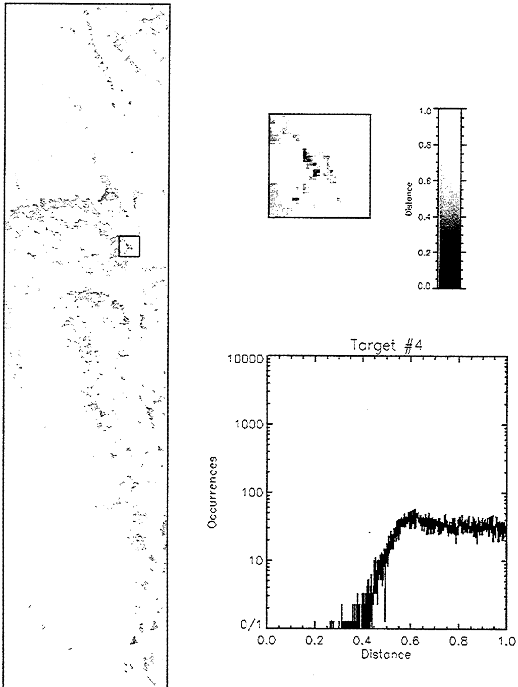
Fig. B.32 Minimum Distance Rule Image for Target #4
