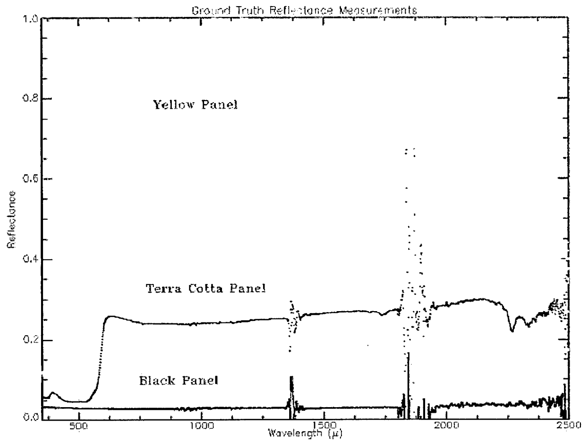
Fig. 5.1 Panel Ground Truth Reflectance
