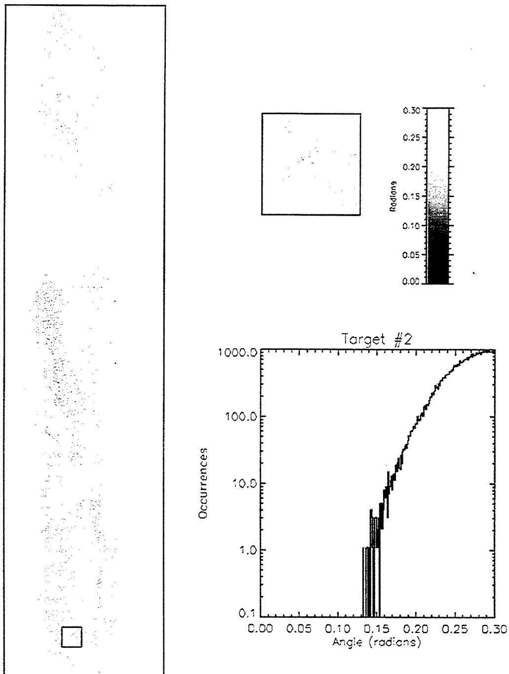
Fig. B.12 ELM SAM Rule Image for Target #2
