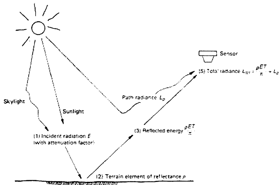
Fig. 2.6 Atmospheric Effects Influencing the Measurement of Reflected Solar Energy (From Lillesand, 1994)
