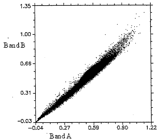
Fig. 4.2 Two-Band Histogram of Hyperspectral Data
