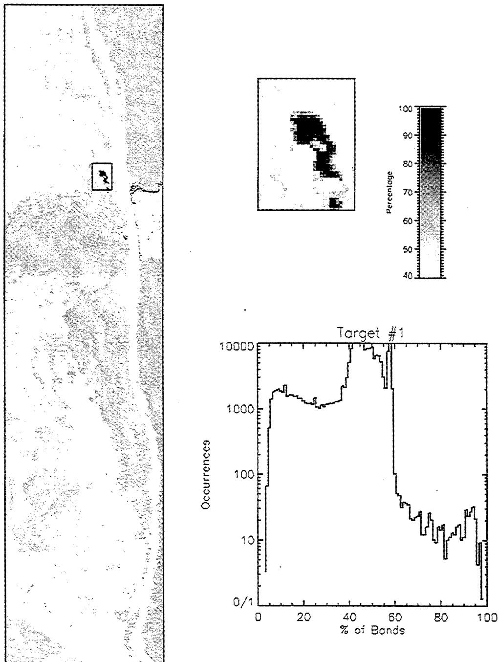
Fig. B.23 Binary Encoding Rule Image for Target #1
