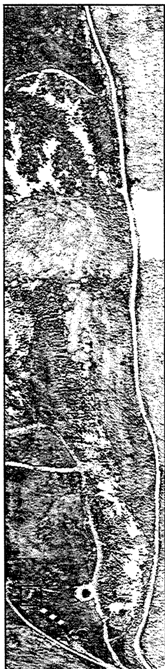
Fig. B.25 Binary Encoding Rule Image for Target #3
