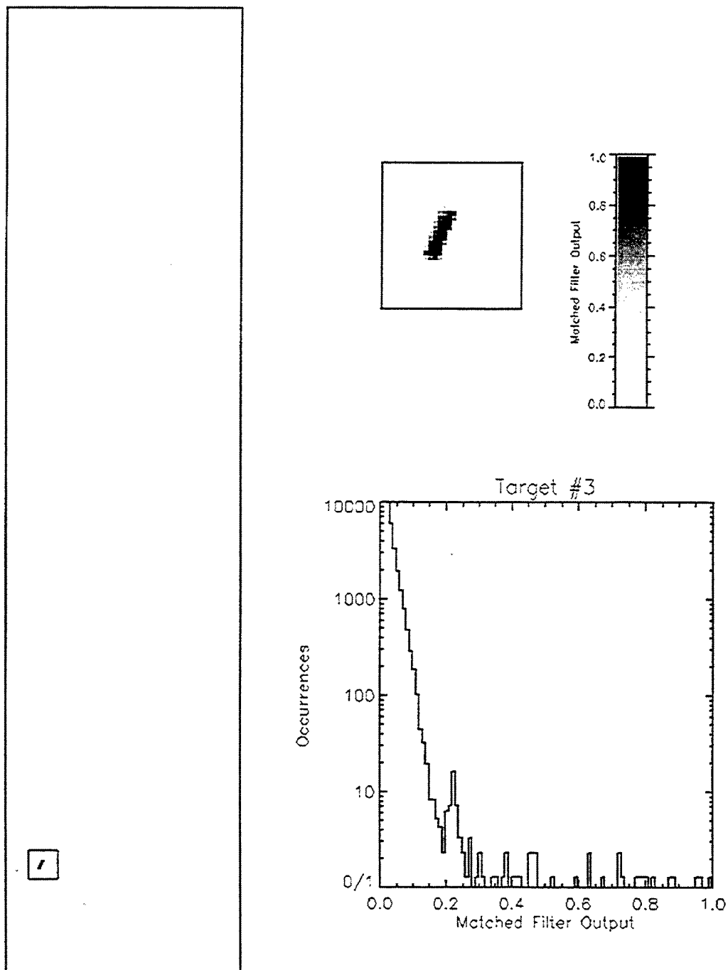
Fig. B.52 Matched Filter Rule Image for Target #3
