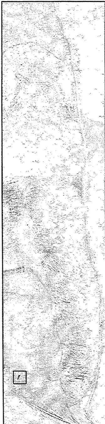
Fig. B.37 Mahalanobis Distance Rule Image for Target #3
