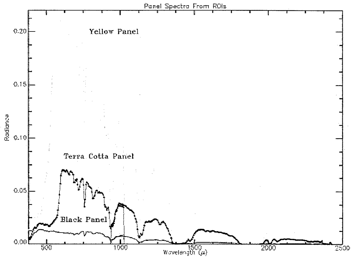
Fig 5.2 Panel Spectra from ROI's
