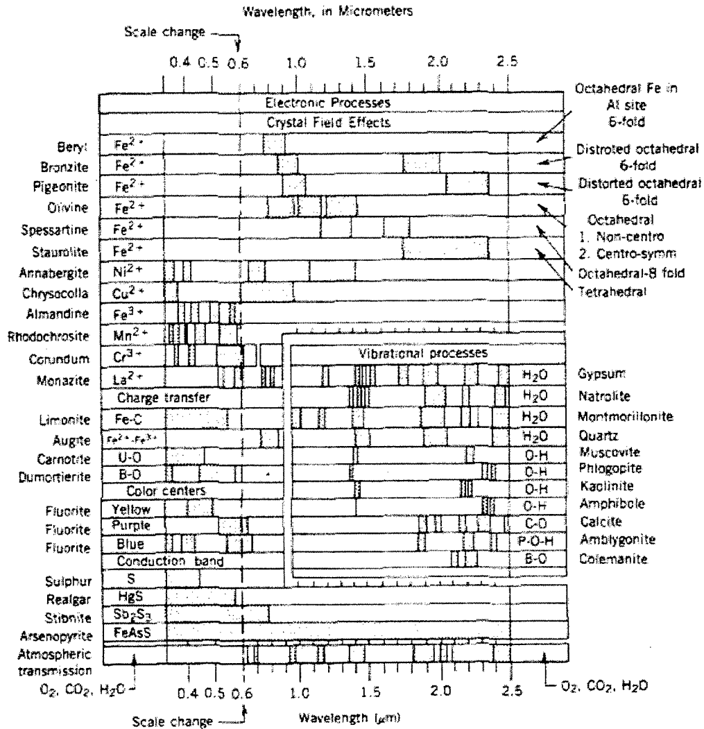
Fig. 2.8 Spectral Signature Diagram of a Variety of Geologic Materials (From Elachi, 1987)
