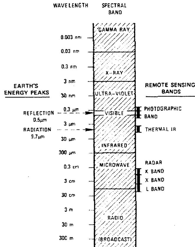
Fig. 2.1 Electromagnetic Spectrum (From Sabins, 1978)
