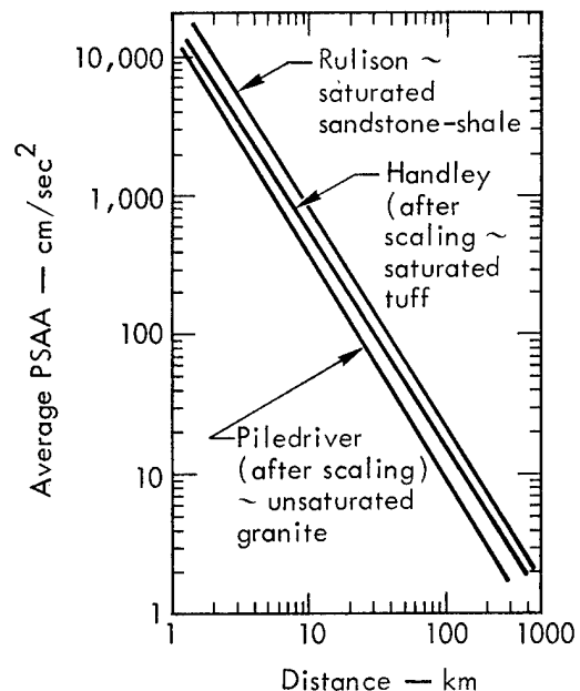
Fig. 4. Distance vs PSAA of Rulison, Handley, and Piledriver Events for 40-kt yield, 8400-ft DOB, and 5% damping.
