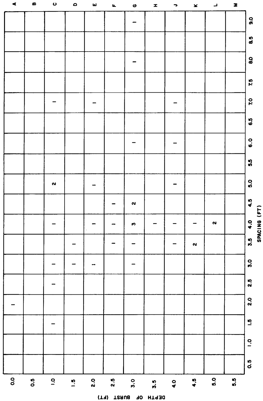
Figure 2.6 Summary of spacings and burst depths used in the row-charge experiment
