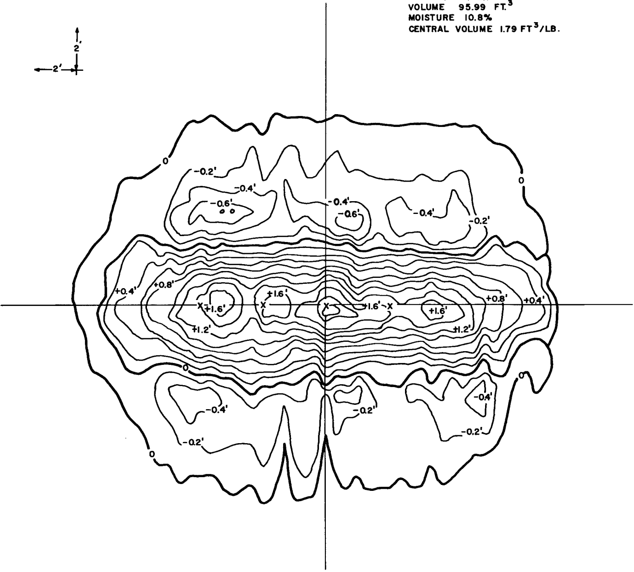
Figure B.3 Crater topography 8-pound row charge buried 1 foot, spaced 2.5 feet
