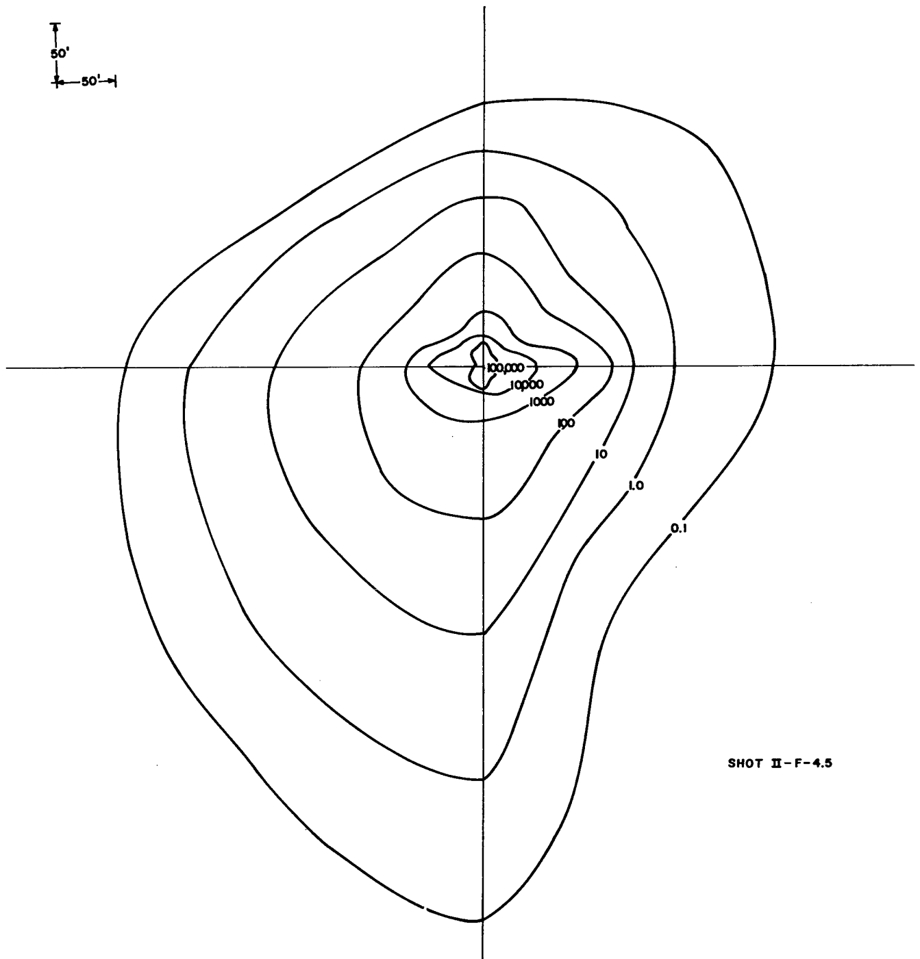
Figure D.31 Throwout deposition, 8-pound row charge, buried 2.5 feet, spaced 4.5 feet-- contours are in \text{gm}/\text{ft}^2
