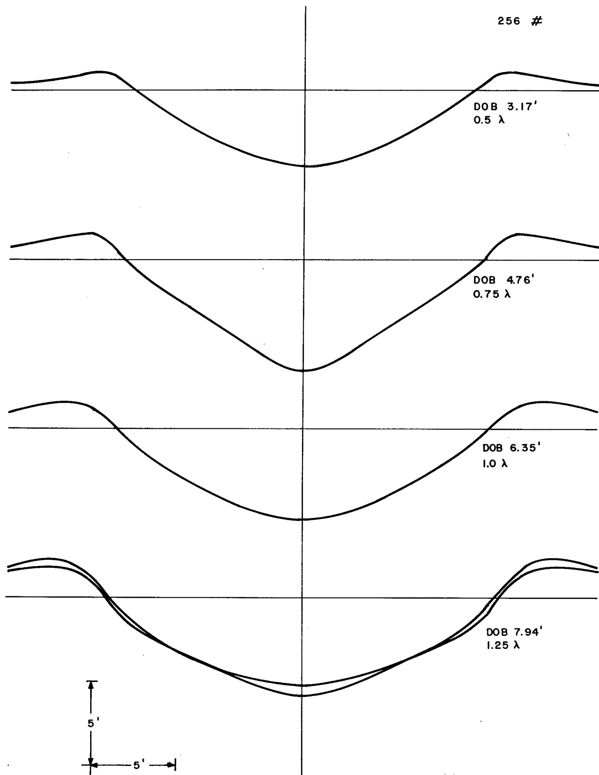
Figure C.1 Profiles of 256-pound single-charge craters
