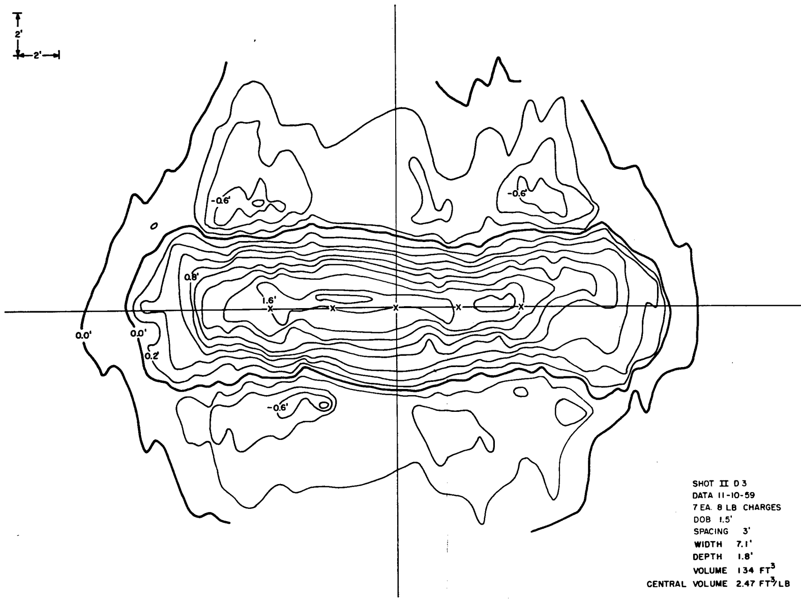
Figure B.9 Grater topography 8-pound row charge buried 1.5 feet, spaced 3 feet
