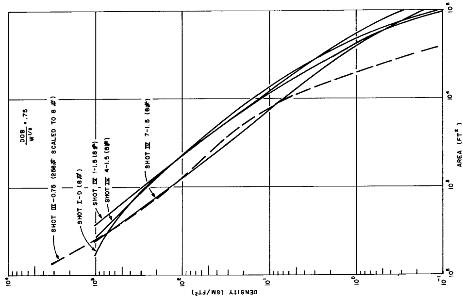
Figure 3.16 Throughout area-density curves for single charges at a scaled burst depth of 0.75 ft/lb 1/3
