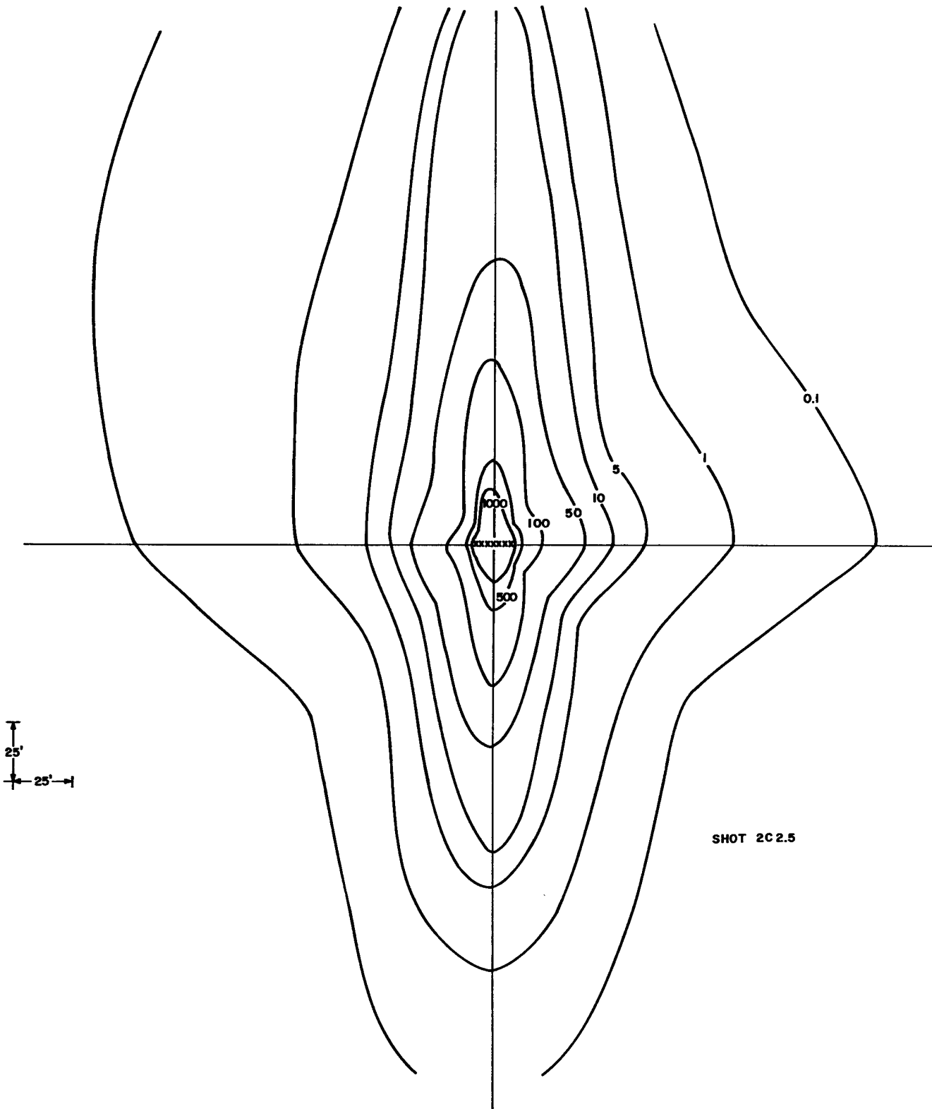
Figure D.26 Throwout deposition, 8-pound row charge, buried 1 foot, spaced 2.5 feet-- contours are in \text{gm/ft}^2
