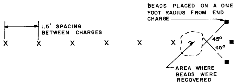
Figure 3.22 Passive evidence of inward motion of debris ejected from the end of the crater
