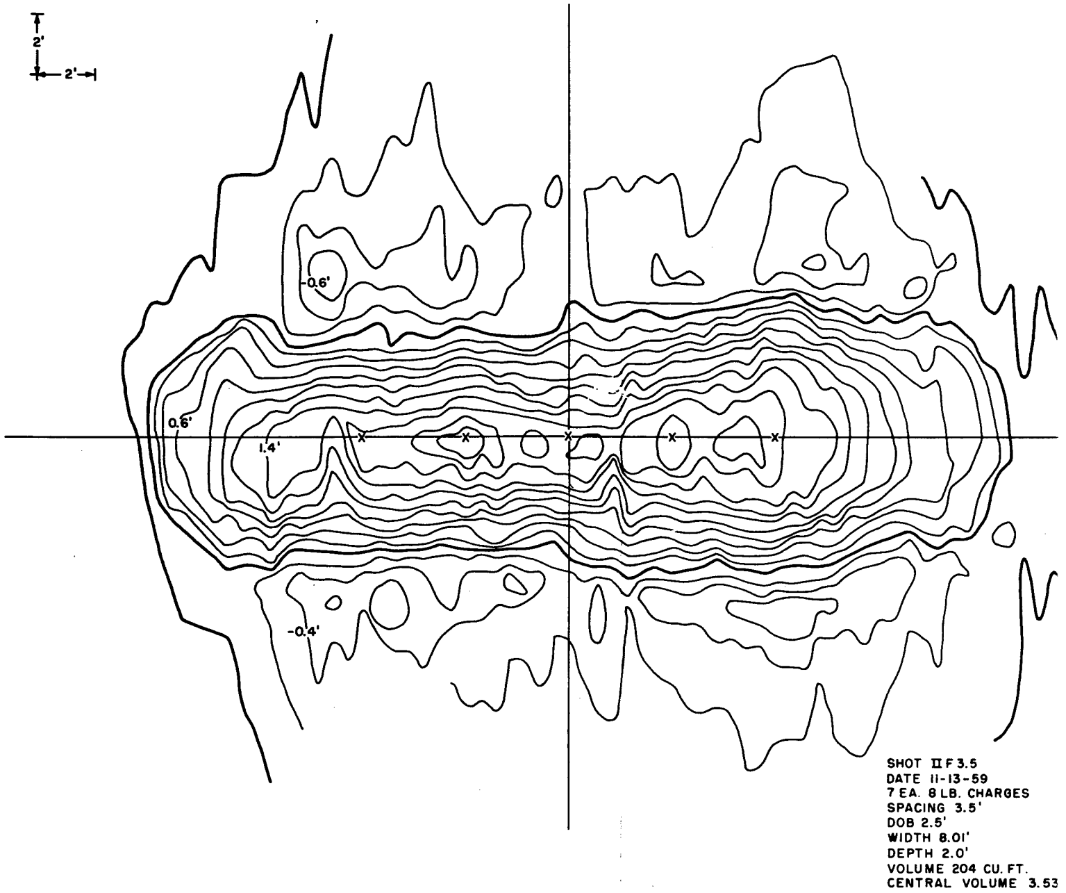
Figure B.15 Crater topography 8-pound row charge buried 2.5 feet, spaced 3.5 feet
