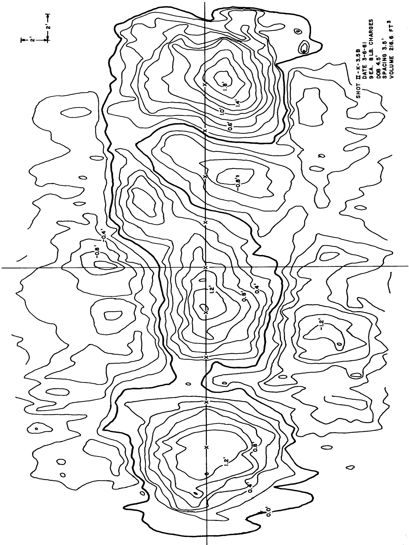
Figure B.33 Crater topography 8-pound row charge buried 4.5 feet, spaced 3.5 feet
