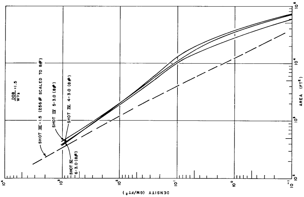
Figure 3.19 Throughput area-density curves for single charges at a scaled burst depth of 1.15 ft/lb 1/3
