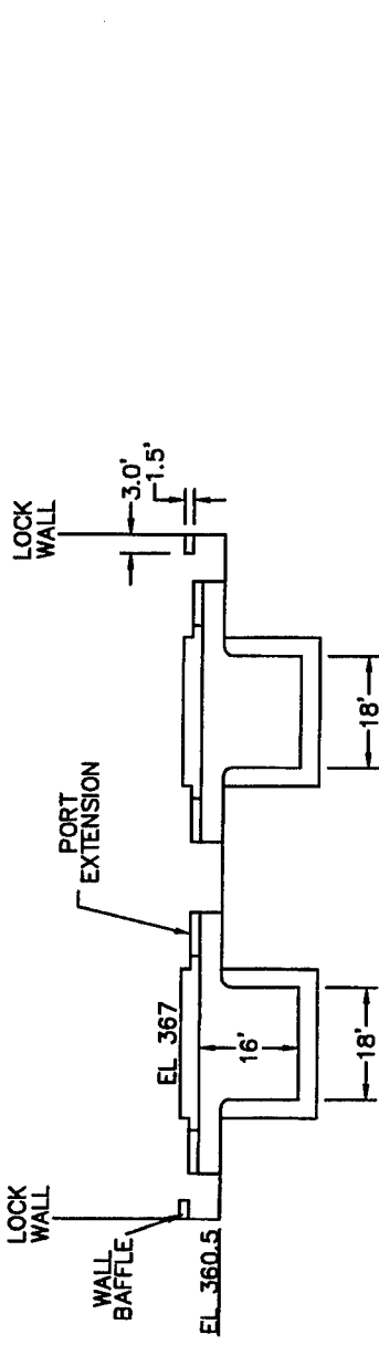
CROSS-SECTIONAL VIEW THROUGH UPSTREAM PORTS
