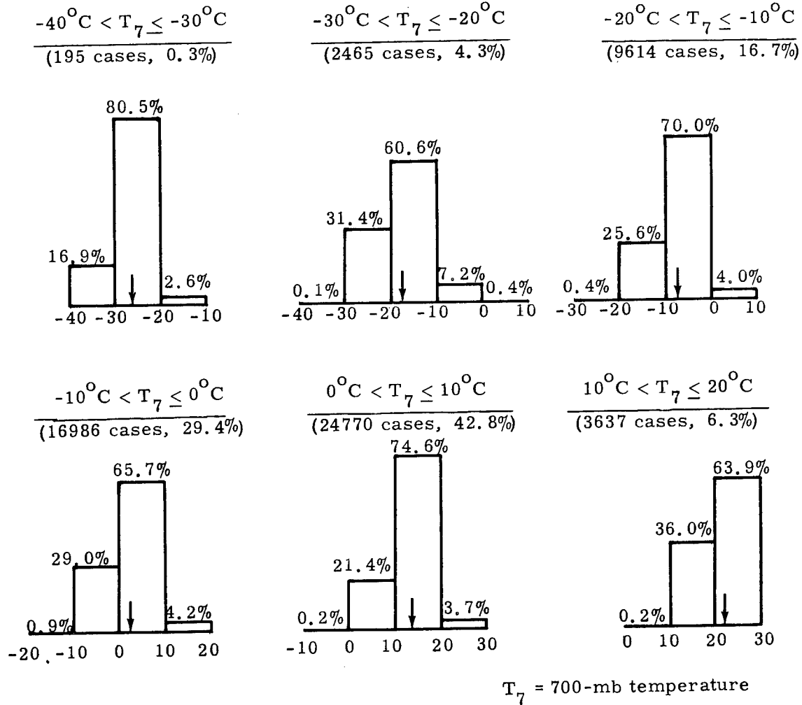
Fig. 5 -- Percent frequency of 850-mb temperatures occurring with specified 700-mb temperatures (arrows indicate group means)
