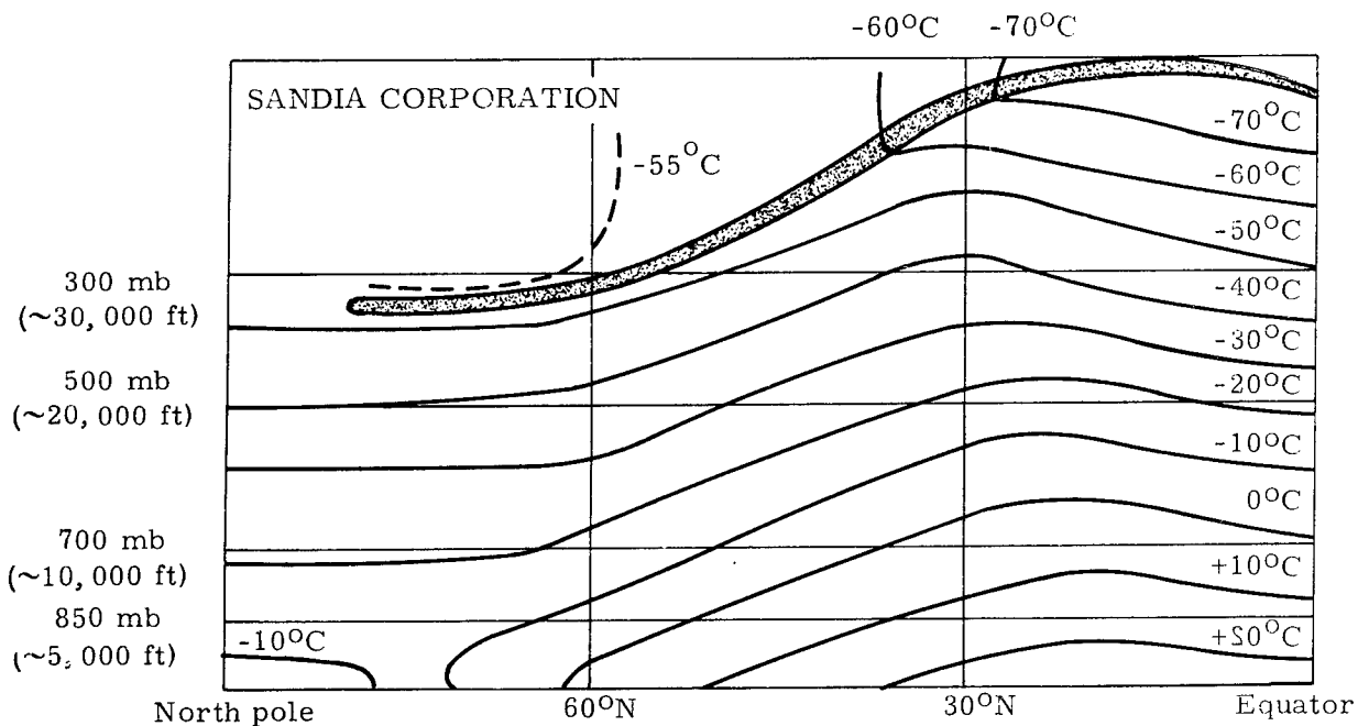
Fig. 1 -- Schematic temperature cross section of Northern Hemisphere (shaded area is the tropopause)
