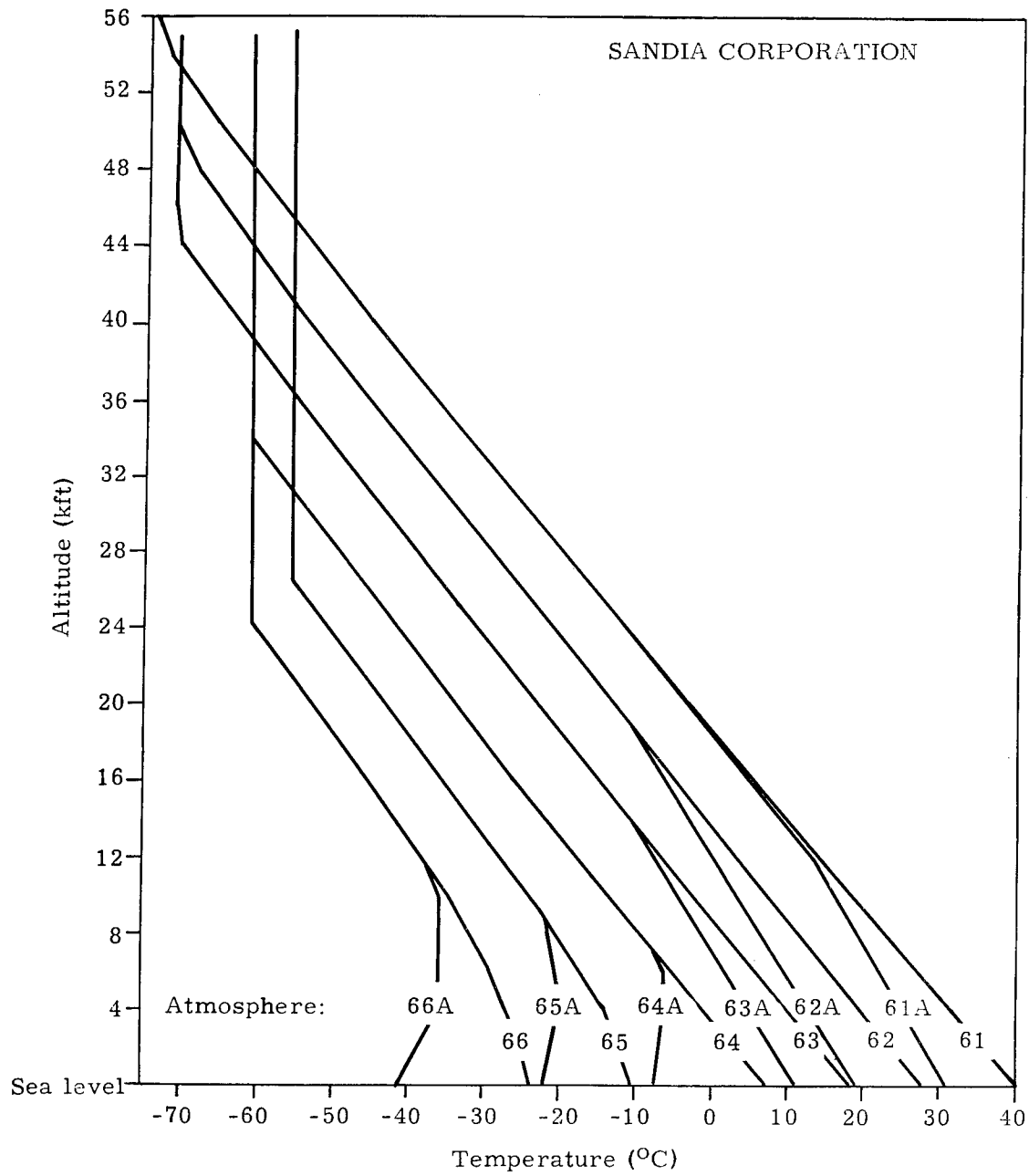
Fig. 3 -- Standard Atmospheres
