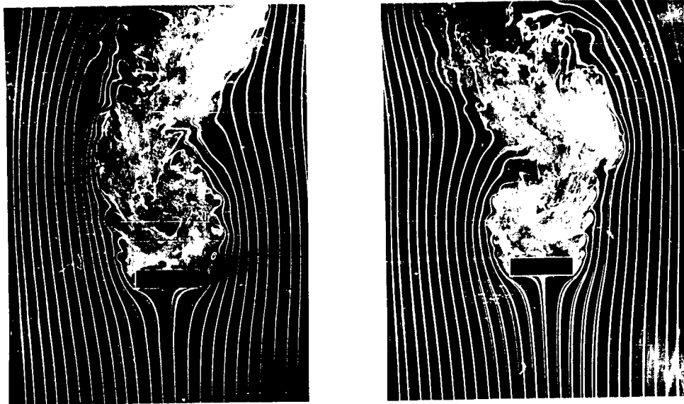
Fig. 29. Experimental streakline patterns for R = 5000 obtained by Lippisch.
