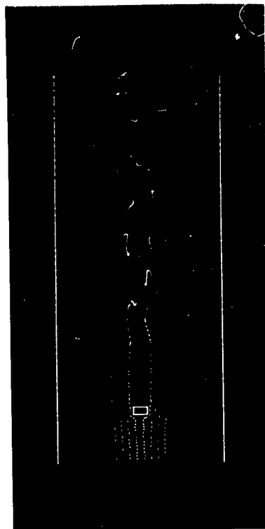
Fig. 12. Qualitative comparison between examples of experimental and calculated streakline patterns. Upper frame obtained by Thom.
