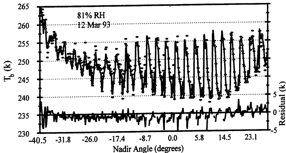
Fig. 5. Angle dependence of data for a cloud-free region of the tropical Pacific ( 7^{\circ}\text{S} to 3^{\circ}\text{N} , 190^{\circ}\text{E} to 203^{\circ}\text{E} , March 12, 1993). The solid line connects SSM/T-2 measurements at 92 GHz and the open circles represent the corresponding adjusted 85-GHz M/I signals. SSM/I measurements.
