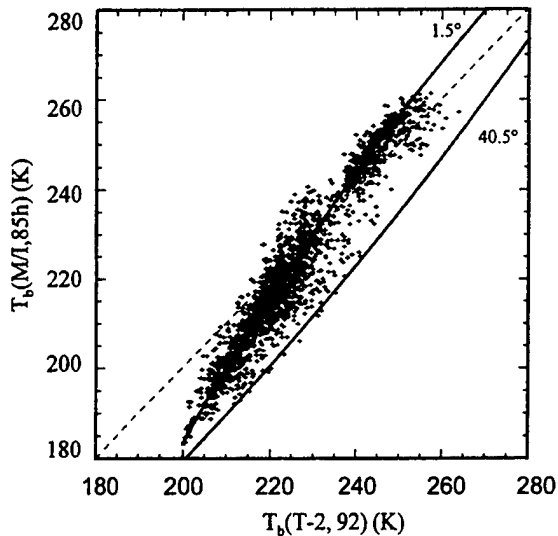
Fig. 6. Scatter plot of raw SSM/I 85( h ) measurements versus the collocated 92-GHz SSM/T-2 measurements, for orbital passes f11-17 211 (45°S to 45°N) spanning the central Pacific Ocean. All SSM/T-2 scan angles are represented. The data were not cloud-cleared and include an extensive frontal system. The upper solid curve, labeled 1.5°, summarizes the results for \phi = 1.5^\circ from model calculations for a variety of atmospheres. Corresponding results for the outer scan position \phi = 40.5^\circ fall along the lower solid line.
