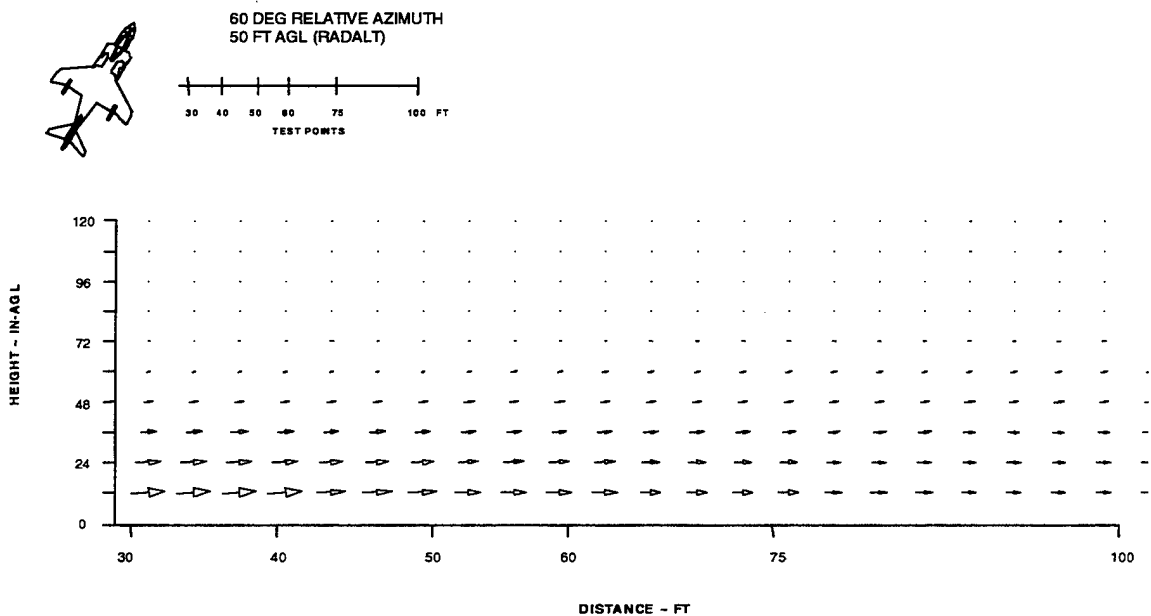
Figure F-6: Flow Field Streamlines during a 50 ft-AGL Hover at the 60 deg Relative Test Azimuth
