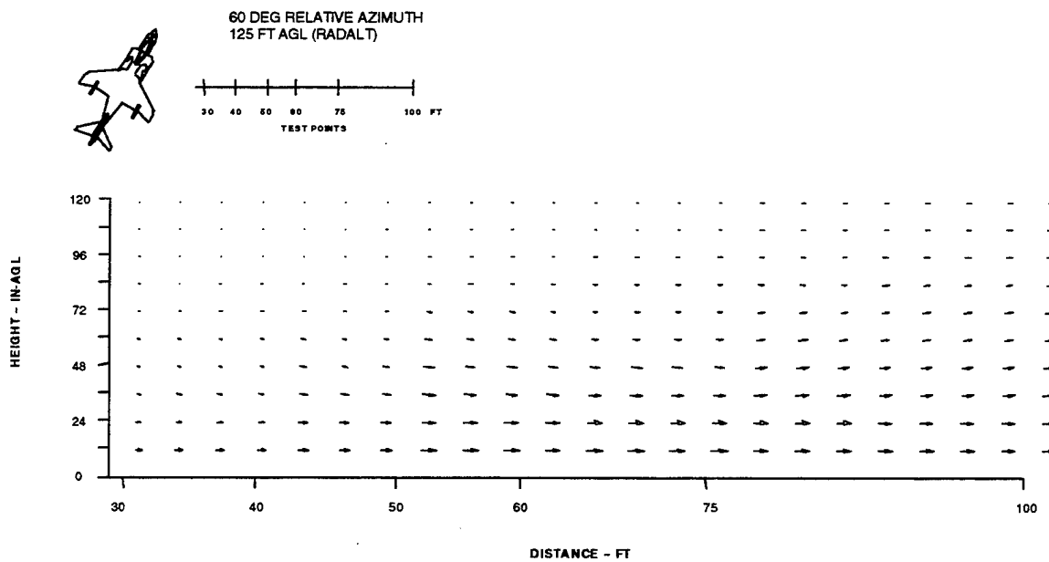
Figure F-18: Flow Field Streamlines during a 125 ft-AGL Hover at the 60 deg Relative Test Azimuth
