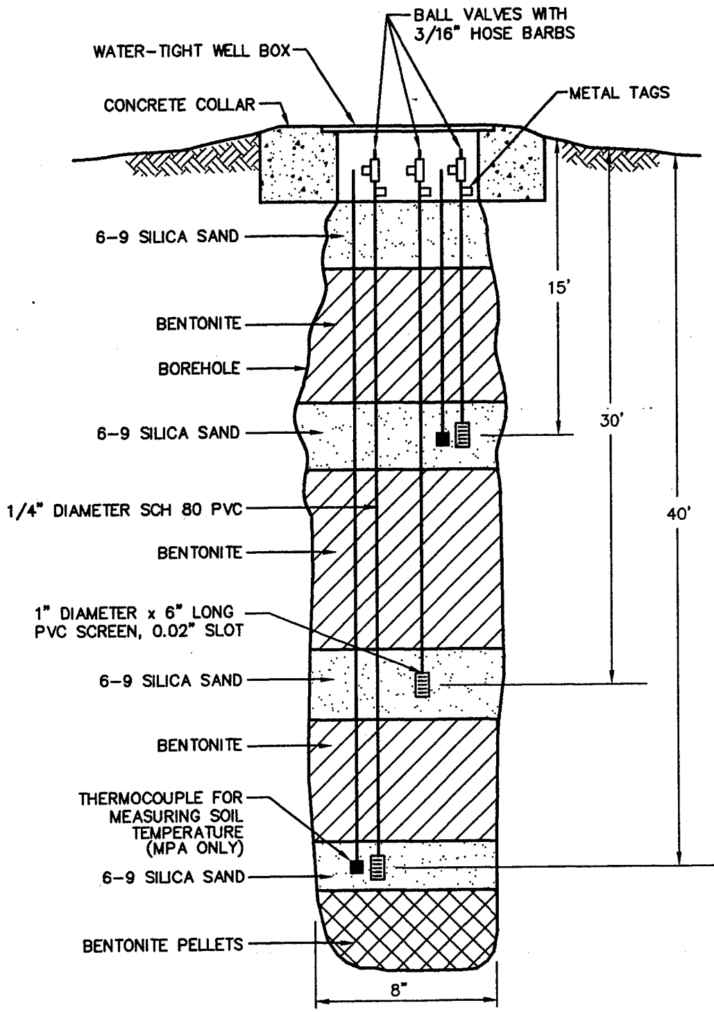
FIGURE 3.3 PROPOSED MONITORING POINT CONSTRUCTION DETAIL SWMU 14 Fort Rucker, Alabama PARSONS ENGINEERING SCIENCE, INC. Denver, Colorado
