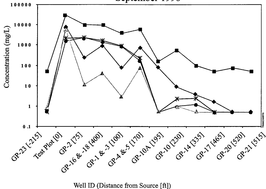
Figure 54. Contaminants Along Transect (a) 1996; (b) 1998
