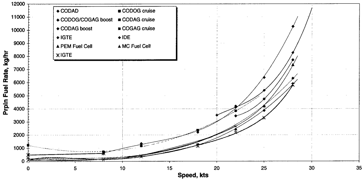
Figure 7. Large plant fuel rates versus speed.
