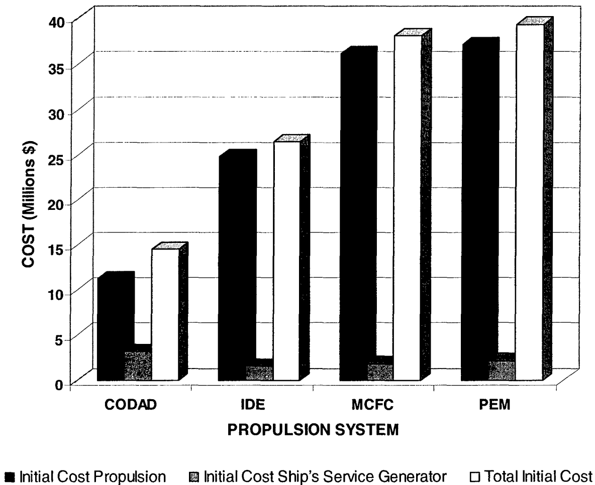
Figure B-1. Propulsion system initial costs.
