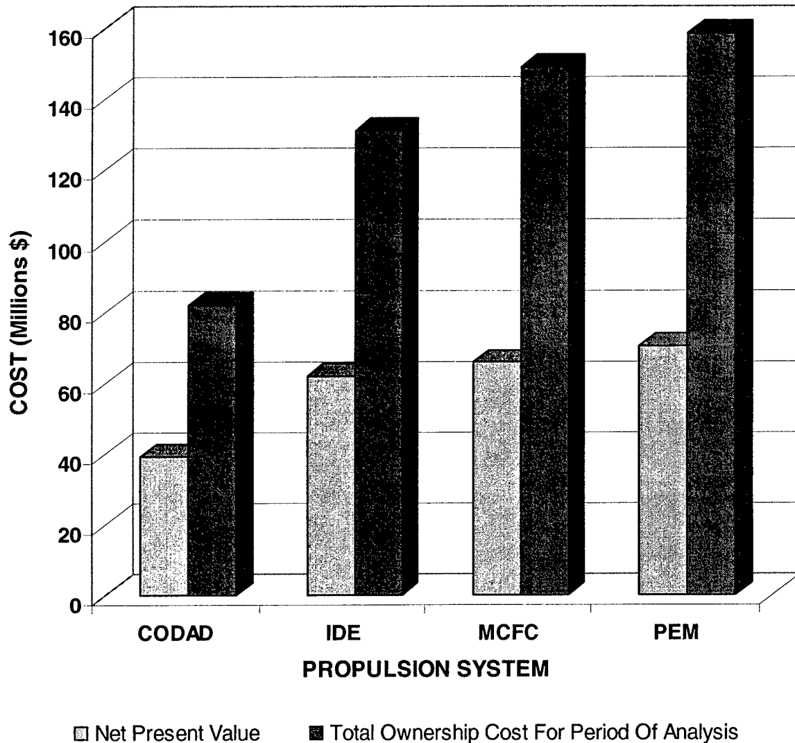
Figure B-3. Propulsion system total ownership costs.
