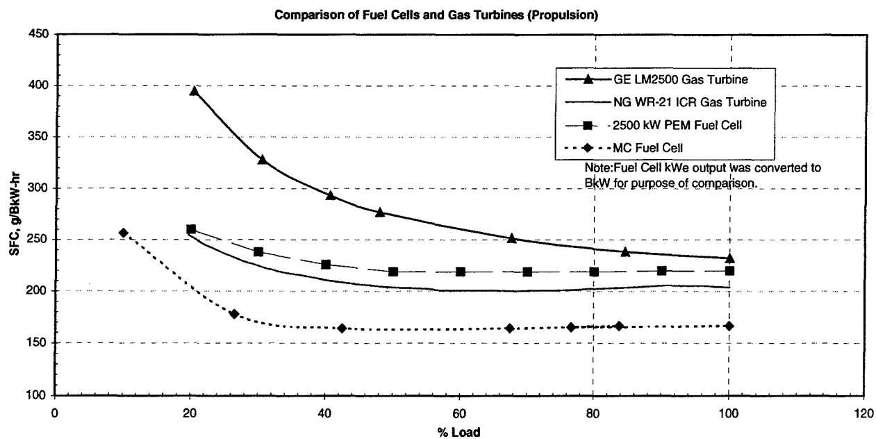
Figure 5. Comparison of fuel cells and gas turbines propulsion specific fuel consumption.
