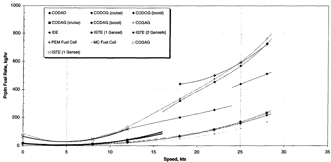
Figure 6. Small plant fuel rates versus speed.
