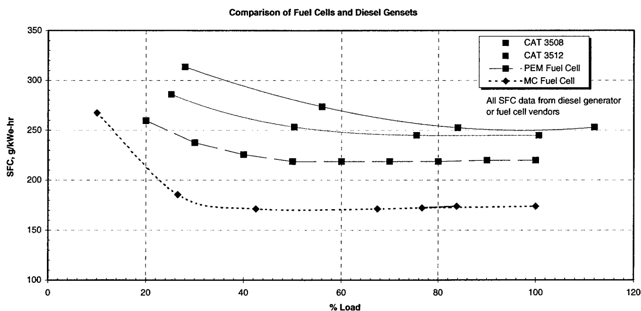
Figure 4. Comparison of fuel cells and diesel gensets specific fuel consumption.
