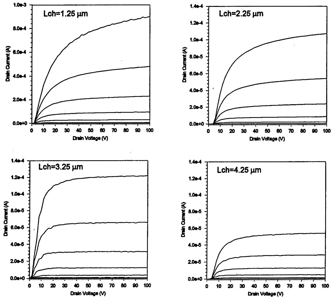
Fig. 1.35 Effect of the channel length ( L_{ch} ) on the output characteristics of an ACCUFET of device structure 2 on a 30 \mu\text{m} thick epilayer with a doping of 2 \times 10^{15} \text{ cm}^{-3} at room temperature (gate voltage varied from 0 to 32 V in steps of 4 V). (LPCVD gate oxide, W_{jch}=3.5 \mu\text{m} )
