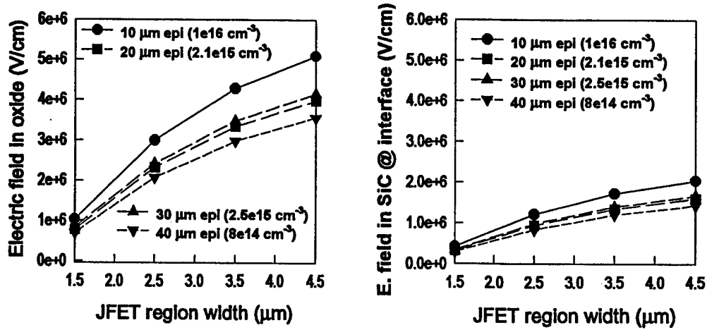
Fig. 1.16 Electric fields in \text{SiO}_2 and in SiC at the \text{SiO}_2/\text{SiC} interface as a function of JFET region width for different epilayers, when the applied drain bias is near breakdown voltage.
