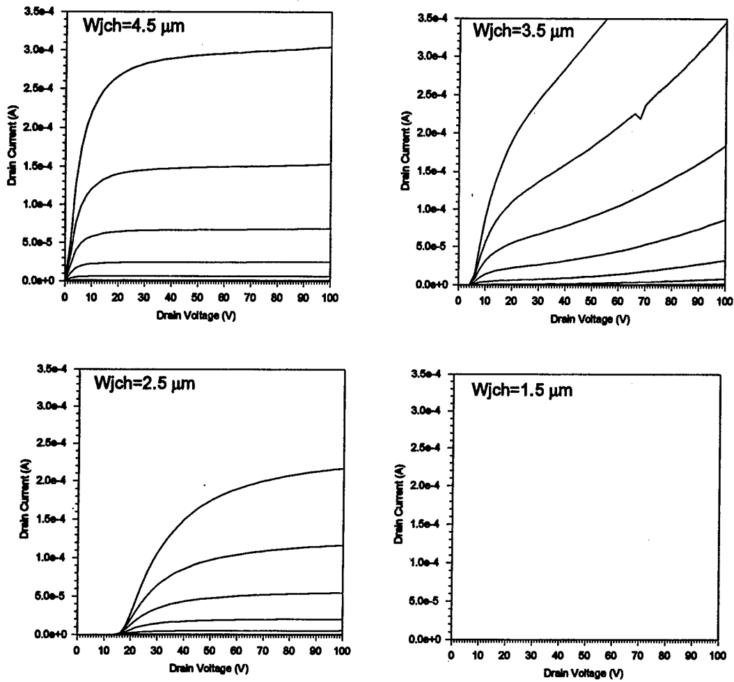
Fig. 1.21 Effect of the width of the buried JFET region ( W_{jch} ) on the output characteristics of an ACCUFET of device structure 3 on a 20 \mu\text{m} thick epilayer with a doping of 1.5 \times 10^{15} \text{ cm}^{-3} at room temperature (gate voltage varied from 0 to 32 V in steps of 4 V). (LPCVD gate oxide, L_{ch} = 2.25 \mu\text{m} )
