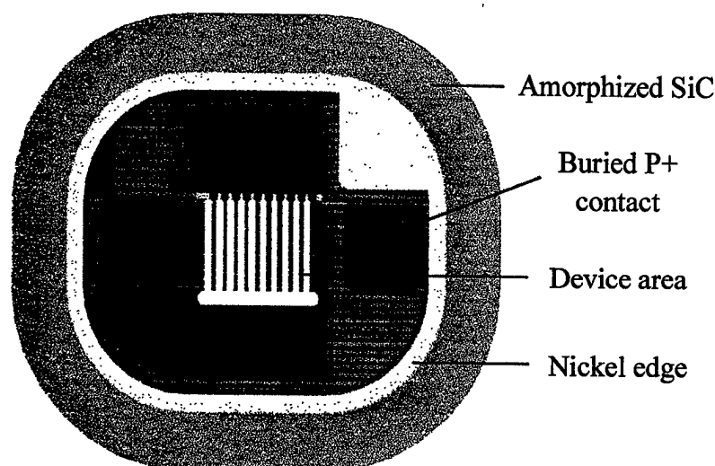
Fig. 1.8 Layout of an ACCUFET exhibiting both the device region and the edge termination.
