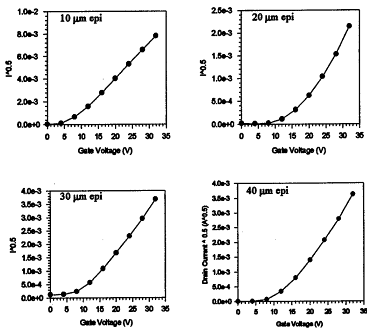
Fig. 1.4 Transfer characteristics of lateral MOSFETs on different epilayers at a temperature of 200 °C (gate voltage varied from 0 to 32 V in steps of 4 V).
