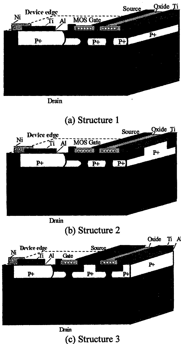
Fig. 1.9 Cross-sections of the three different structures designed for fabrication of ACCUFETs.
