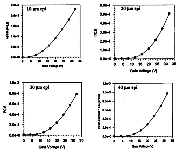
Fig. 1.3 Transfer characteristics of lateral MOSFETs on different epilayers at room temperature (gate voltage varied from 0 to 32 V in steps of 4 V).
