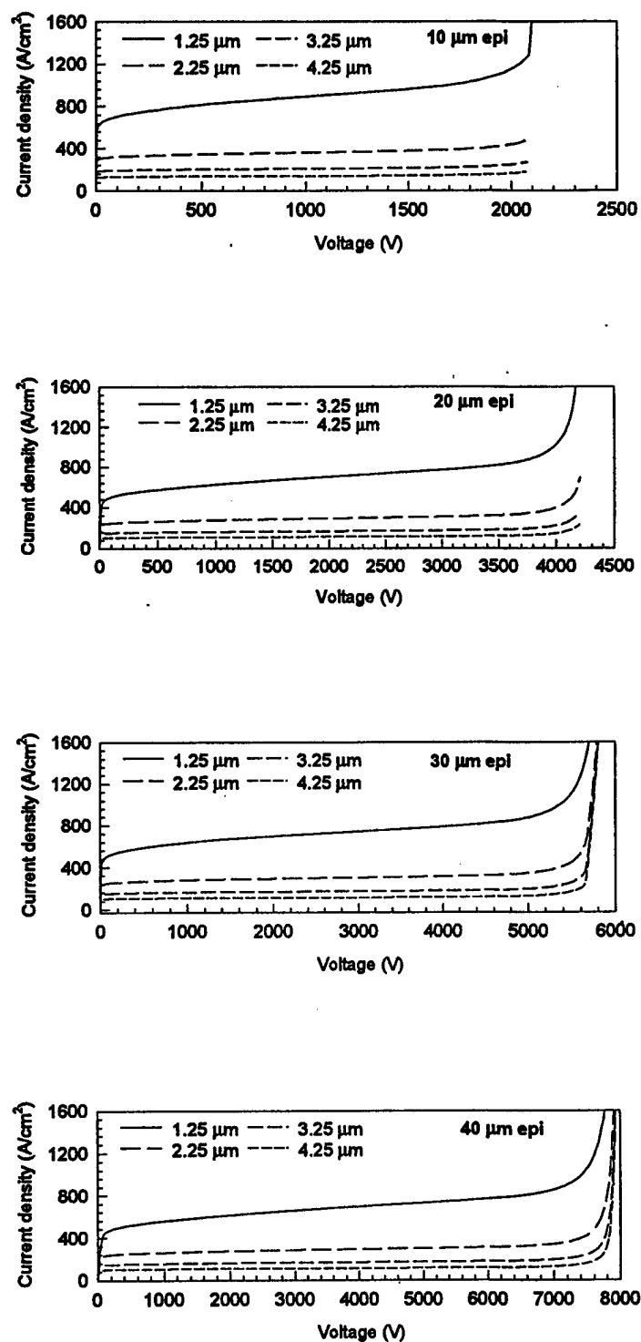
Fig. 1.20 J-V characteristics of the different epilayer materials at a gate bias of 5 V exhibiting breakdown voltage dependence on channel length.
