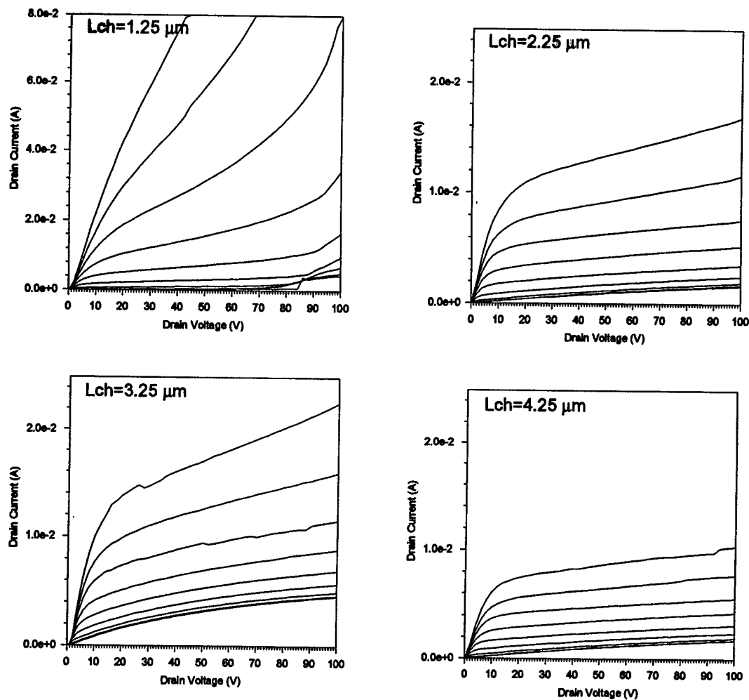
Fig. 1.18 Effect of the channel length ( L_{ch} ) on the output characteristics of an ACCUFET of device structure 3 on a 10 \mu\text{m} thick epilayer with a doping of 1 \times 10^{16} \text{ cm}^{-3} at 200^\circ\text{C} (gate voltage varied from 0 to 32 V in steps of 4 V). (LPCVD gate oxide, W_{jch} = 3.5 \mu\text{m} )
