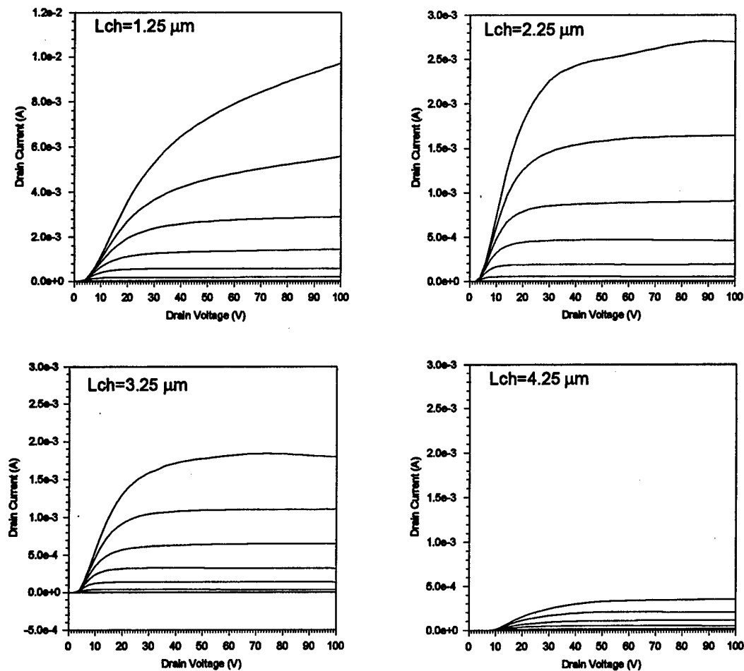
Fig. 1.29 Effect of the channel length ( L_{ch} ) on the output characteristics of an ACCUFET of device structure 2 on a 20 \mu m thick epilayer with a doping of 1.5 \times 10^{15} \text{ cm}^{-3} at 200 ^{\circ}\text{C} (gate voltage varied from 0 to 32 V in steps of 4 V). (LPCVD gate oxide, W_{jch} = 3.5 \mu m )
