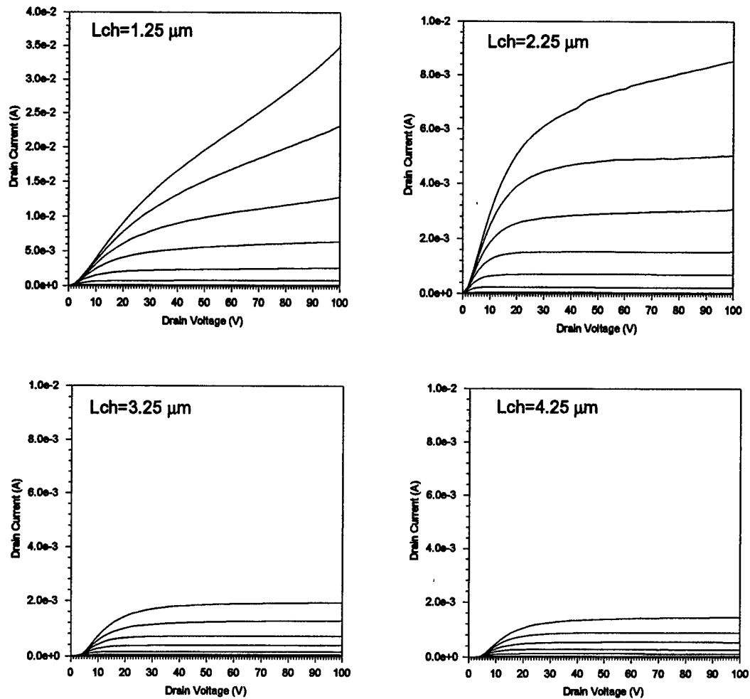
Fig. 1.42 Effect of the channel length ( L_{ch} ) on the output characteristics of an ACCUFET of device structure 3 on a 30 \mu m thick epilayer with a doping of 2 \times 10^{15} \text{ cm}^{-3} at 200 ^{\circ}\text{C} (gate voltage varied from 0 to 32 V in steps of 4 V). (LPCVD gate oxide, W_{jch} = 3.5 \mu m )
