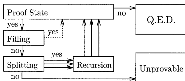
Figure 8.1: Proof strategy
