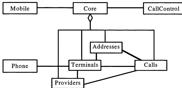
Figure 10: Class diagram representing the domain view of Telephony
