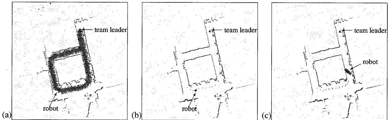
Figure 13: A second robot localizes itself in the map of the first, then contributes to building a single unified map. In (a), the initial uncertainty of the relative pose is expressed by a uniform sample in the existing map. The robot on the left found its pose in (b), and then maintains a sense of location in (c).
