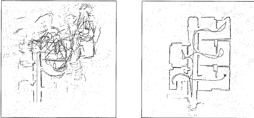
Figure 9: Autonomous exploration and mapping using the urban robot: Raw data and final map, generated in real-time during exploration.
