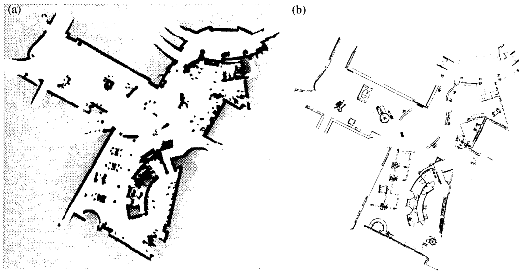
Figure 10: (a) Occupancy grid map and (b) architectural blueprint of a recently constructed museum in San Jose. Notice that the blueprint is inaccurate in certain places.
