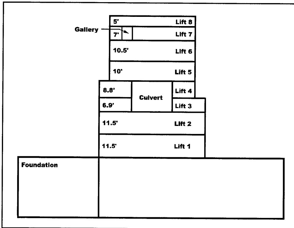
Figure 16. Lock wall section used in example
