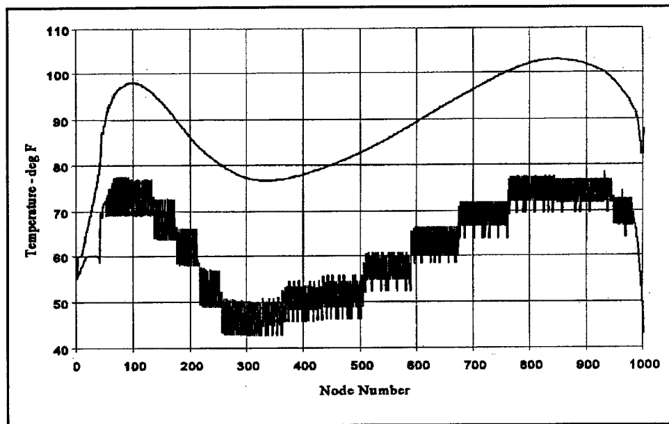
Figure 10. Mass gradient peak temperatures for 1 July start
