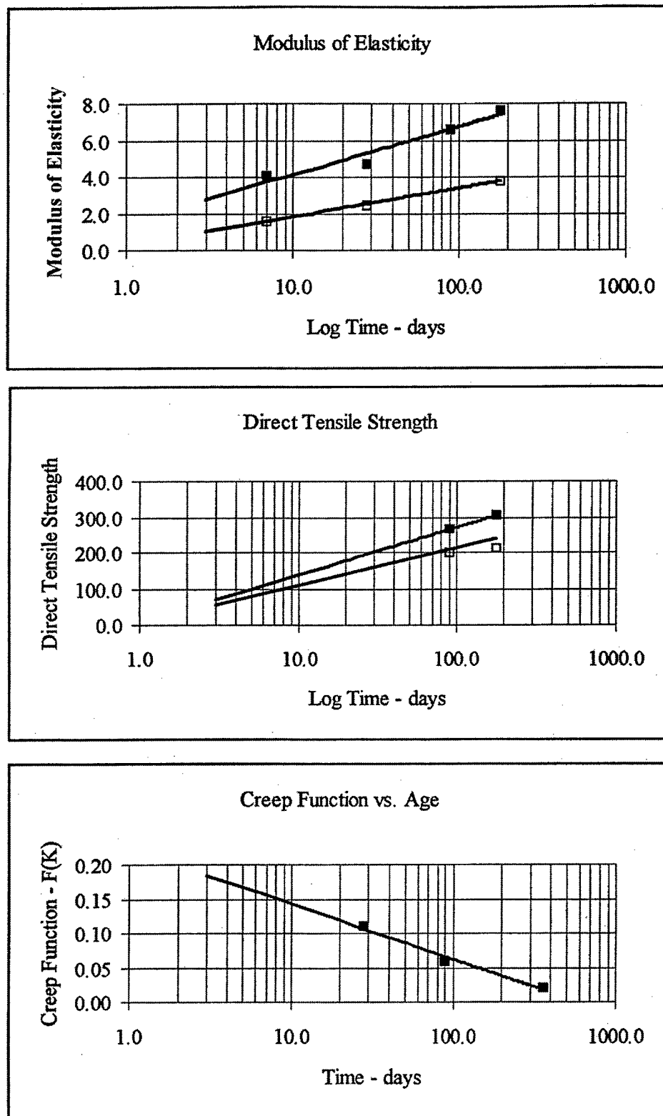
Figure 3. Estimated elastic and creep properties
