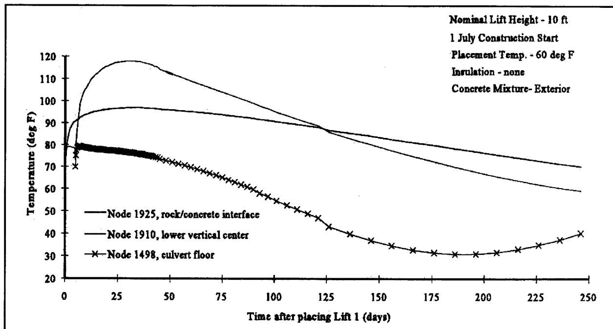
Figure 20. Typical temperature histories at locations of mass gradient analysis
