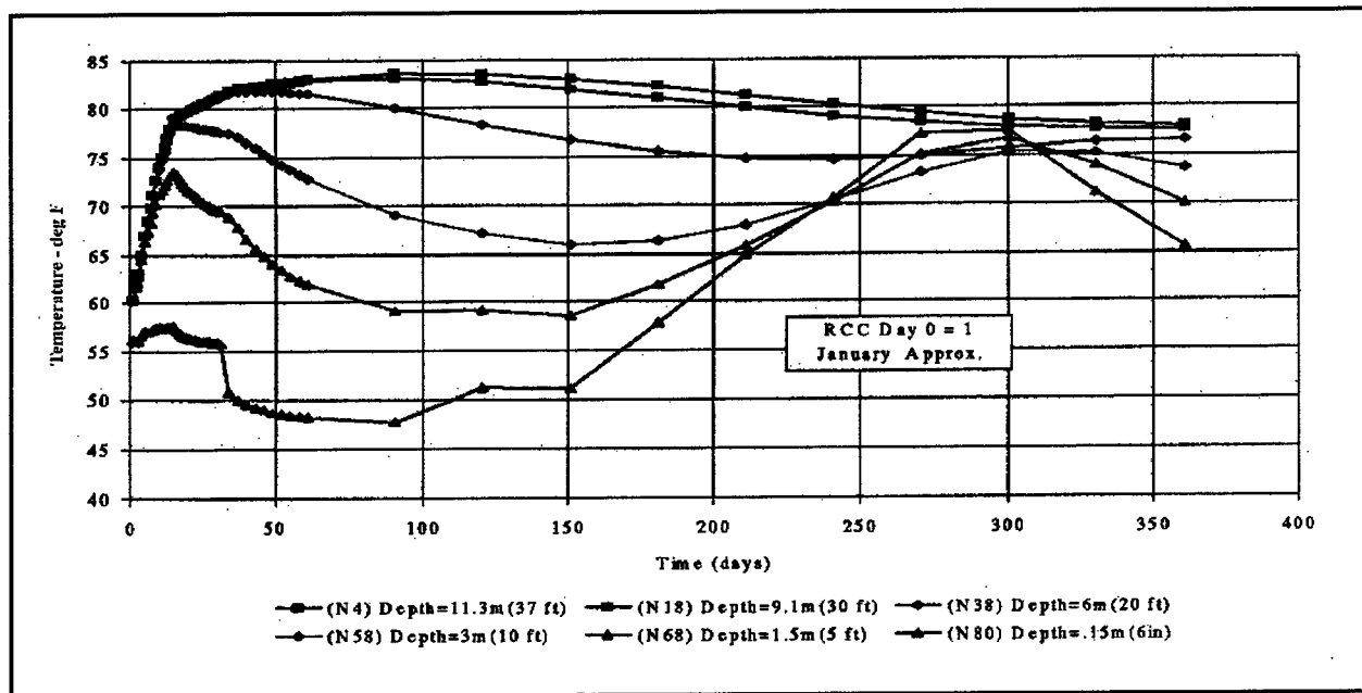
Figure 13. Temperature history for selected nodes from surface gradient model
