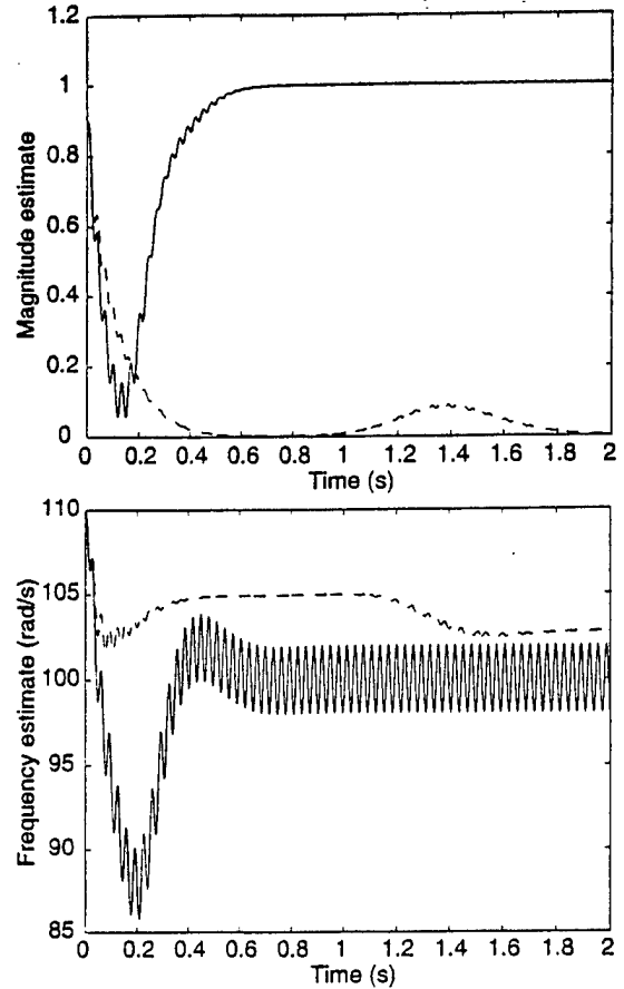
Fig. 5. Estimates \theta_1 and \theta_2 of the original and improved algorithms.
