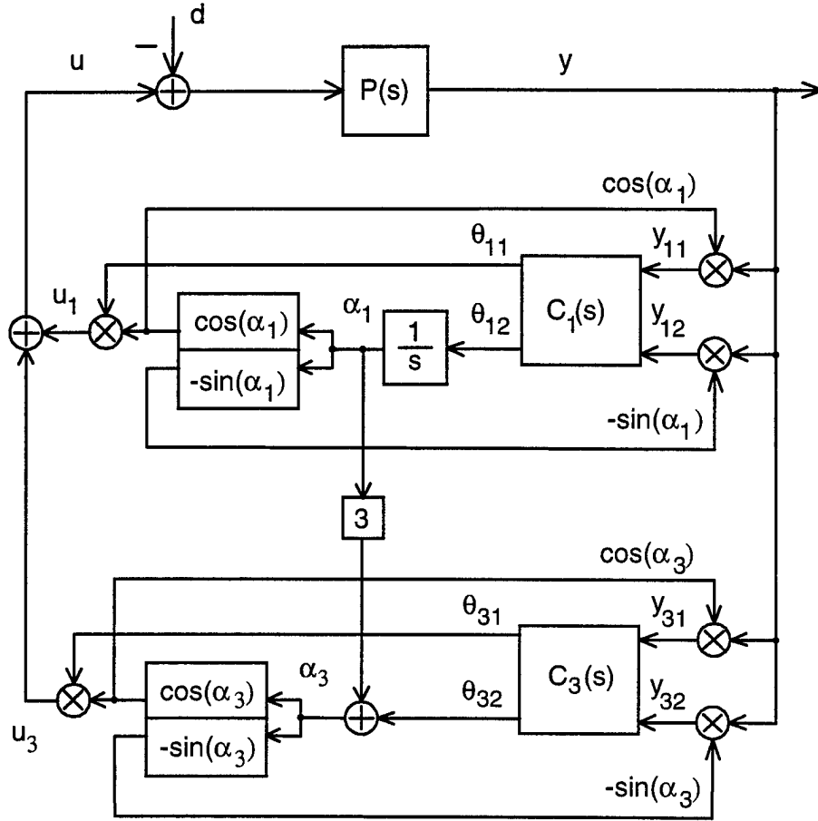
Figure 3: Direct algorithm for periodic disturbance cancellation
