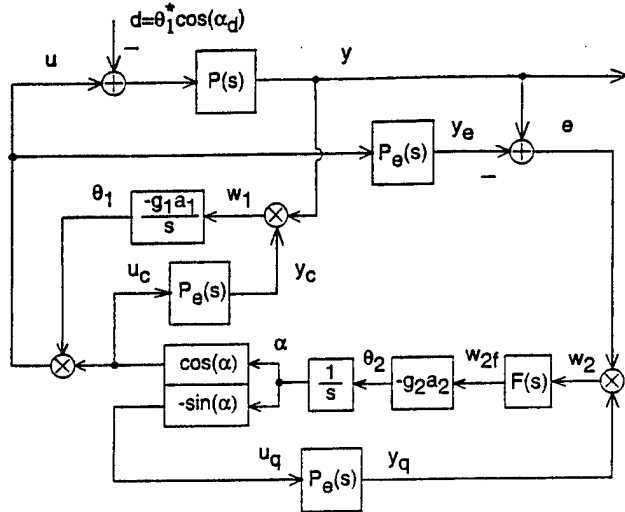
Fig. 4. Improved implementation of Chaplin and Smith's method.
