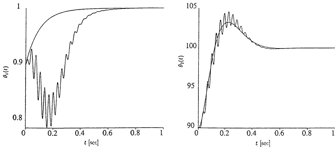
Figure 5: Adaptive parameters - Noiseless case
