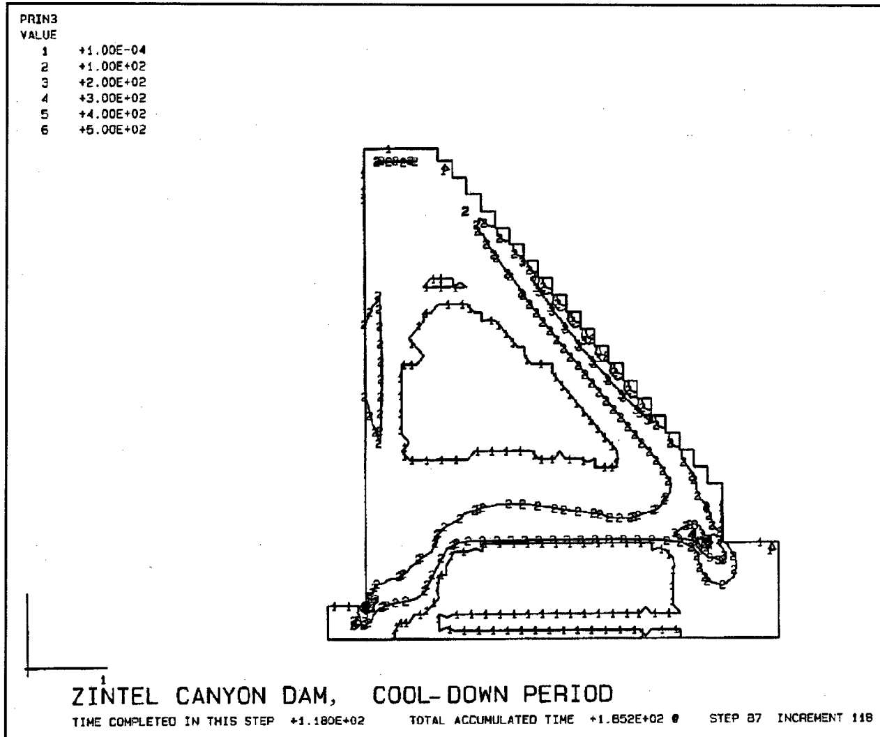
Figure 16. Principal stress contours, transverse model, Zintel Canyon Dam, cool-down period
