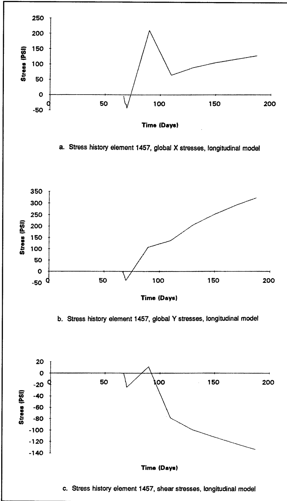
Figure 38. Stress histories for elements, longitudinal model, element 1457
