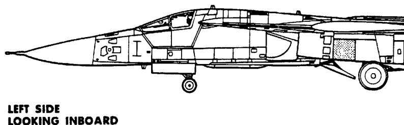
Figure 15: Location of panel 3208 (12B3913) on the F-111 aircraft (identified by shaded area) [2].
