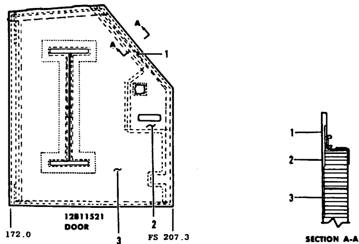
Figure 18. Panel 1102 structural detail. [2]
