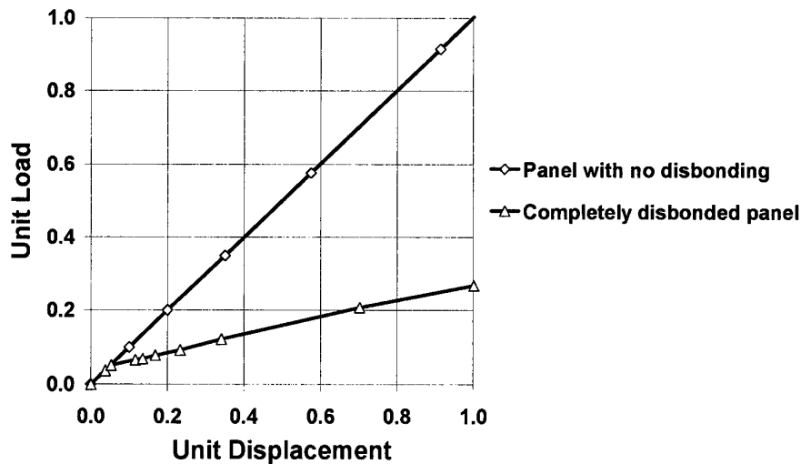
Figure 14: Load-displacement response of an intact panel and a completely disbonded panel.
