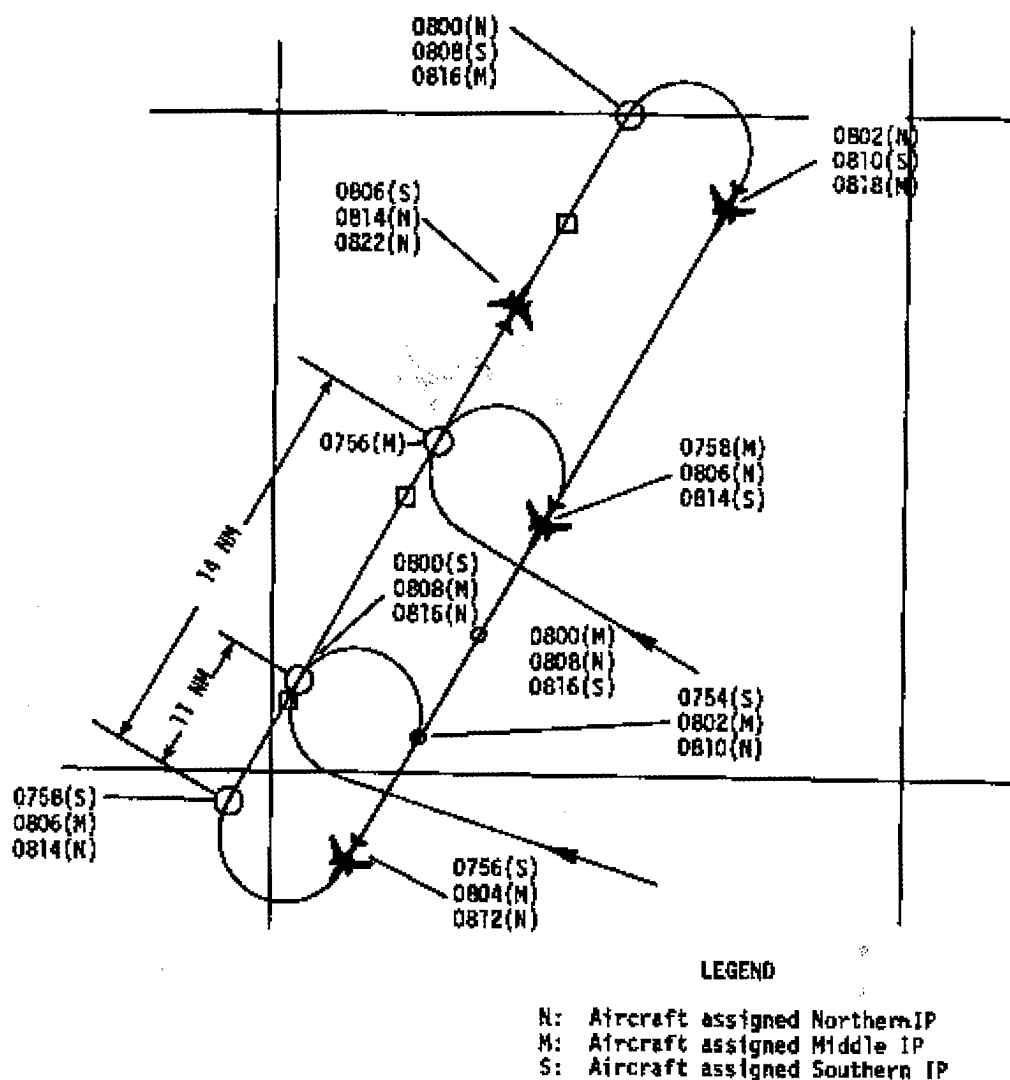
Figure 12. This sketch shows how three EB-66s would be positioned with a scheduled "in place" time of 0800. This "super" orbit was successfully used throughout the Vietnam War. Four aircraft are depicted to show proper positioning.
