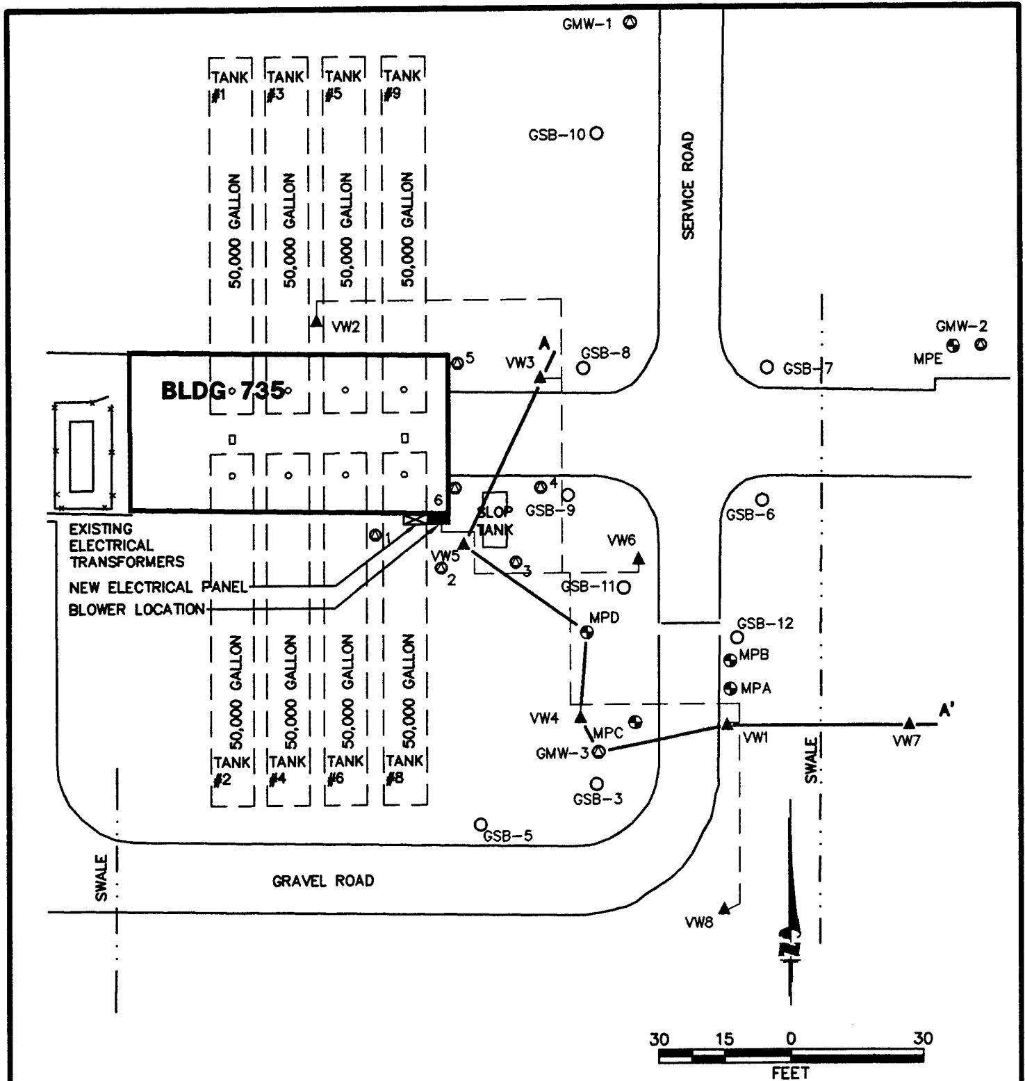
FIGURE 2.1 AS-BUILT SITE LAYOUT Building 735 Grissom Air Force Base Indiana PARSONS ENGINEERING SCIENCE, INC. Denver, Colorado
