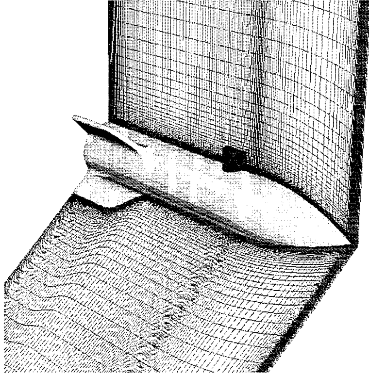
Figure 1. Computational Mesh.
