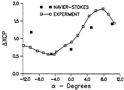
Figure 12. Center of Pressure Versus Angle of Attack, Mach 2, P_{oj} = 27 atm, Body Alone.
