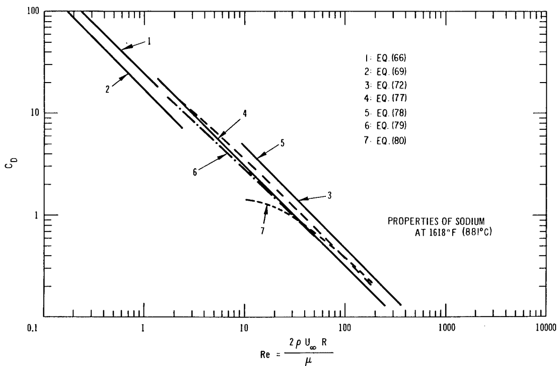
Fig. 13. Drag Coefficient for a Sodium-vapor Bubble
