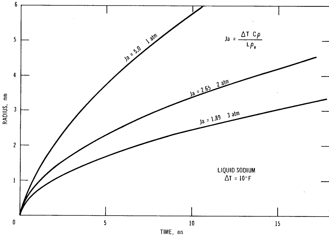
Fig. 9. Effect of Pressure on Growth of a Sodium-vapor Bubble. Conversion factors: 1 atm = 0.1 MPa; °C = (°F - 32)/1.8.
