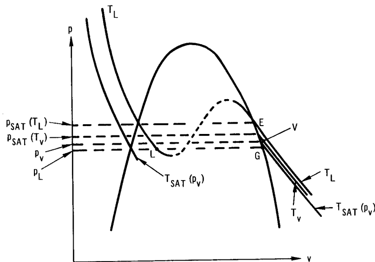
Fig. 3. Equilibrium States of Liquid and Vapor with a Curved Interface
