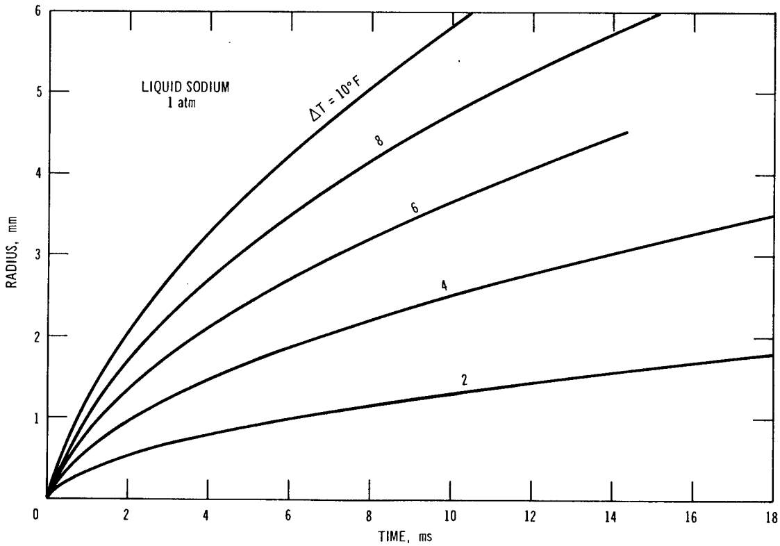
Fig. 10. Effect of Superheat on Growth of a Sodium-vapor Bubble. Conversion factors: 1 atm = 0.1 MPa; °C = (°F - 32)/1.8.
