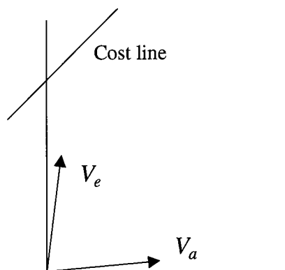
Figure 5. Probability Vectors
