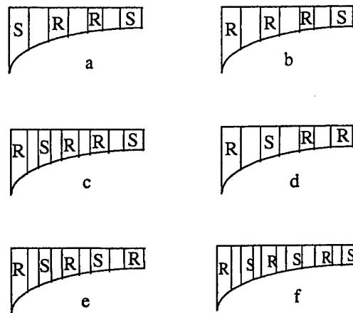
Illustration of different configurations R = rotor blade S = stator blade
