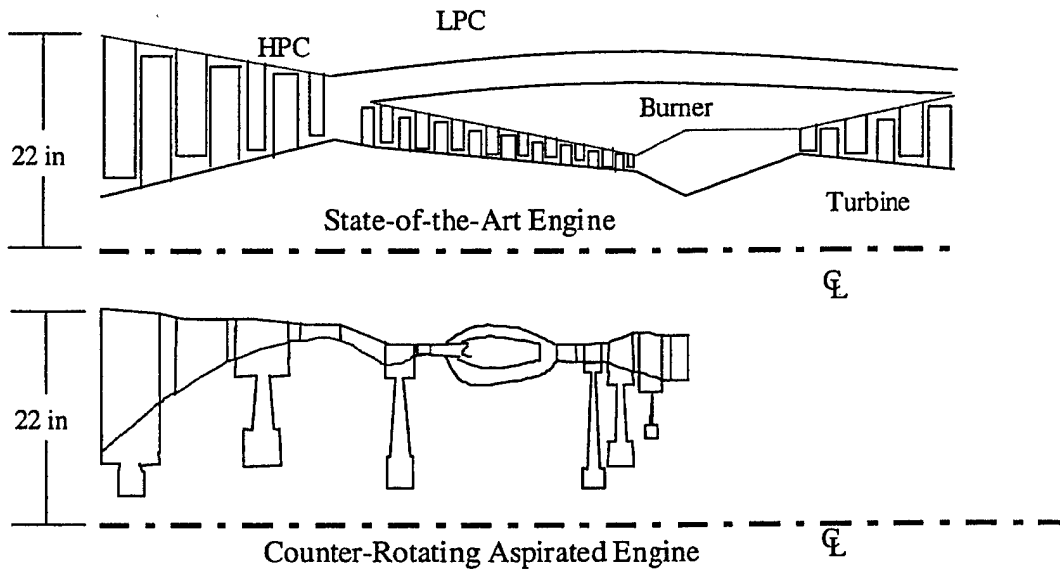
Figure 3.3: Comparison of counter-rotating aspirated engine to a modern engine
