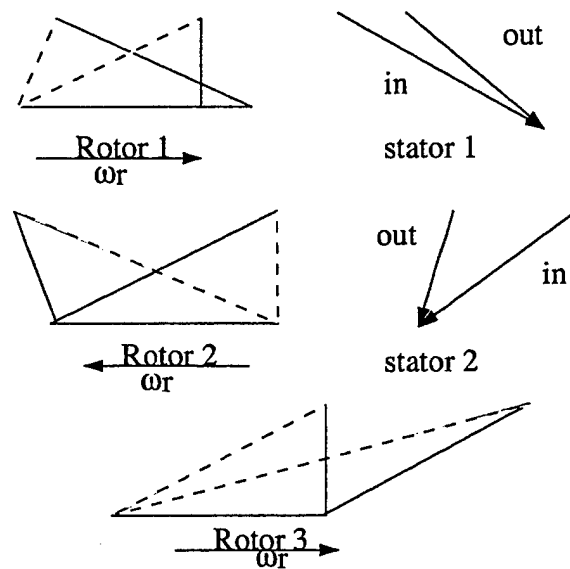
Composite velocity triangles at mean streamline
