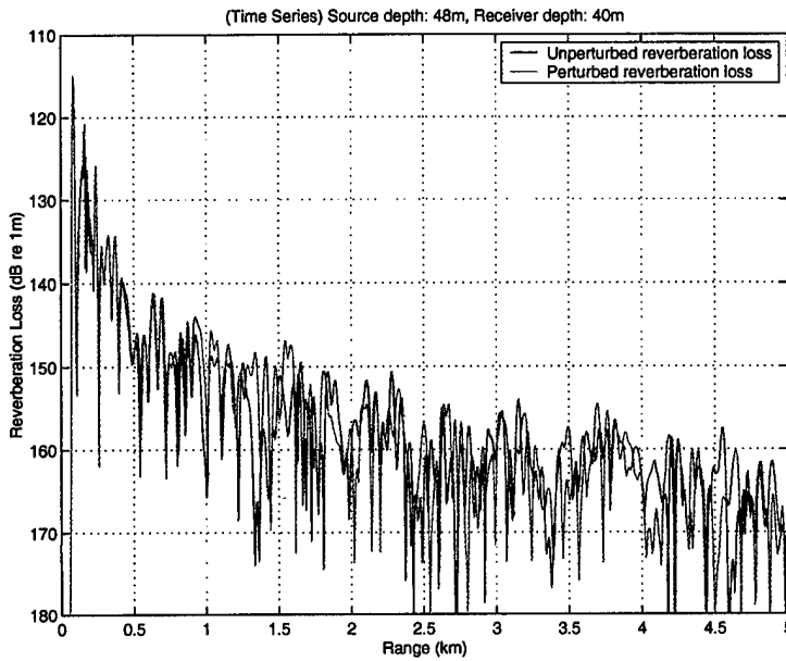
Figure 4.26 – Interface Reverberation Loss (dB re 1 m) vs Range Using Time Series Data
