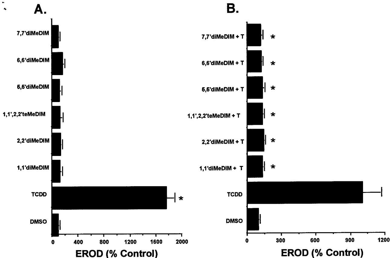
Fig. 3. EROD induction (A) and inhibition of TCDD-induced EROD activity (B) by alkyl-substituted DIMs in T47D cells. Cells were treated with DMSO vehicle, 1 nM TCDD, 100 \mu M alkyl-substituted DIMs (50 and 10 mM not shown) or cotreated with 1 nM TCDD plus 10 \mu M alkyl-substituted DIMs and EROD activities were determined fluorimetrically. Results are the average of 3 replicate experiments expressed percent control \pm standard error. (A) * Significant induction ( P < 0.05 ) of EROD activity compared to control experiment. (B) * Significant inhibition ( P < 0.05 ) of TCDD-induced EROD activity.
