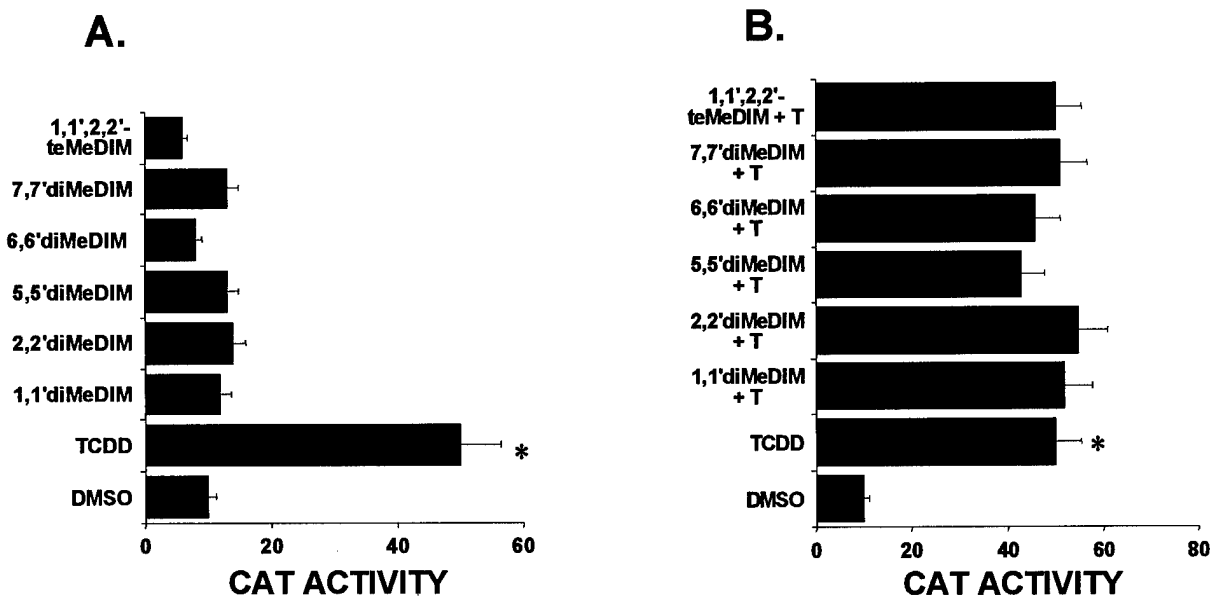
Fig. 4. AhR agonist (A) and antagonist (B) activities of alkyl-substituted DIMs in T47D cells transfected with pRNH11c. Cells were treated with DMSO (control), TCDD (T) (1 nM) and compounds (10 \mu M) alone or in combination with TCDD and CAT activities were determined. Results are expressed as means \pm S.E. for three separate experiments for each treatment group. * Significant induction ( P < 0.05 ) of CAT activity.
