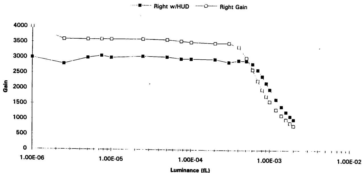
Figure 3 GAIN COMPARISON WITH AND WITHOUT HUD
