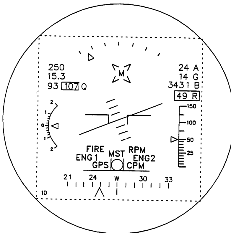
Figure 1 HH-60H MASTER MODE SYMBOLGY
