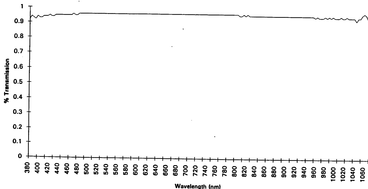
Figure 2 HUD TRANSMISSIVITY
