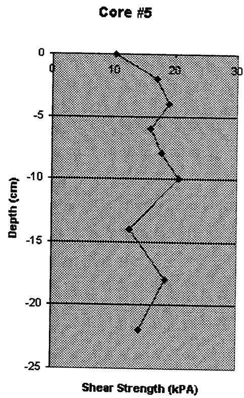
Figure 14. Shear Strength Vs. Depth for Cores 1-3, and 5.
