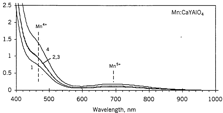
Fig. 1. Absorption in manganese doped \text{CaYAlO}_4 . 1 - Mn=0.1%, 2 - Mn=0.5%, 3 - Mn=0.5%, Ce=0.5%, 4 - Mn=2%.
