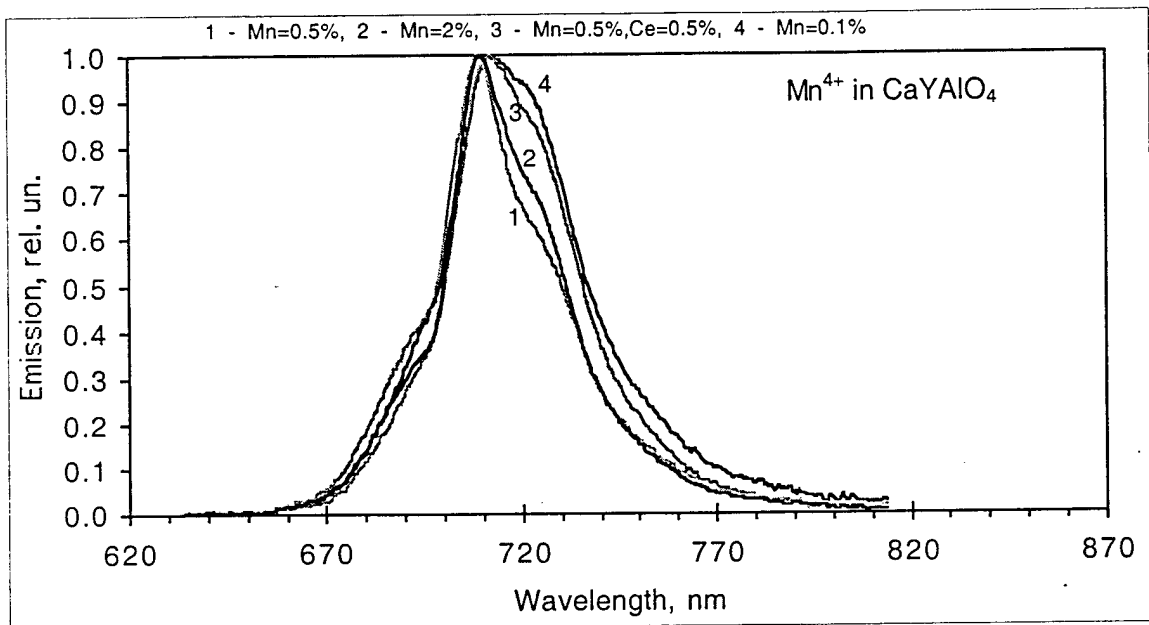
Fig. 2. Emission spectra in manganese doped CaYAlO_4 . 1 - Mn=0.5%, 2 - Mn=2%, 3 - Mn=0.5%, Ce=0.5%, 4 - Mn=0.1%.
