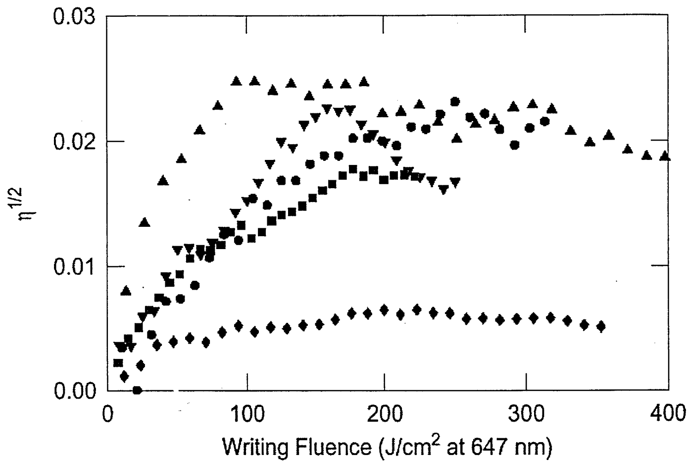
Figure 7. Dependence of diffraction efficiency on red light fluence (647 nm) at different red light intensities and intermediate green light intensity (514.5 nm, 0.7 W/cm 2 ). 647 nm: ▲ - 0.65 W/cm 2 , ◆ - 0.78 W/cm 2 , ■ - 0.9 W/cm 2 , ▼ - 1 W/cm 2 , and ● - 1.3 W/cm 2 .
