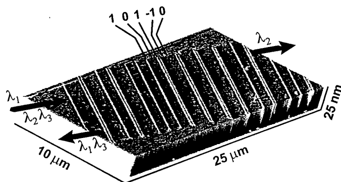
Fig. 6. A non-periodic silicon dioxide grating that has been direct written on a silicon surface using an atomic force microscope. The structure (which also was profiled by an AFM) is annotated with wavelengths and stripe reflectances in the same manner as the proposed filter of Fig. 1(c). The closest spacing of adjacent lines in this AFM profile is 240 nm for a 1 followed by a -1.
