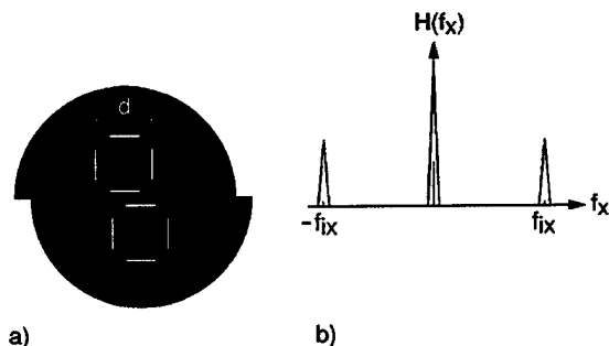
Figure 2. (a) Schematic of the two four-slot pupil arrangements covering the split-lens device and (b) its corresponding monochromatic optical transfer function along the x direction; b shows 2x magnified view.
