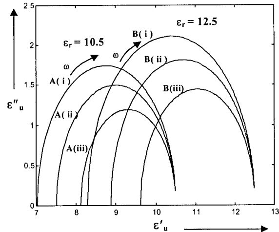
Fig. 3 Cole-Cole diagram for the test microstrip structures curves A: alumina ( \varepsilon_r = 10.5 ) curves B: gallium arsenide ( \varepsilon_r = 12.5 ) (i) (w/\lambda)/(h/\lambda) = 1.0 (ii) (w/\lambda)/(h/\lambda) = 2.0 (iii) (w/\lambda)/(h/\lambda) = 4.0
