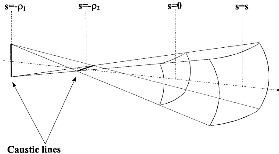
Figure 1. Astigmatic wavefront.
