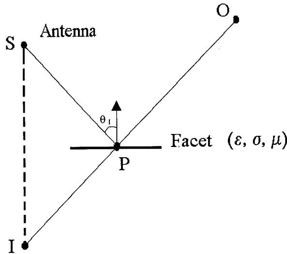
Figure 2. Transmitter antenna in front of a flat facet and definition of the image point, the reflection point and the incident angle.
