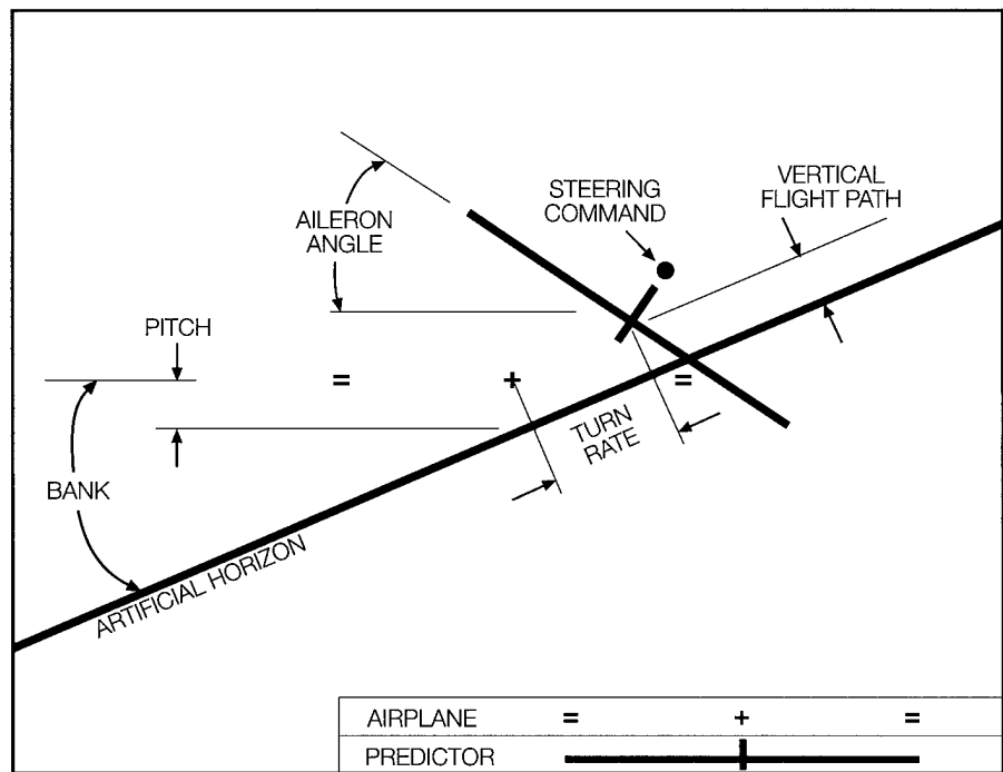
Figure 1. Conventional moving-horizon attitude display with the addition of a flight path predictor and an angles-to-turn-through command symbol for localizer/glideslope and enroute guidance. Illustration by Allison L. Herron.
