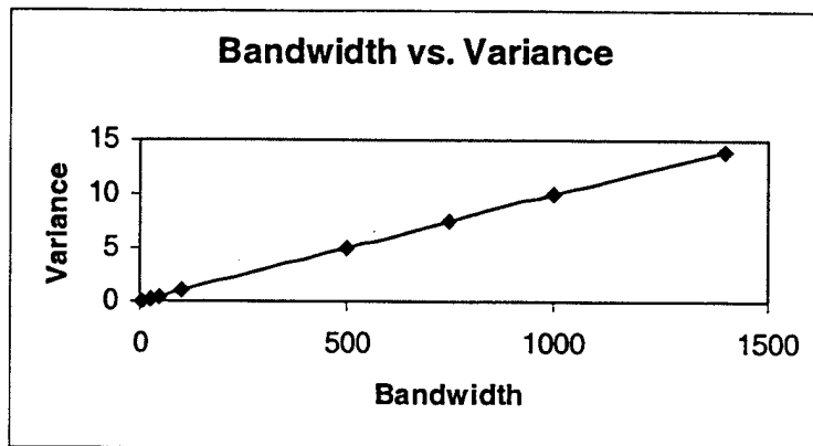
Figure 4. Direct linear relationship between bandwidth and variance.
