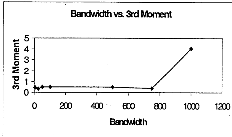
Figure 6. The effect of bandwidth on the skewness (3 rd moment) of the distribution of the first minimum estimates.
