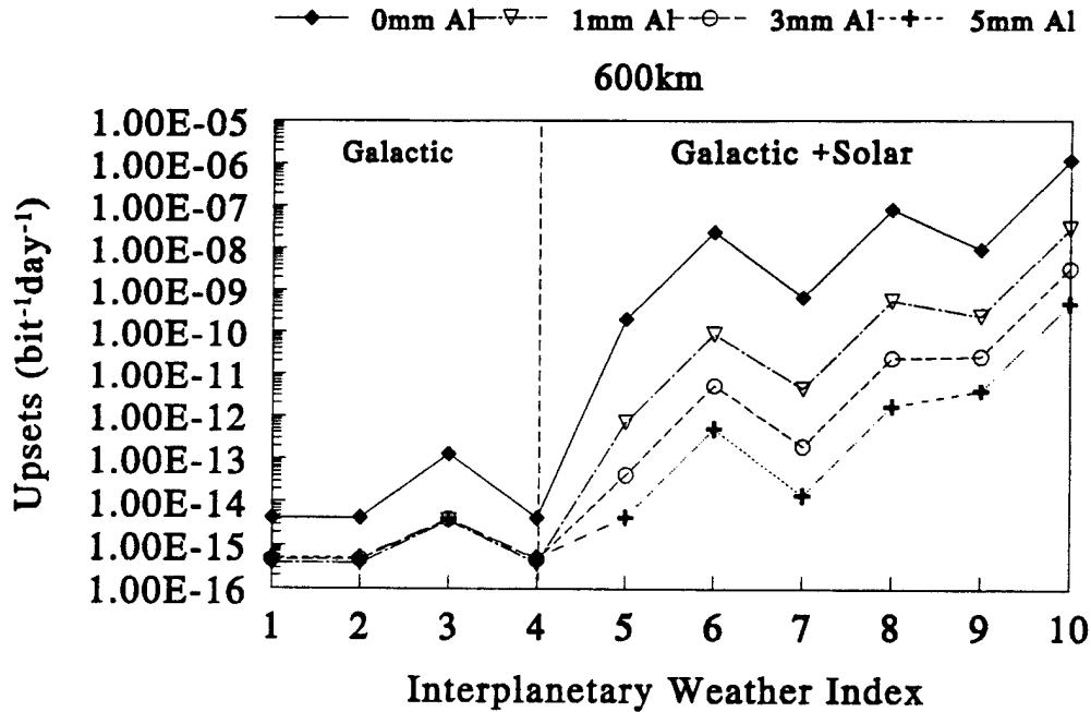
Figure 17. Shielding and solar activity effect on device upset rates at the 600km altitude.
